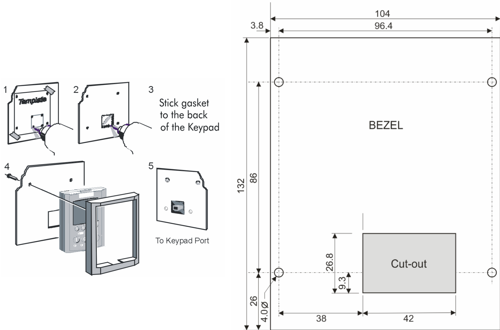
Mounting Dimensions for the Remote-Mounted 6911 Keypad
