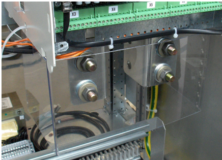
Examples for DC main terminal covers for H3 (left) and H4 (right) converter modules.
