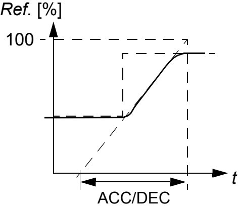
ACC/DEC-tid
