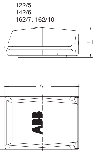
Side-mounted terminal box:
