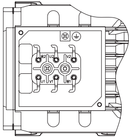
Terminal box size 56-80.
