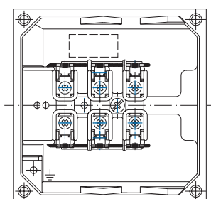
Terminal box size 90-100.
