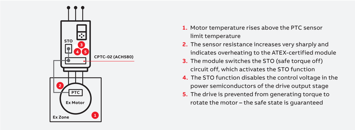
CPTC-02 ATEX certified thermistor protection module, EX II (2) GD
