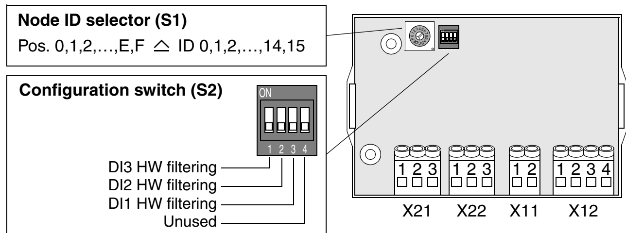
Figure 3-2 Top view of the module, cover removed
