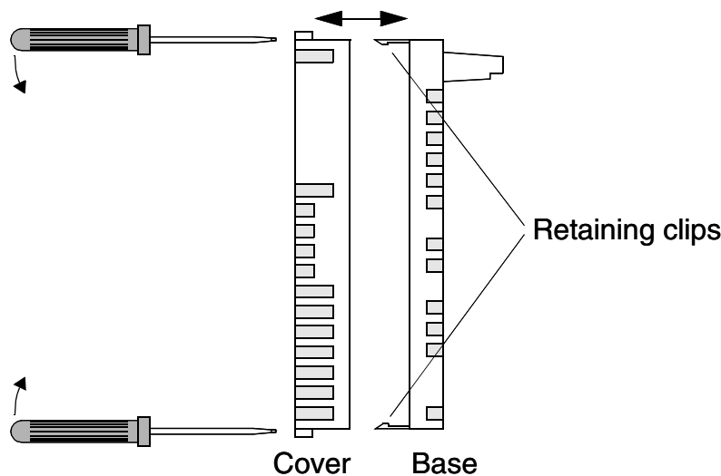
Figure 3-1 Removing and refitting the cover
