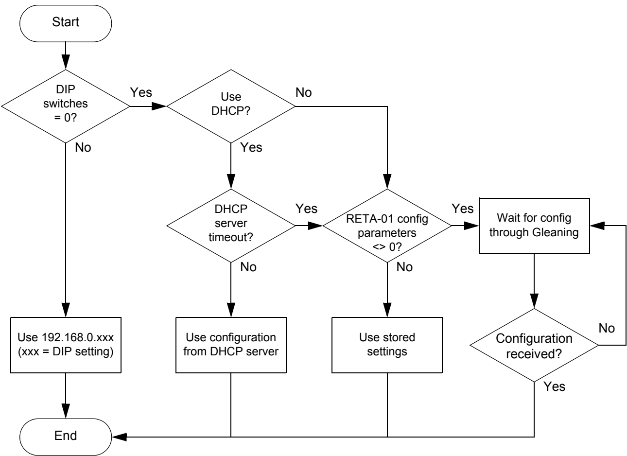
Figure 6. Settings flowchart
