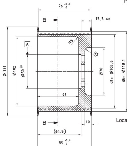
View A
