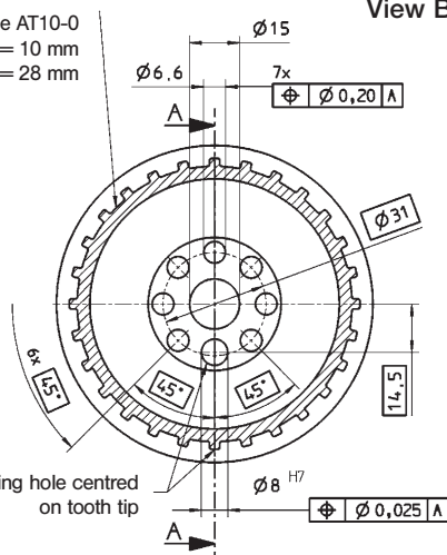
View B
