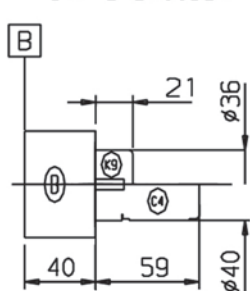
BRAKE+ENCODER
