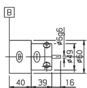
BRAKE+TACHO
