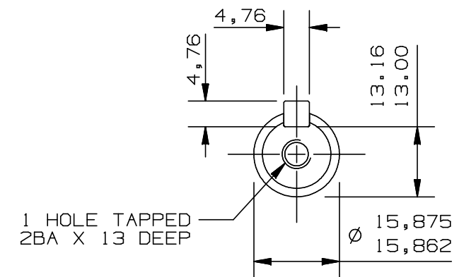
DRIVE END SHAFT DETAILS
