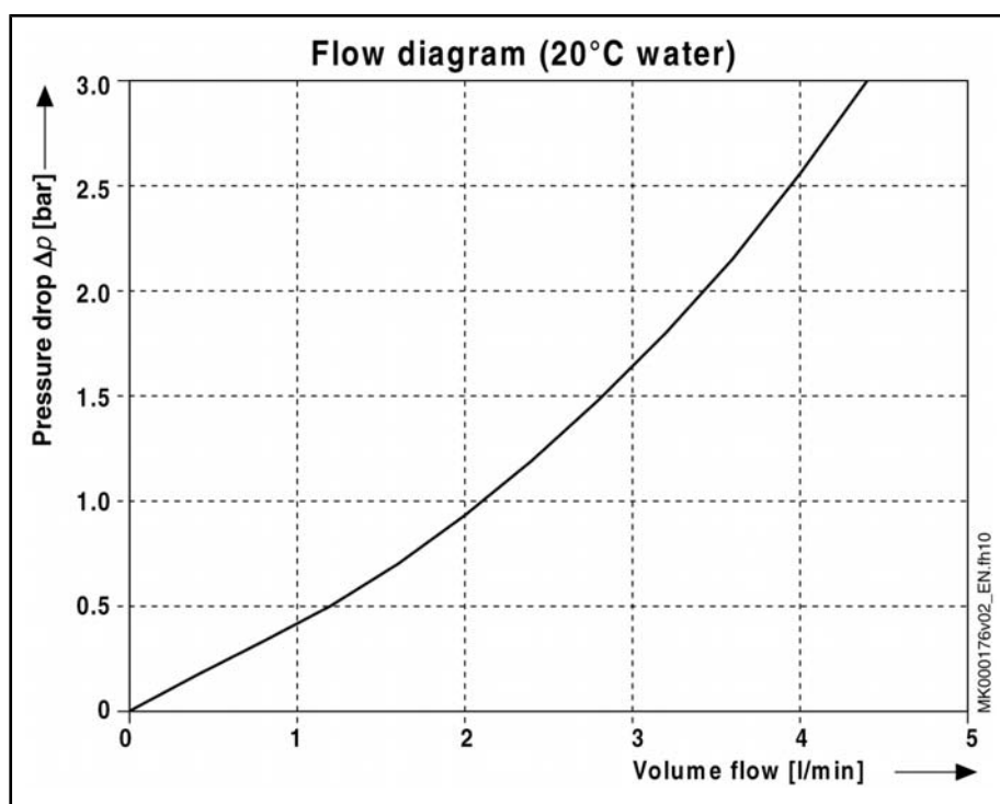
Fig.9-24: Discharge-diagram for MSK motors
