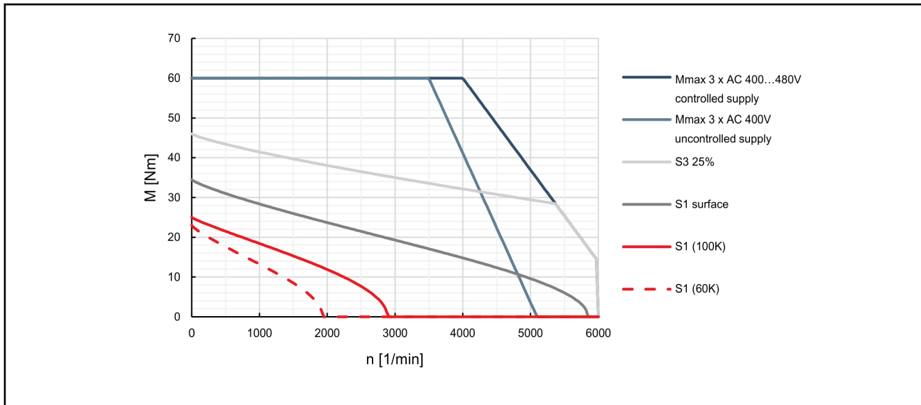
Fig. 4-32: Characteristic curves of motor MSK070E-0450
