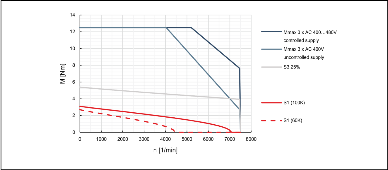
Fig. 4-9: Characteristic curves of motor MSK043C-0600
