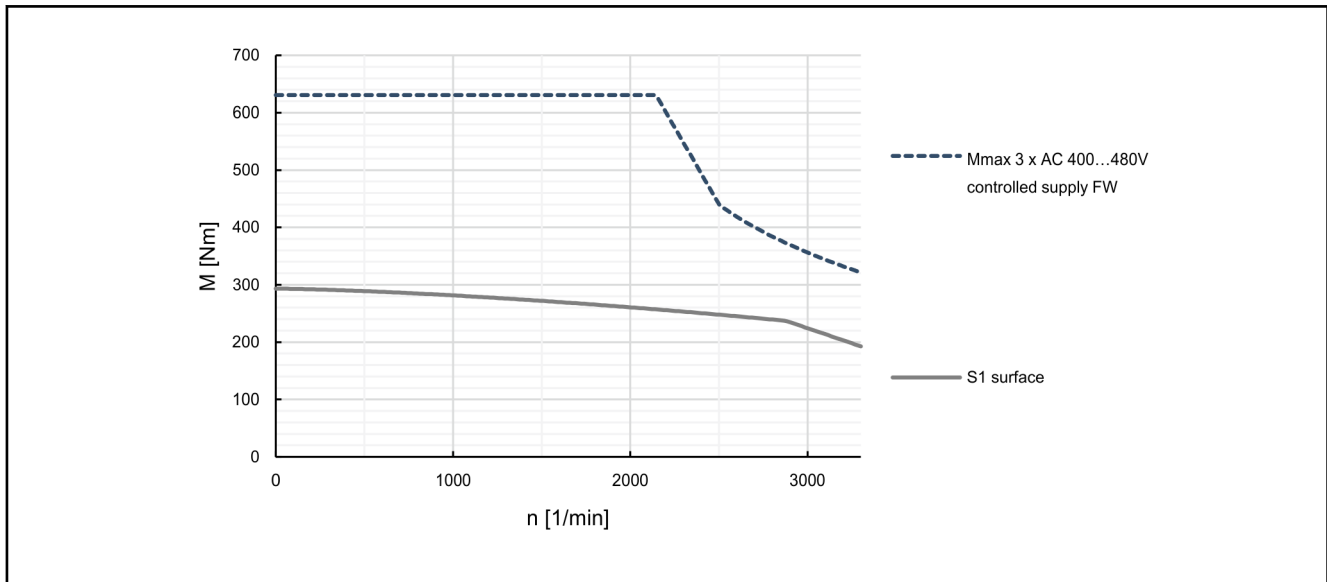
Fig. 4-95: Characteristic curves of motor MSK133E-0202-SA, controlled supply 3 x AC 400 V (-5%) with reluctance characteristic curve and field weakening
