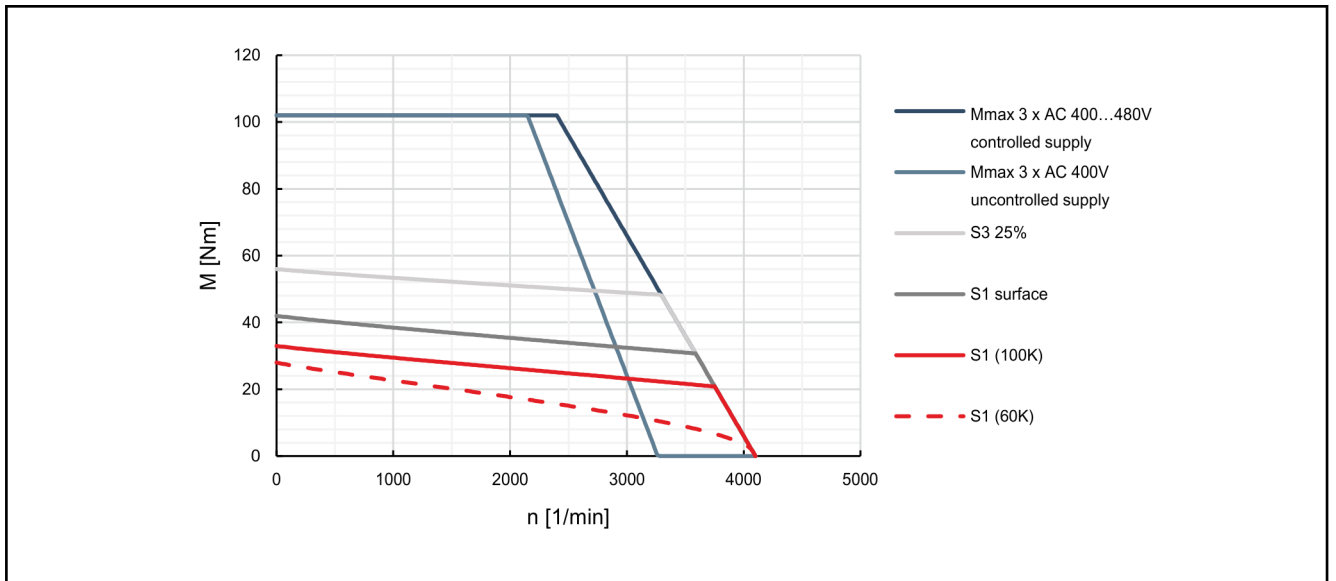
Fig. 4-56: Characteristic curves of motor MSK100B-0200
