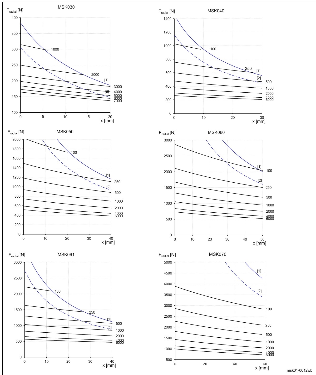
[1] Shaft plain [2] Shaft with keyway n [min -1 ] Average speed Fig. 9-8: Radial force F_{radial}(1)
