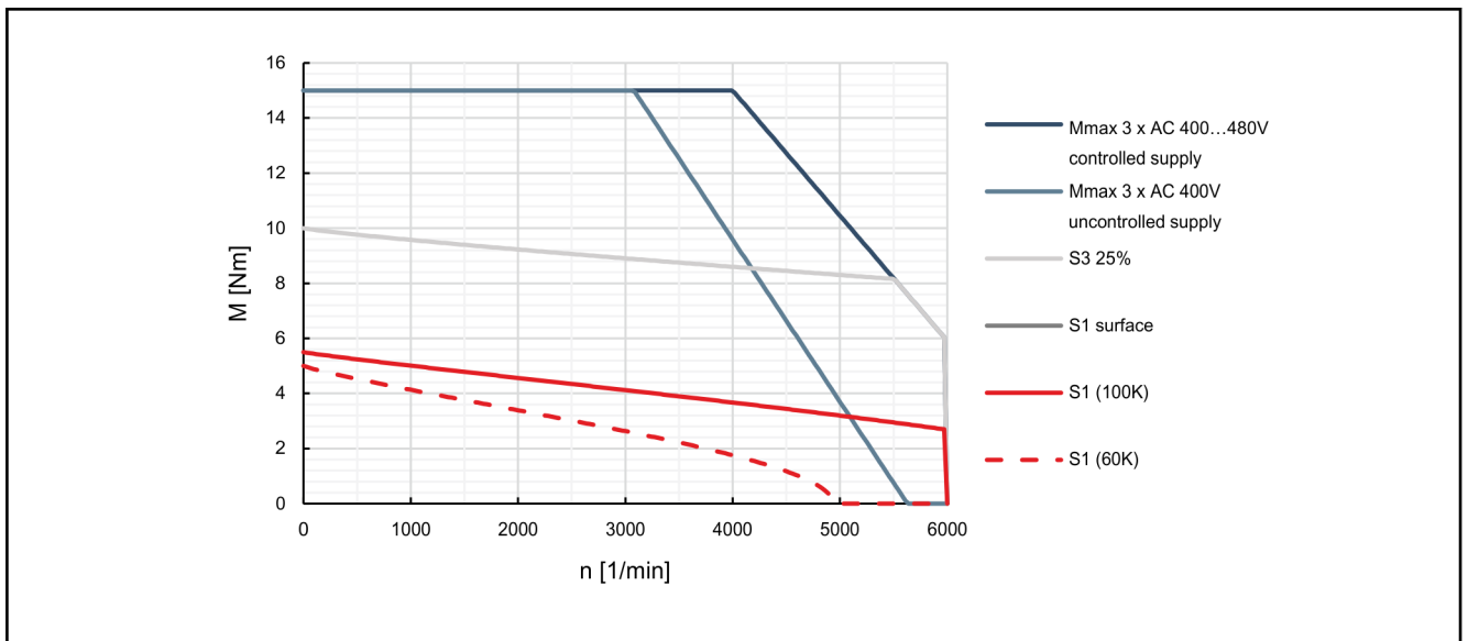
Fig. 4-14: Characteristic curves of motor MSK050C-0450
