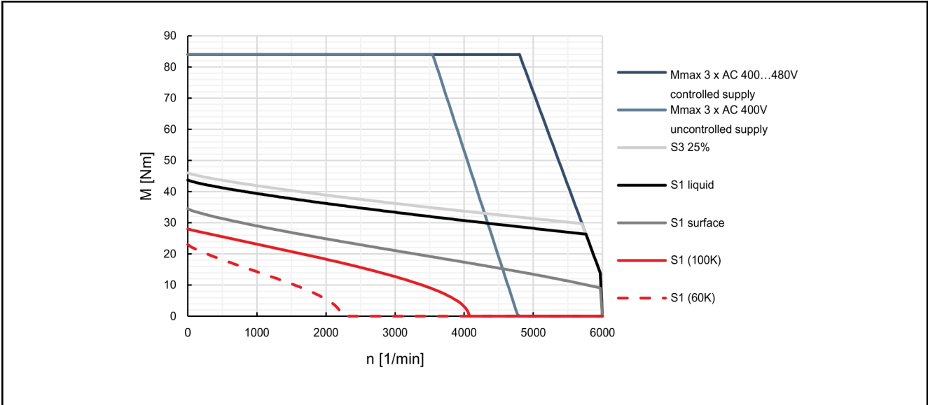
Fig. 4-41: Characteristic curves of motor MSK071E-0450
