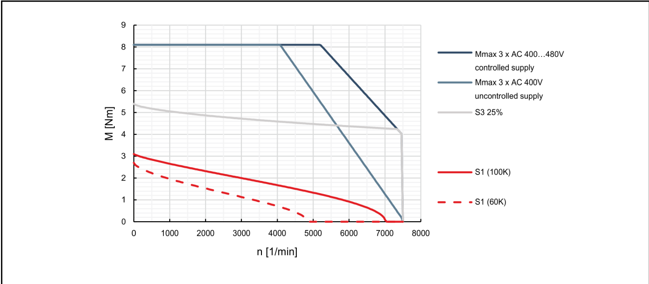
Fig. 4-8: Characteristic curves of motor MSK040C-0600
