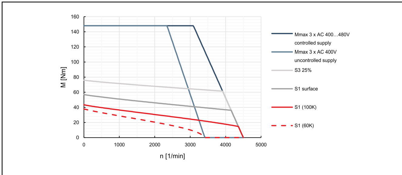
Fig. 4-61: Characteristic curves of motor MSK100C-0300
