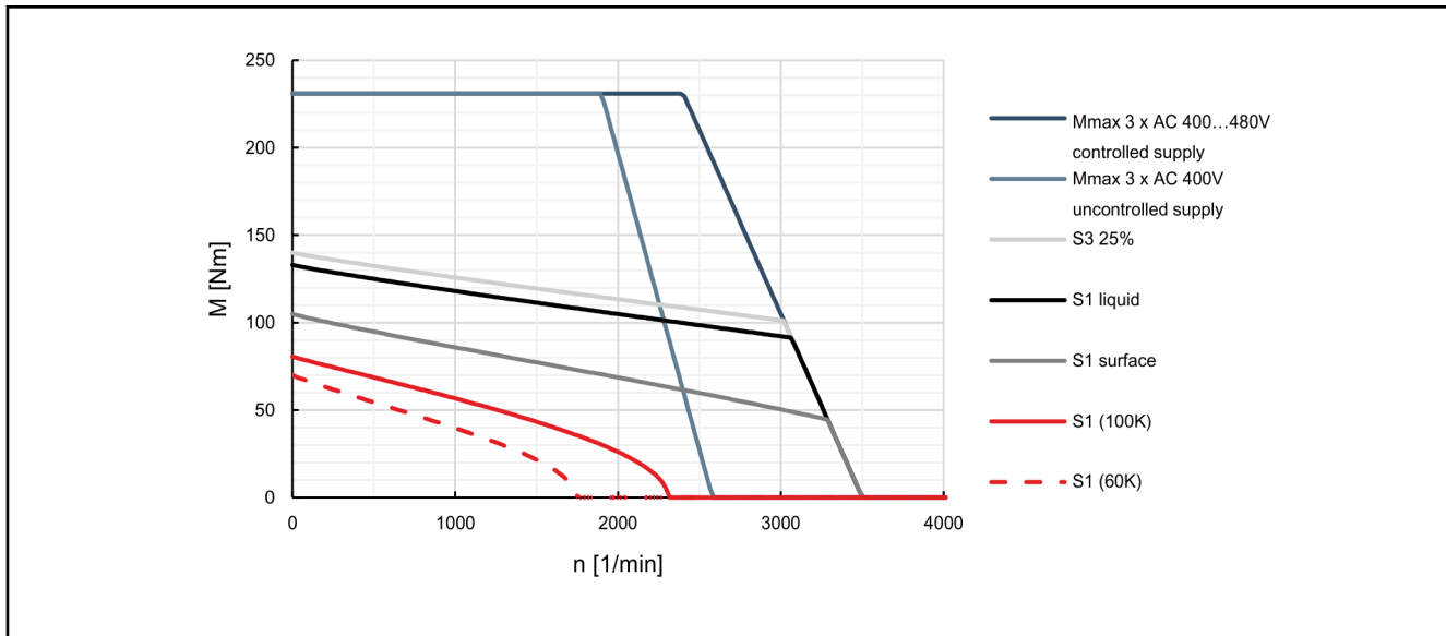
Fig. 4-72: Characteristic curves of motor MSK101E-0200
