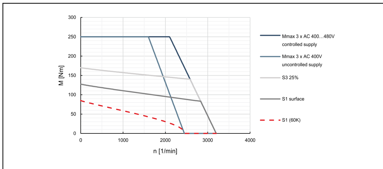
Fig. 4-78: Characteristic curves of motor MSK131B-0200
