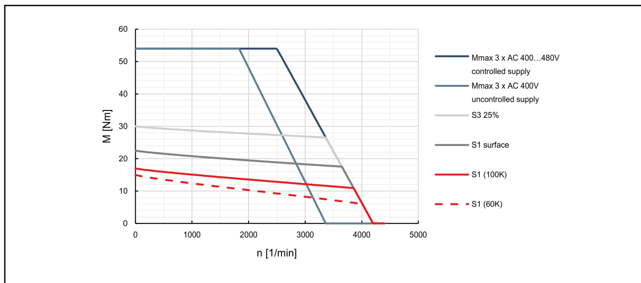
Fig. 4-53: Characteristic curves of motor MSK100A-0200
