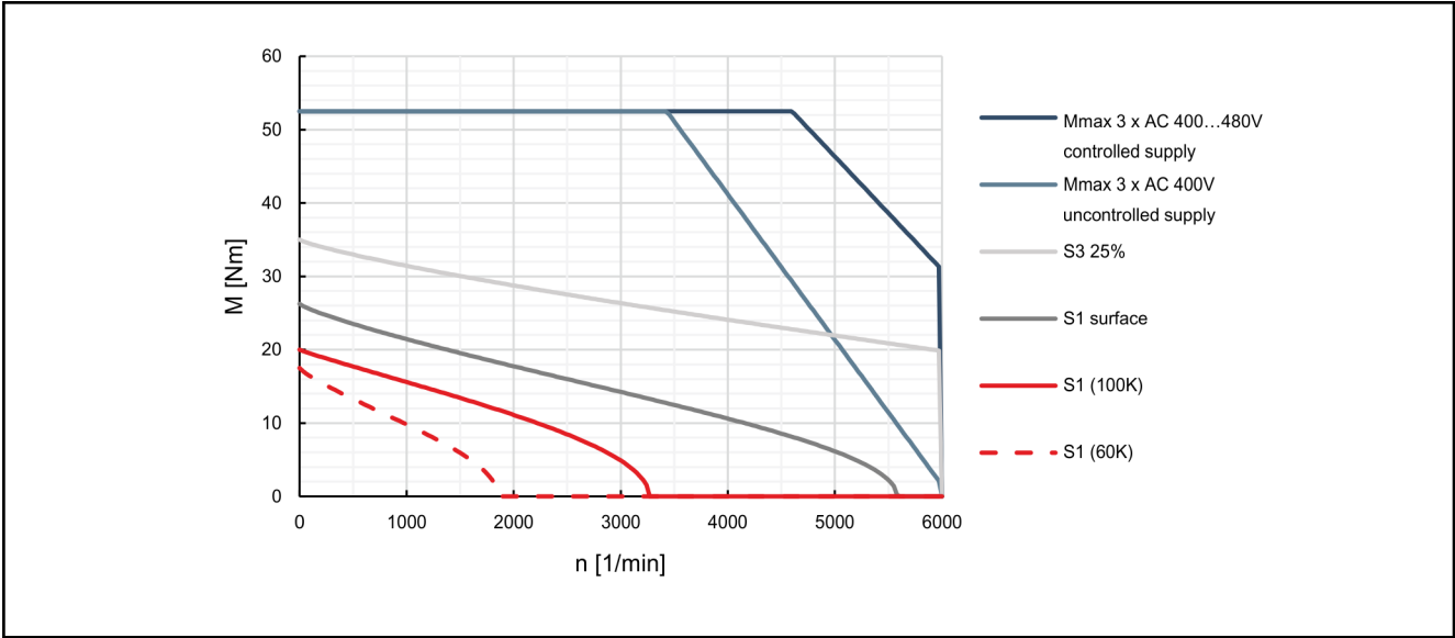
Fig. 4-29: Characteristic curves of motor MSK070D-0450
