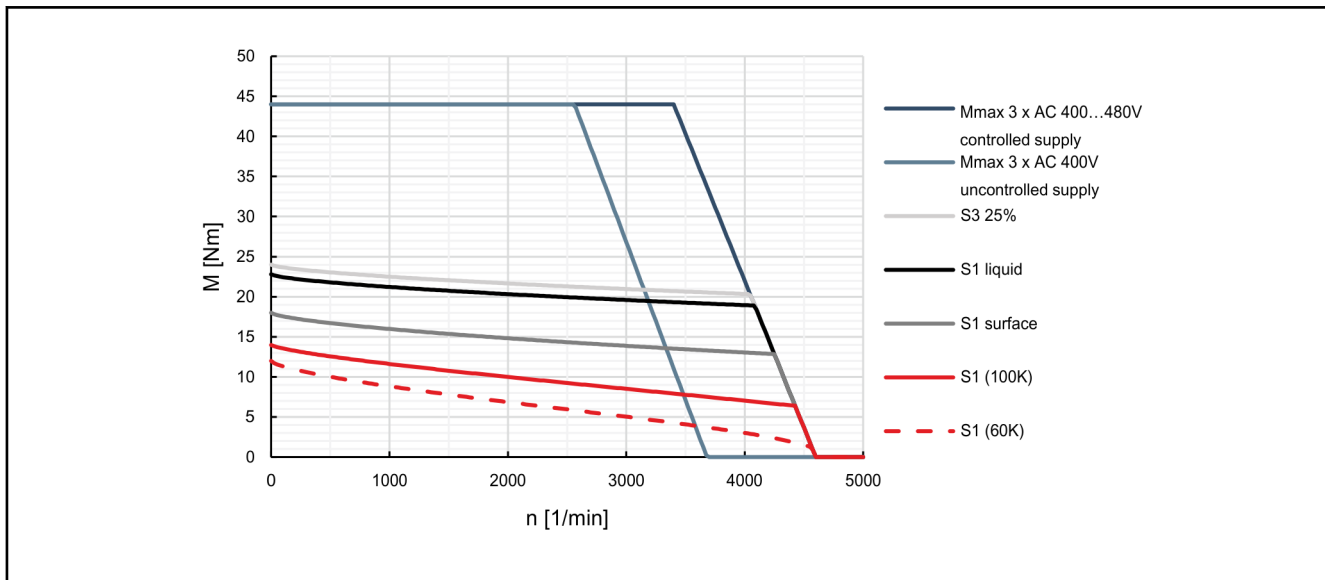
Fig. 4-34: Characteristic curves of motor MSK071C-0300
