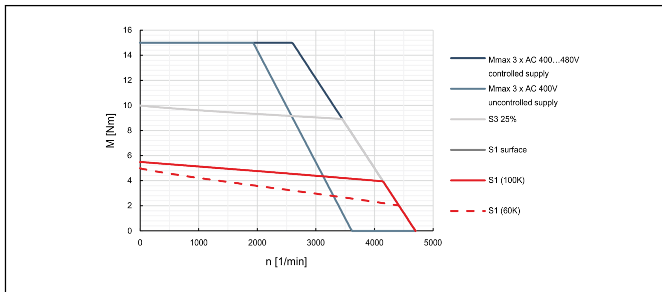
Fig. 4-13: Characteristic curves of motor MSK050C-0300
