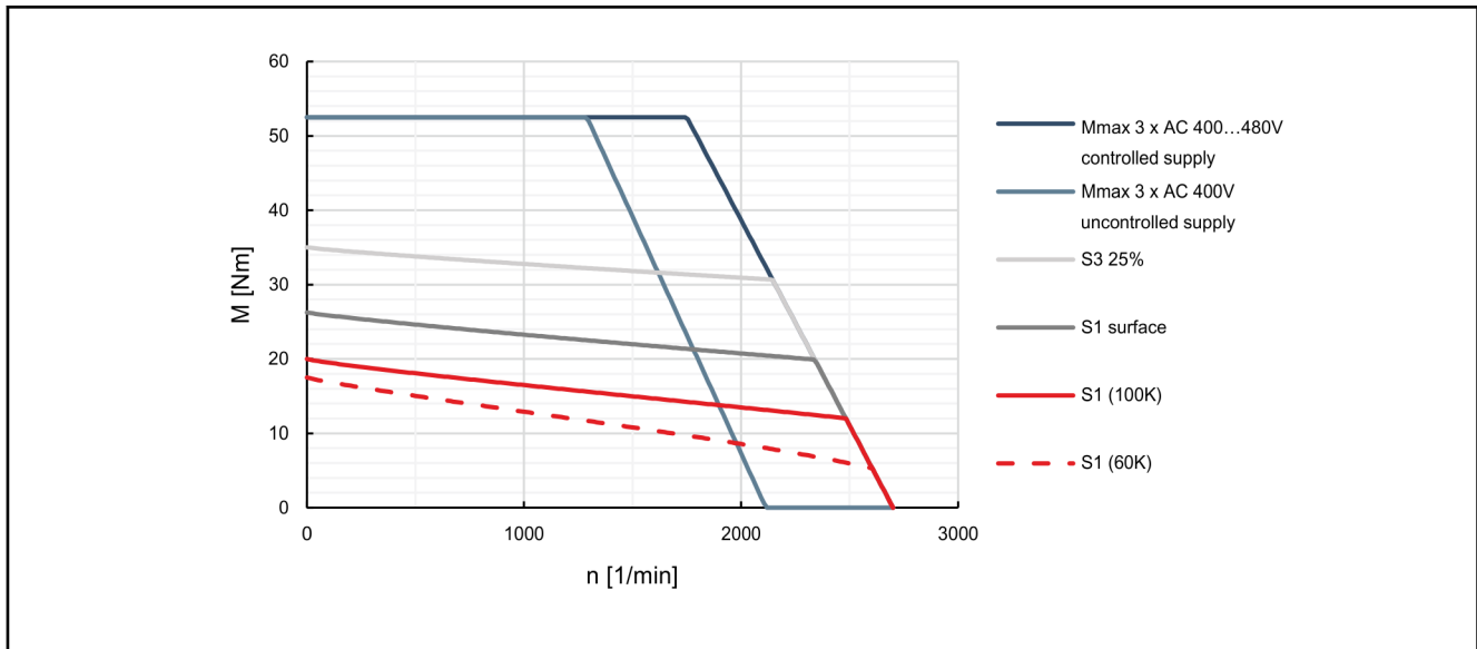
Fig. 4-27: Characteristic curves of motor MSK070D-0150
