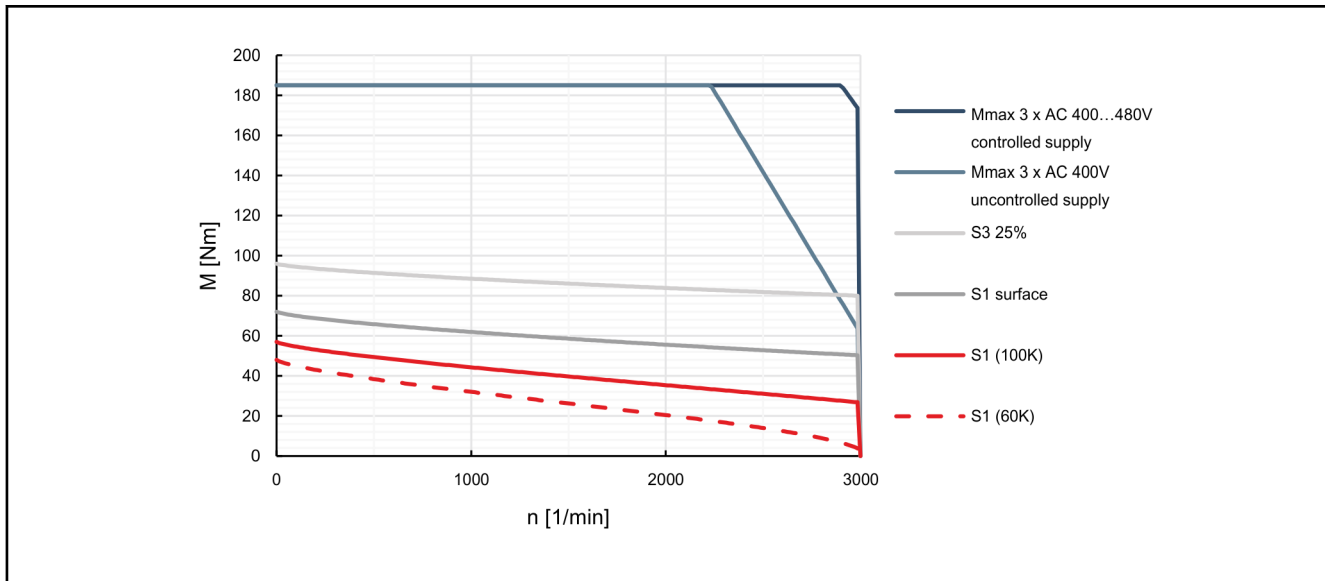
Fig. 4-65: Characteristic curves of motor MSK100D-0350
