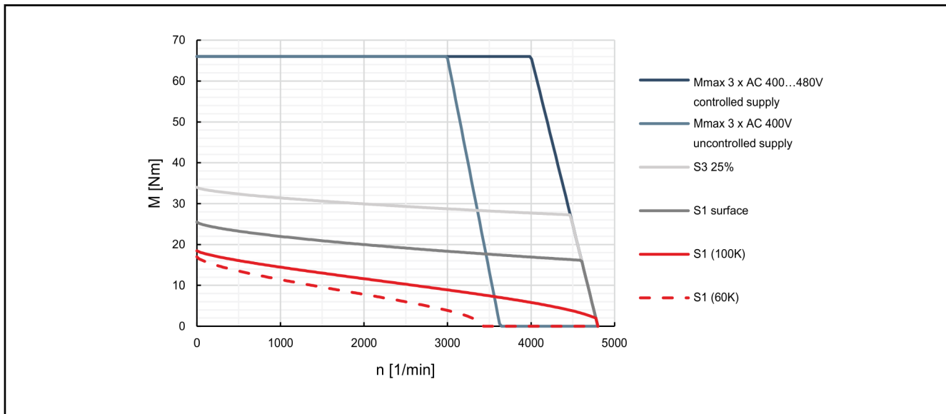
Fig. 4-46: Characteristic curves of motor MSK075D-0300
