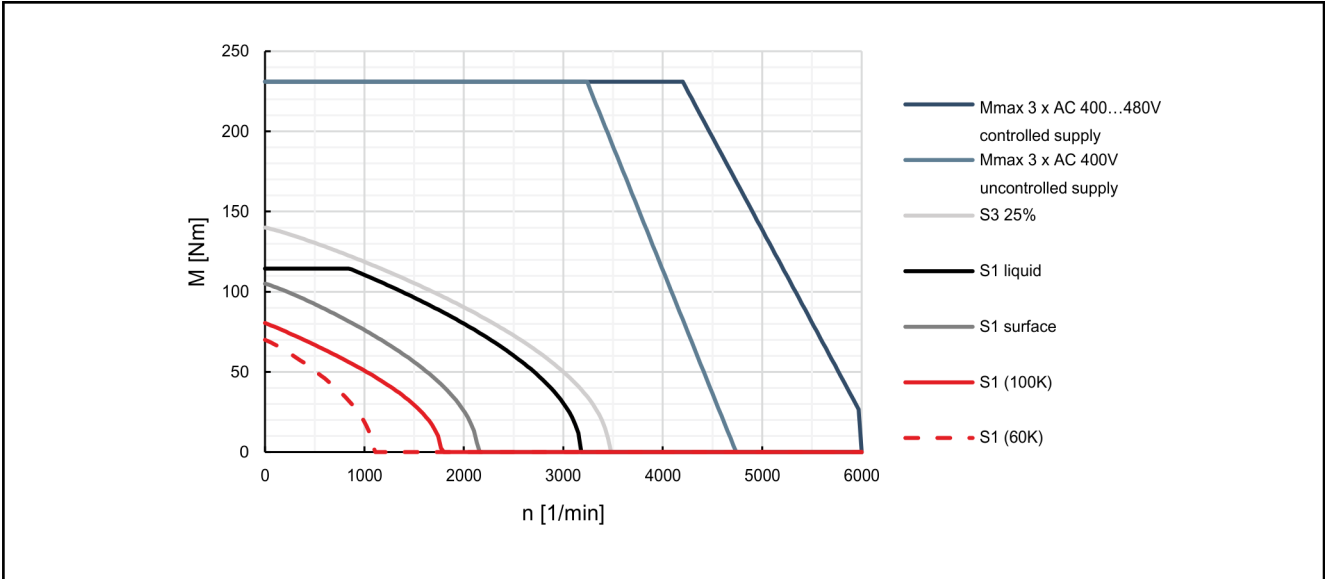
Fig. 4-74: Characteristic curves of motor MSK101E-0450
