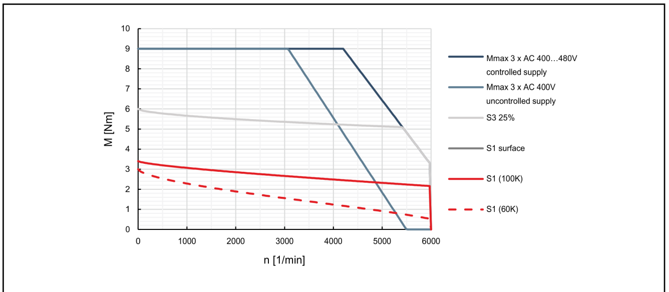
Fig. 4-11: Characteristic curves of motor MSK050B-0450
