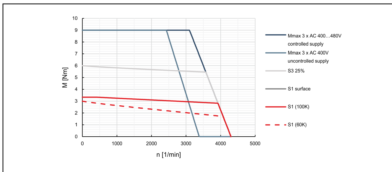
Fig. 4-10: Characteristic curves of motor MSK050B-0300
