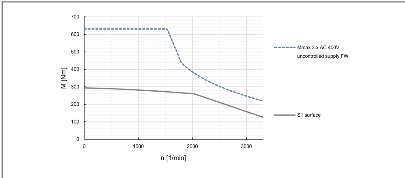
Fig. 4-94: Characteristic curves of motor MSK133E-0202-SA, uncontrolled supply 3 x AC 400 V (-5%) with reluctance characteristic curve and field weakening
