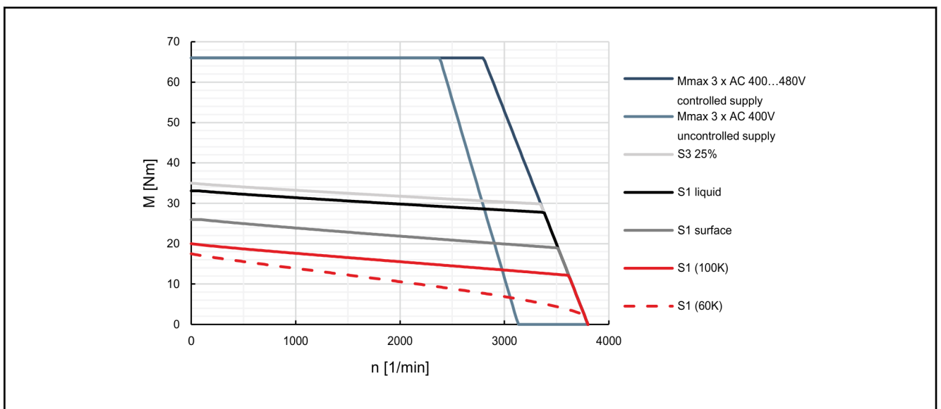
Fig. 4-37: Characteristic curves of motor MSK071D-0300
