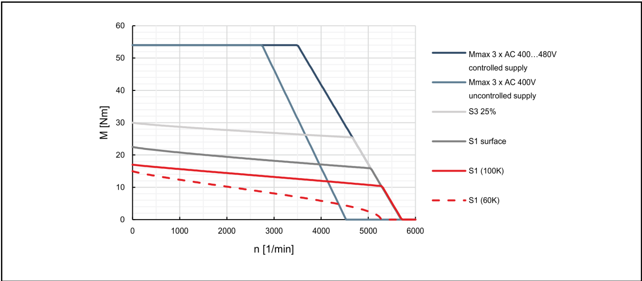
Fig. 4-55: Characteristic curves of motor MSK100A-0450
