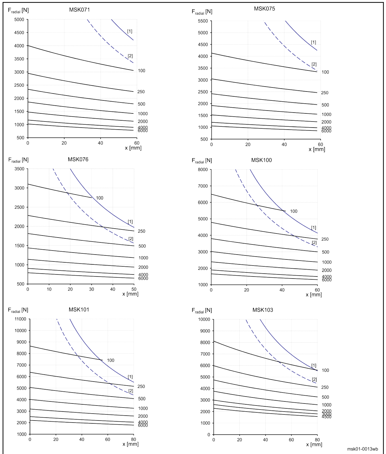
[1] Shaft plain [2] Shaft with keyway n [min -1 ] Average speed Fig. 9-9: Radial force F_{\text{radial}}(2)
