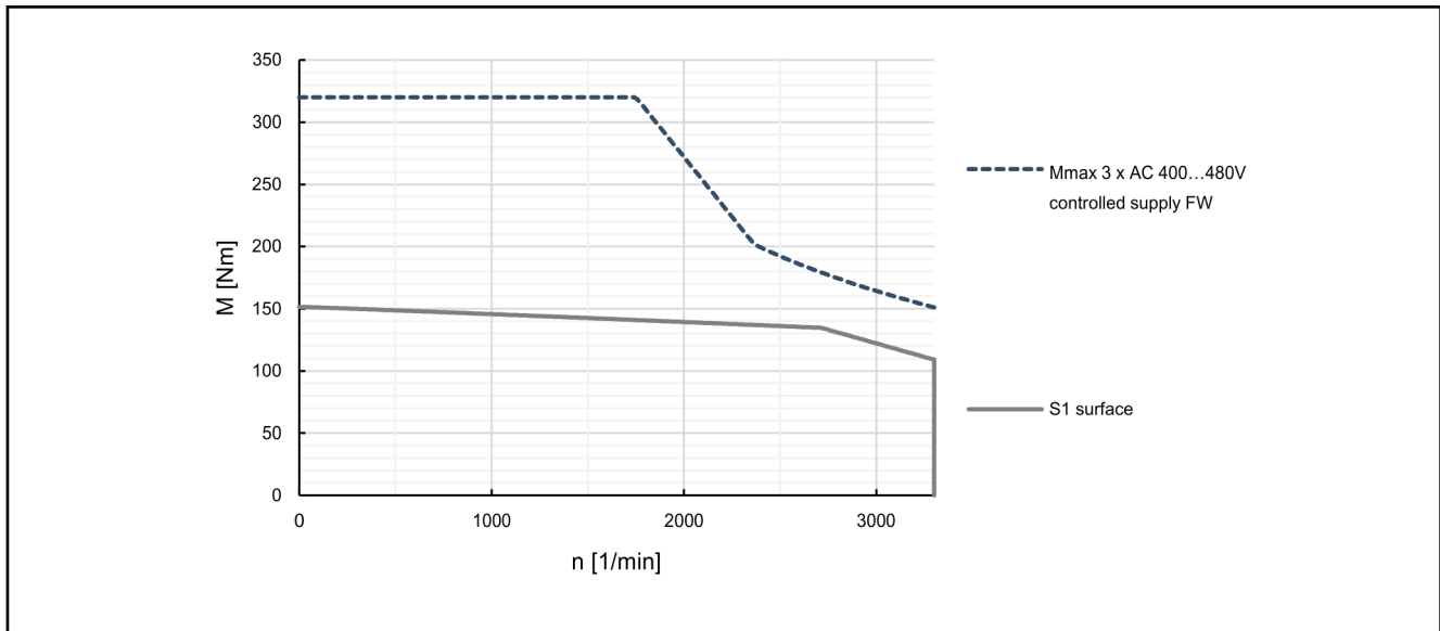
Fig. 4-81: Characteristic curves of motor MSK133B-0202-SA, controlled supply 3 x AC 400 V (-5%) with reluctance characteristic curve and field weakening
