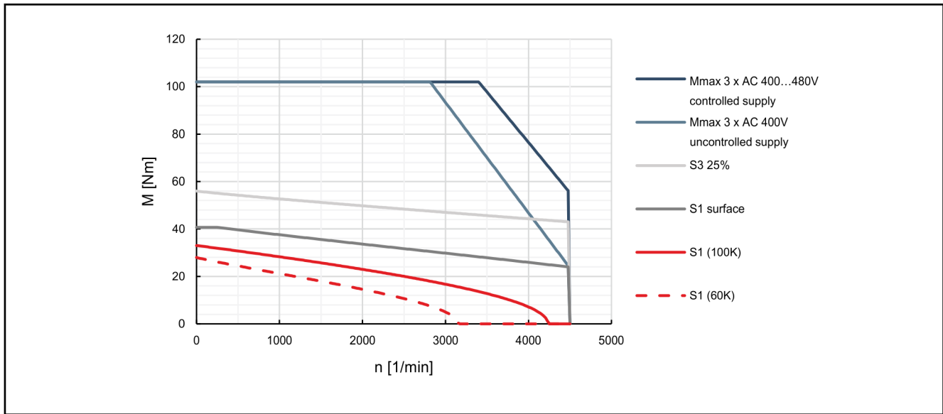
Fig. 4-58: Characteristic curves of motor MSK100B-0400
