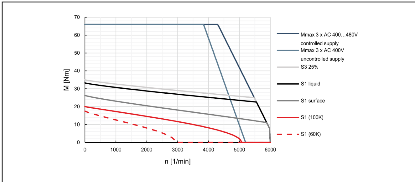
Fig. 4-38: Characteristic curves of motor MSK071D-0450
