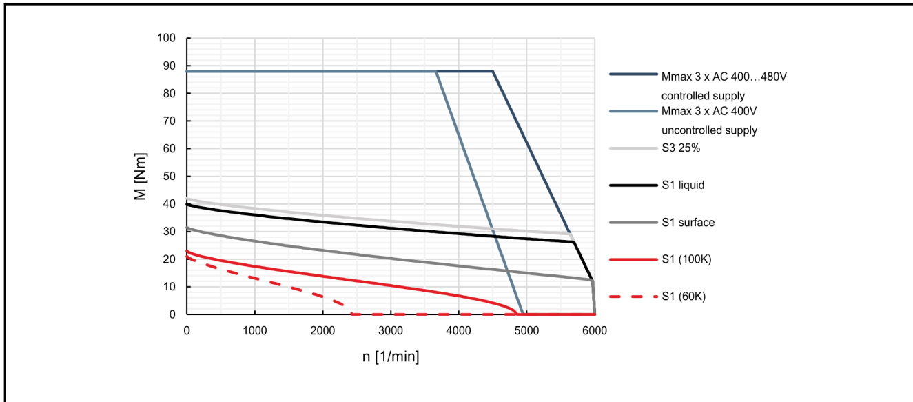
Fig. 4-50: Characteristic curves of motor MSK075E-0450
