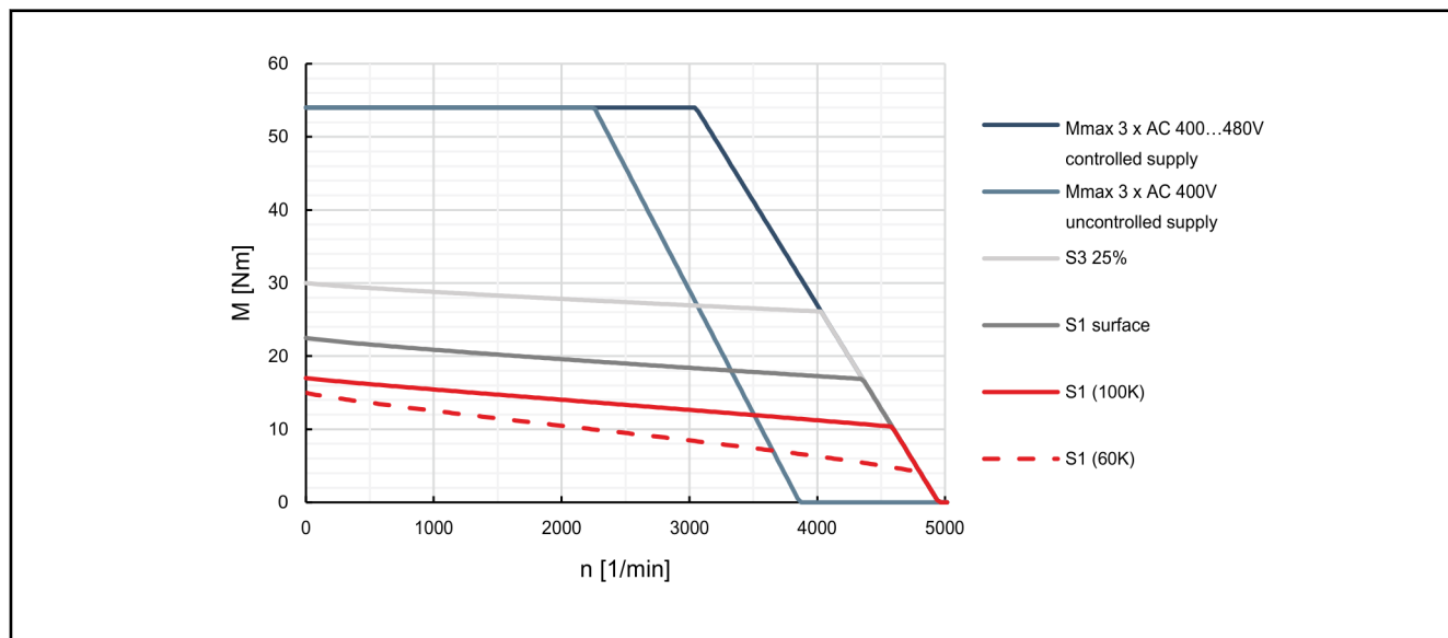
Fig. 4-54: Characteristic curves of motor MSK100A-0300
