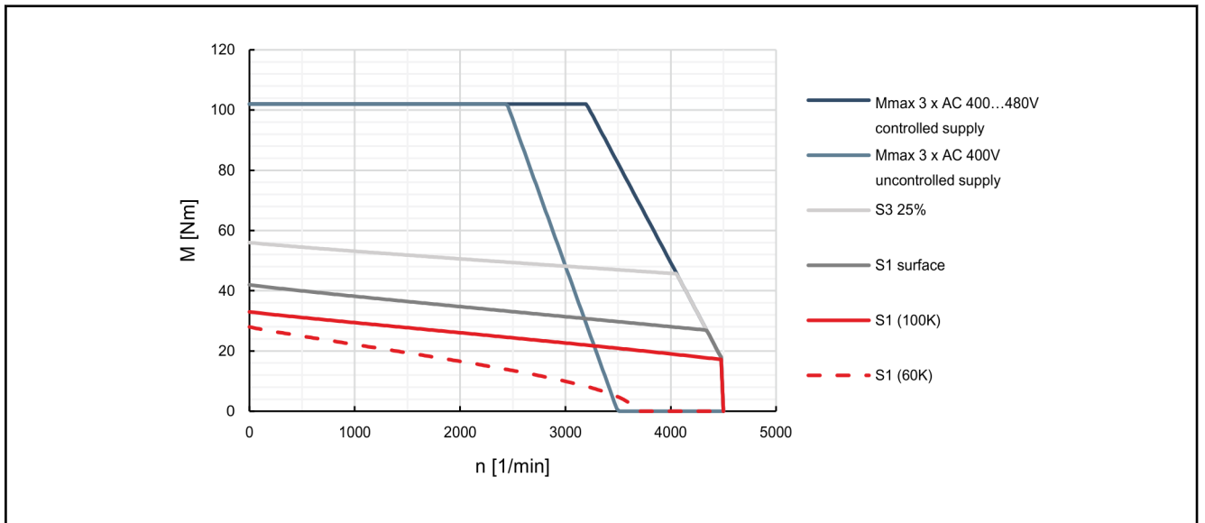
Fig. 4-57: Characteristic curves of motor MSK100B-0300
