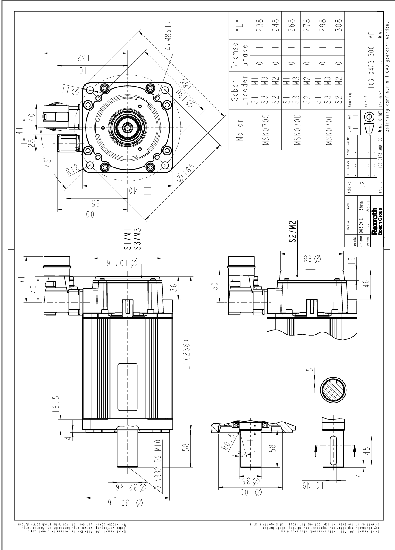
Fig. 5-11: MSK070 specification
