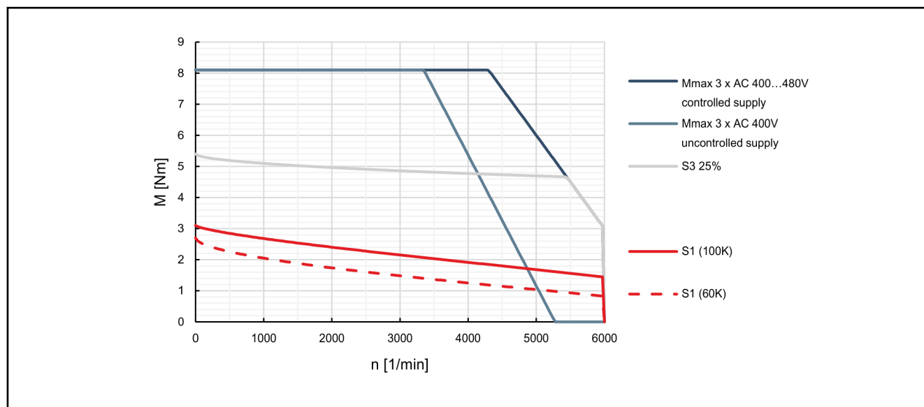
Fig. 4-7: Characteristic curves of motor MSK040C-0450
