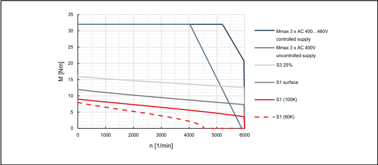
Fig. 4-23: Characteristic curves of motor MSK061C-0600
