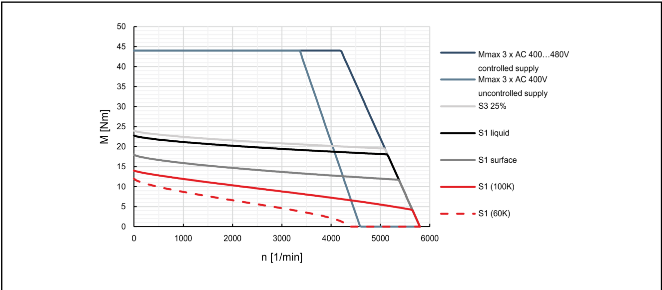
Fig. 4-35: Characteristic curves of motor MSK071C-0450
