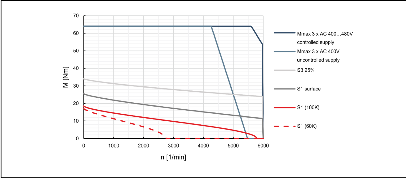
Fig. 4-47: Characteristic curves of motor MSK075D-0450
