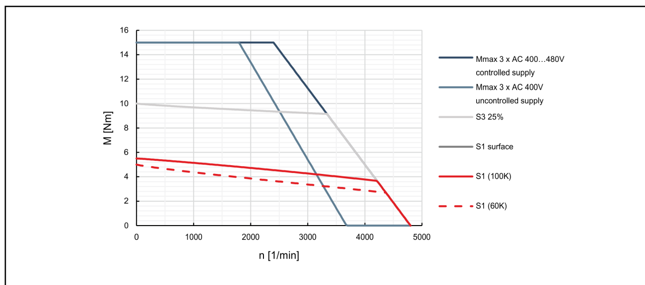
Fig. 4-16: Characteristic curves of motor MSK060B-0300
