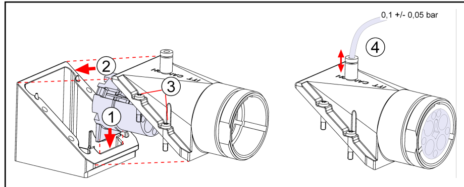
Fig. 7-6: RLS1300 with sealing air connection
