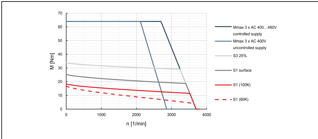
Fig. 4-45: Characteristic curves of motor MSK075D-0200
