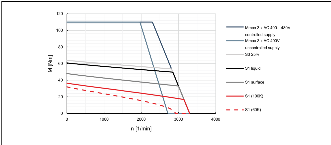
Fig. 4-66: Characteristic curves of motor MSK101C-0200
