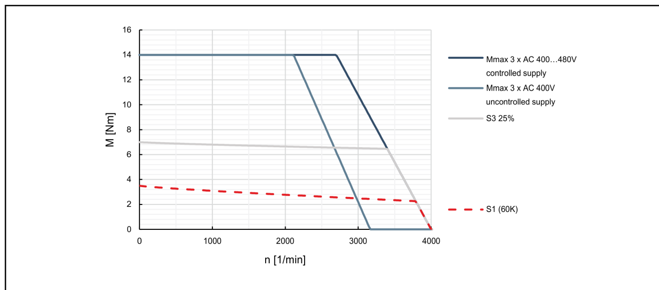
Fig. 4-20: Characteristic curves of motor MSK061B-0300
