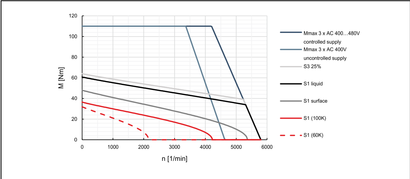
Fig. 4-68: Characteristic curves of motor MSK101C-0450
