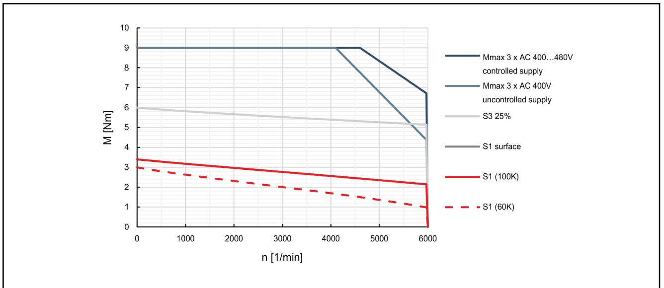
Fig. 4-12: Characteristic curves of motor MSK050B-0600
