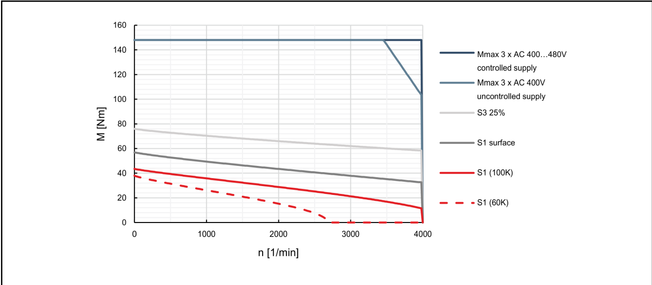
Fig. 4-62: Characteristic curves of motor MSK100C-0450
