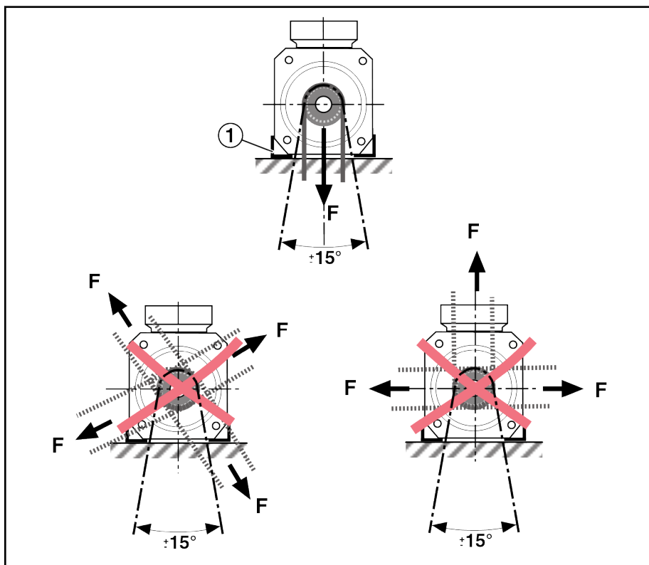
① Mounting feet Fig. 9-3: Foot assembly
