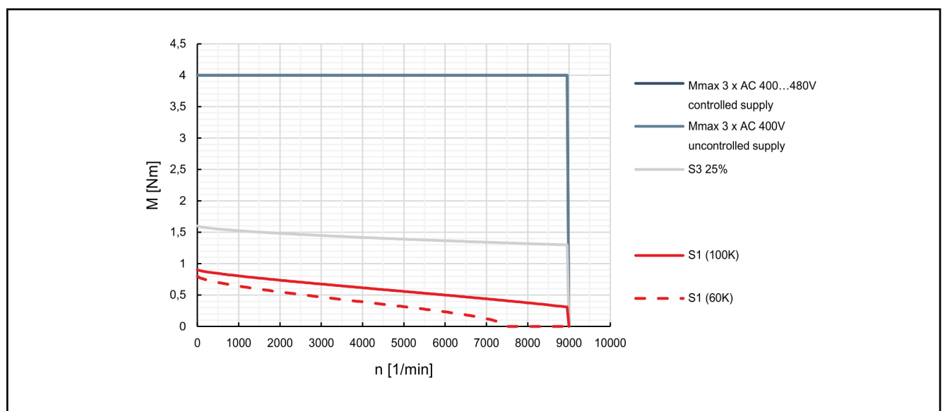
Fig. 4-4: Characteristic curves of motor MSK030C-0900
