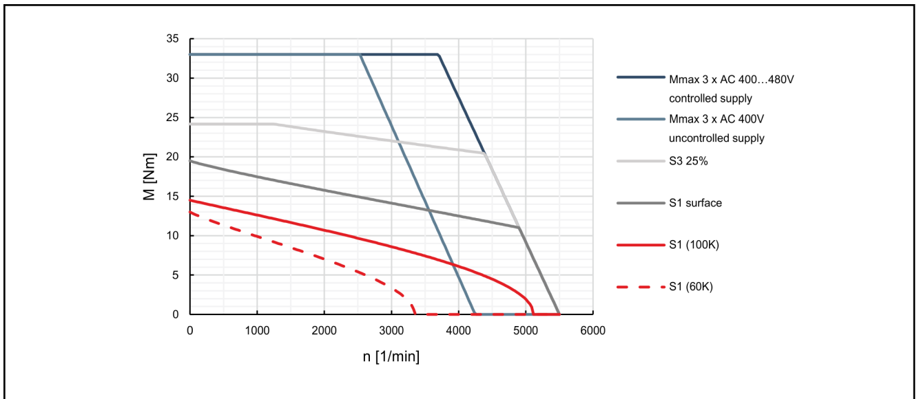
Fig. 4-25: Characteristic curves of motor MSK070C-0300
