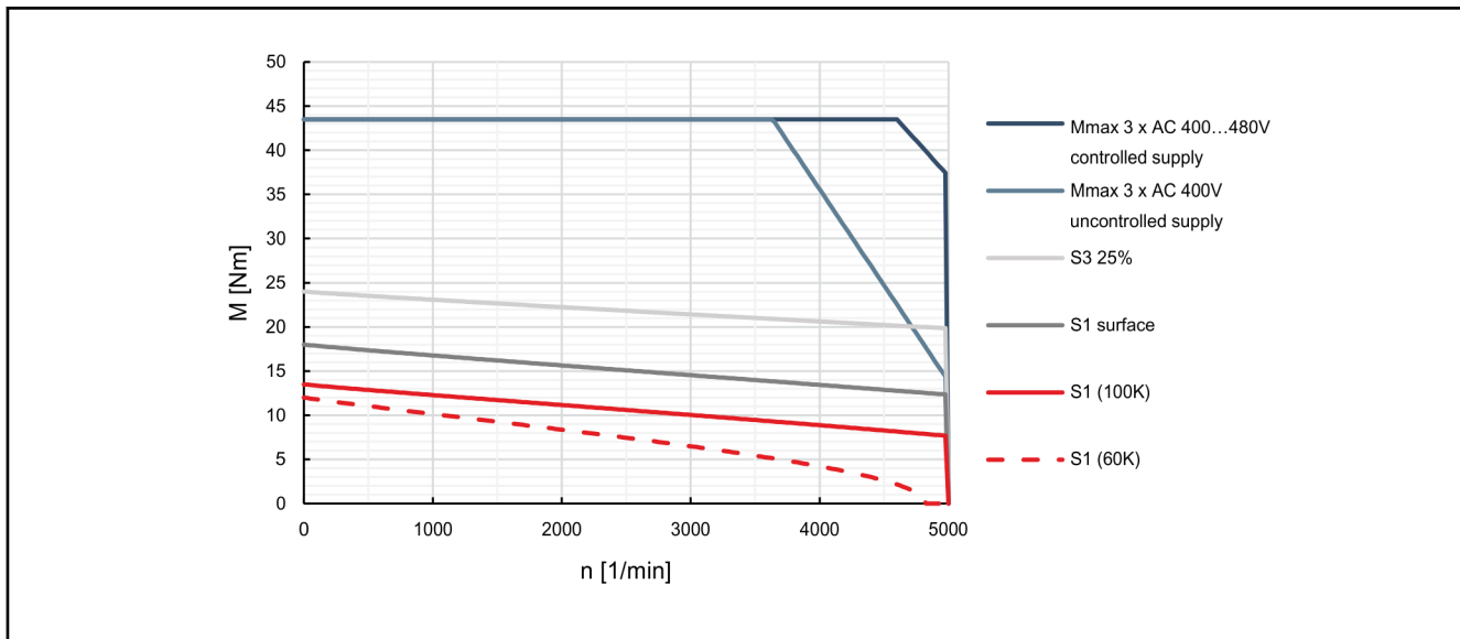
Fig. 4-52: Characteristic curves of motor MSK076C-0450
