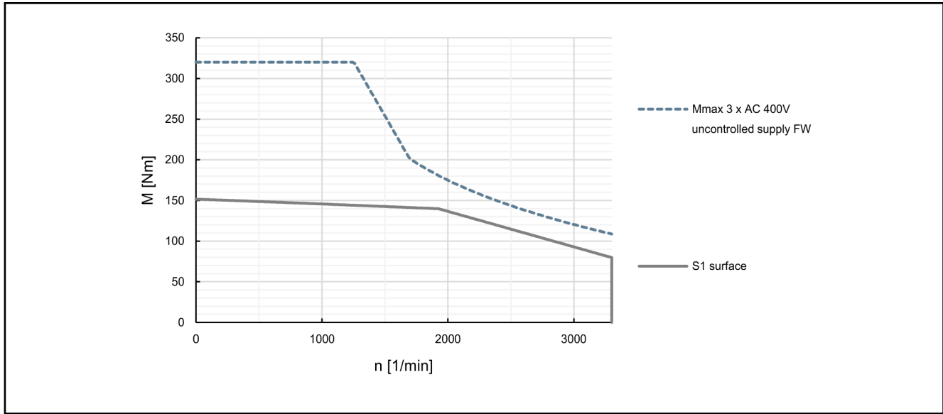
Fig. 4-80: Characteristic curves of motor MSK133B-0202-SA, uncontrolled supply 3 x AC 400 V (-5%) with reluctance characteristic curve and field weakening
