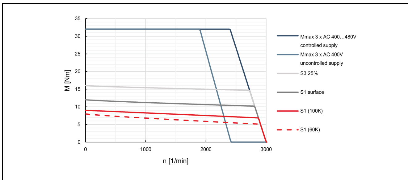
Fig. 4-21: Characteristic curves of motor MSK061C-0200
