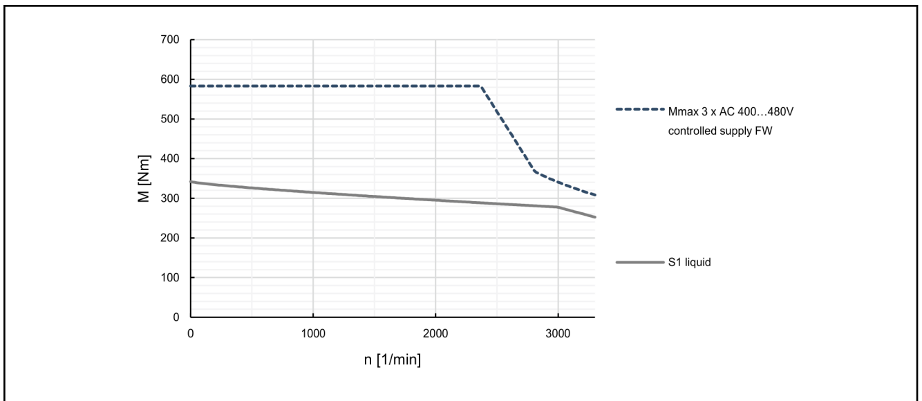
Fig. 4-97: Characteristic curves of motor MSK133E-0203-FN, controlled supply 3 × AC 400 V (-5%) with reluctance characteristic curve and field weakening
