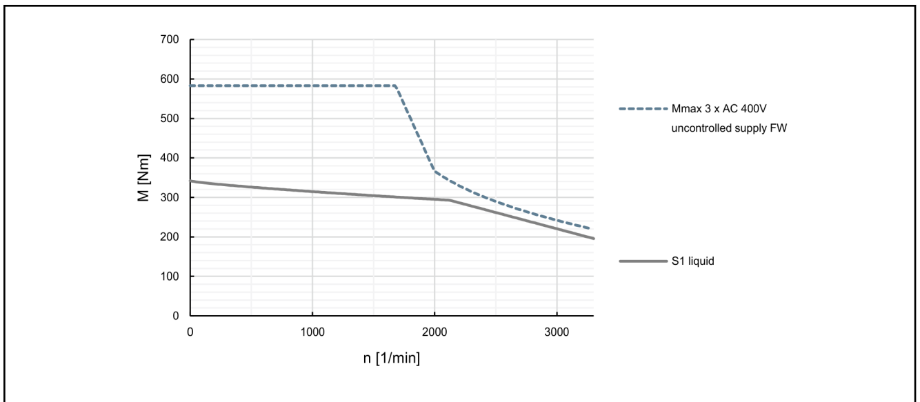
Fig. 4-96: Characteristic curves of motor MSK133E-0203-FN, uncontrolled supply 3 × AC 400 V (-5%) with reluctance characteristic curve and field weakening
