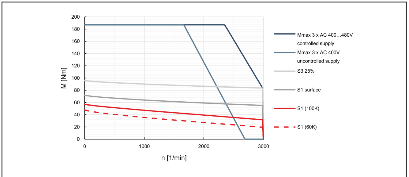
Fig. 4-64: Characteristic curves of motor MSK100D-0300
