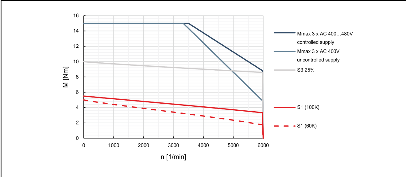
Fig. 4-17: Characteristic curves of motor MSK060B-0600
