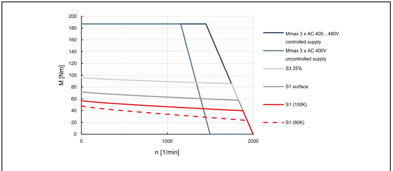
Fig. 4-63: Characteristic curves of motor MSK100D-0200
