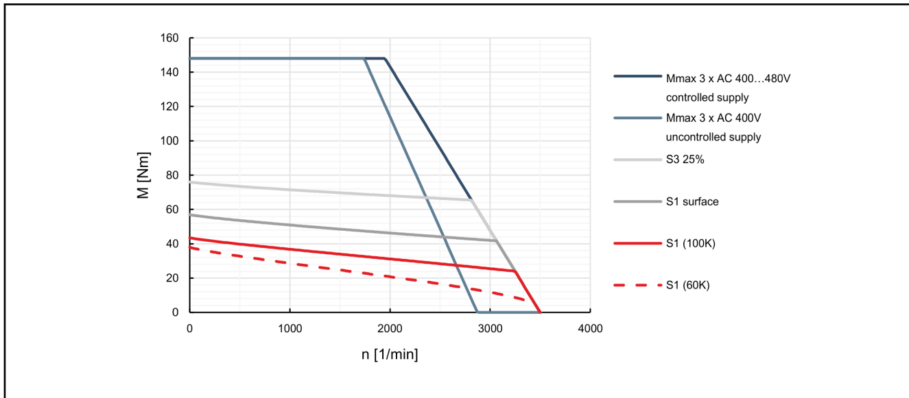
Fig. 4-60: Characteristic curves of motor MSK100C-0200
