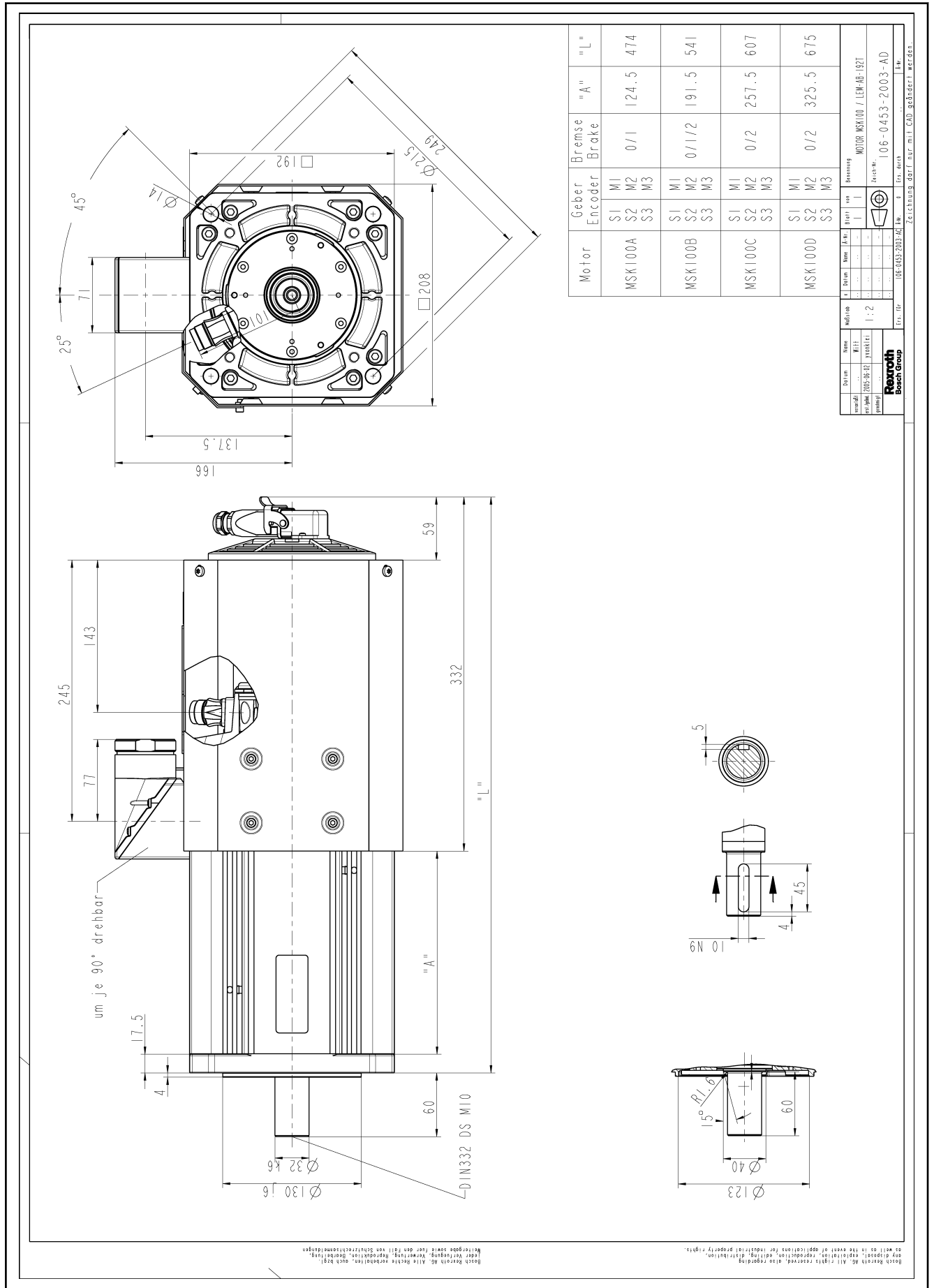
Fig. 5-26: Dimension sheet MSK060 with axial fan unit
