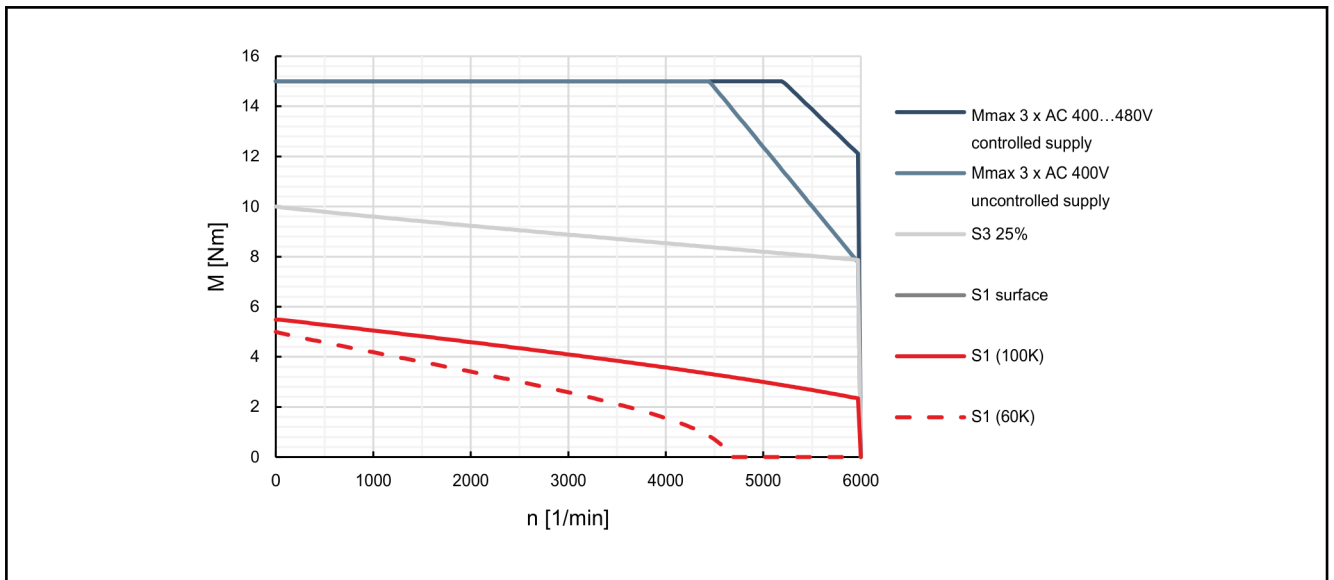
Fig. 4-15: Characteristic curves of motor MSK050C-0600
