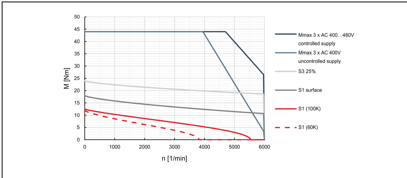
Fig. 4-44: Characteristic curves of motor MSK075C-0450
