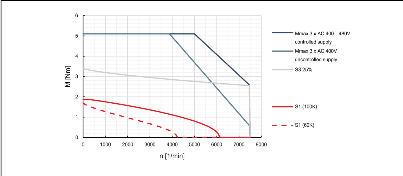
Fig. 4-6: Characteristic curves of motor MSK040B-0600
