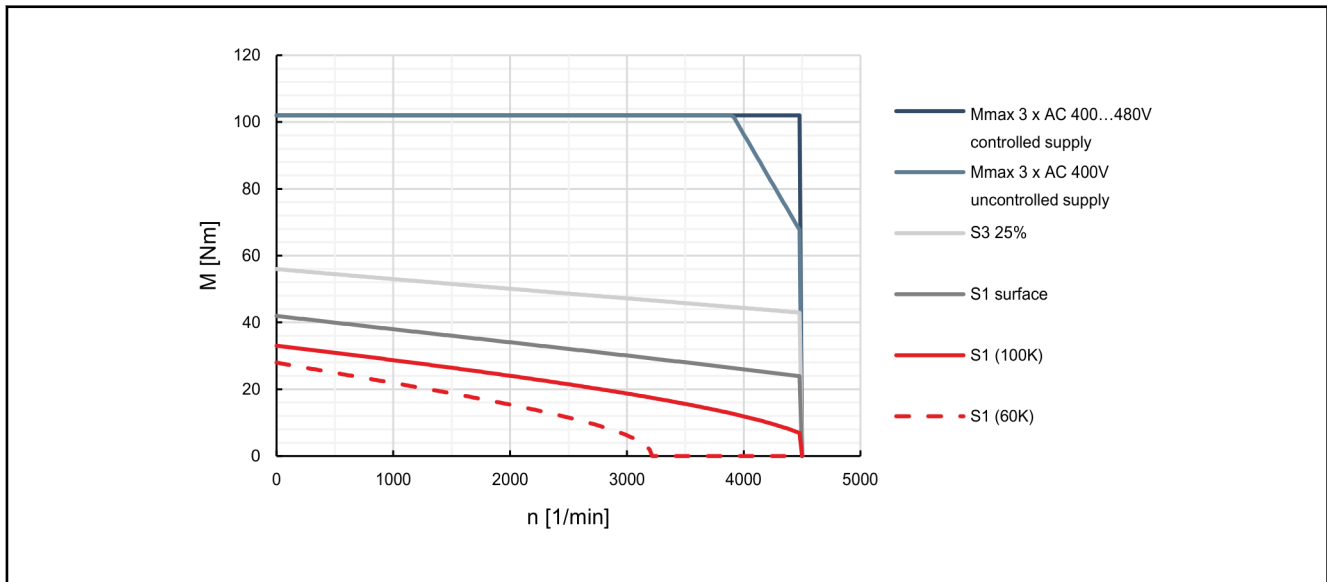
Fig. 4-59: Characteristic curves of motor MSK100B-0450
