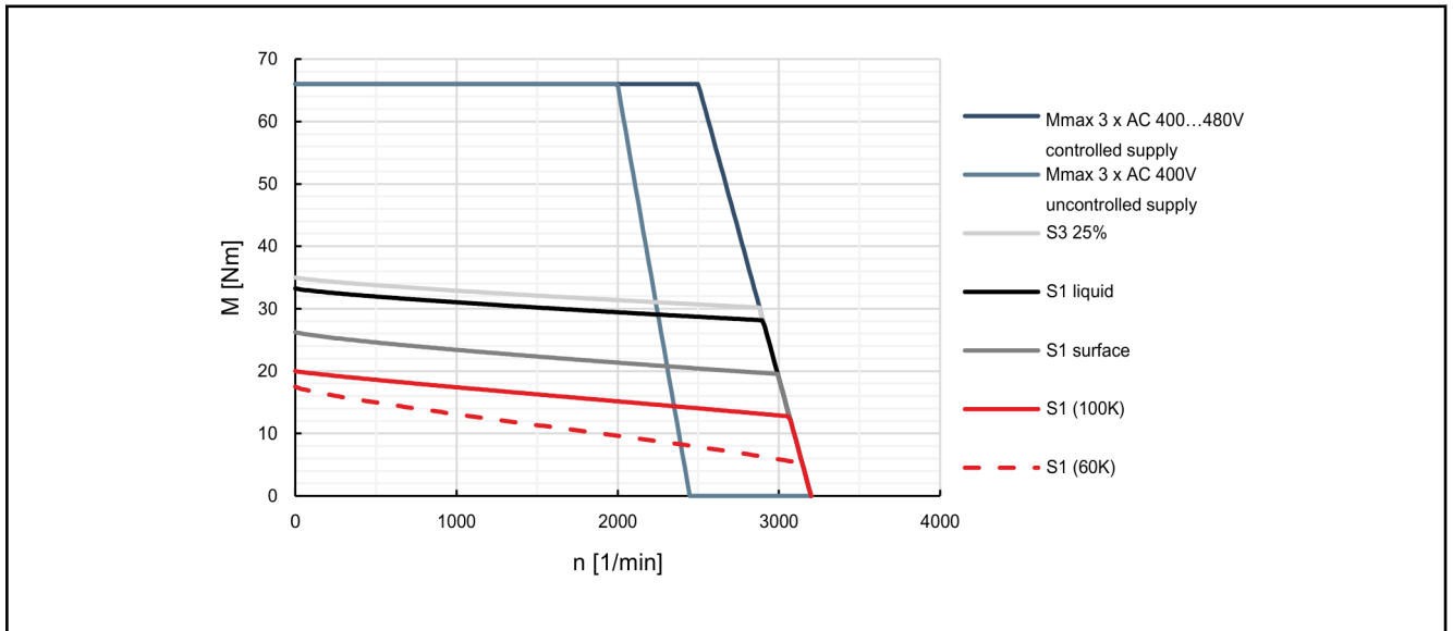
Fig. 4-36: Characteristic curves of motor MSK071D-0200
