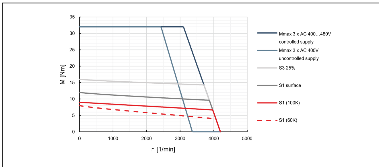
Fig. 4-22: Characteristic curves of motor MSK061C-0300
