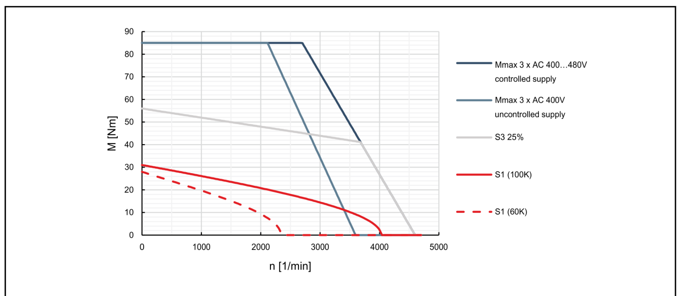
Fig. 4-76: Characteristic curves of motor MSK103B-0300
