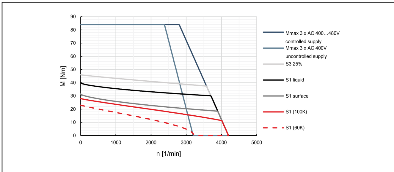
Fig. 4-40: Characteristic curves of motor MSK071E-0300
