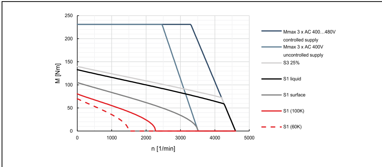
Fig. 4-73: Characteristic curves of motor MSK101E-0300
