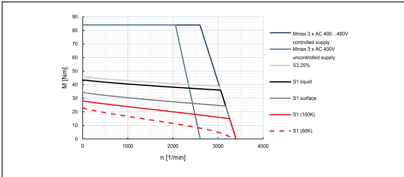
Fig. 4-39: Characteristic curves of motor MSK071E-0200
