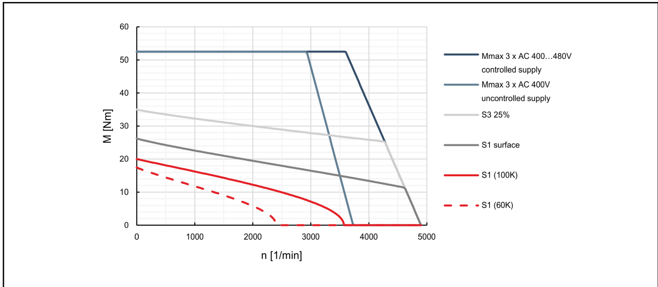
Fig. 4-28: Characteristic curves of motor MSK070D-0300
