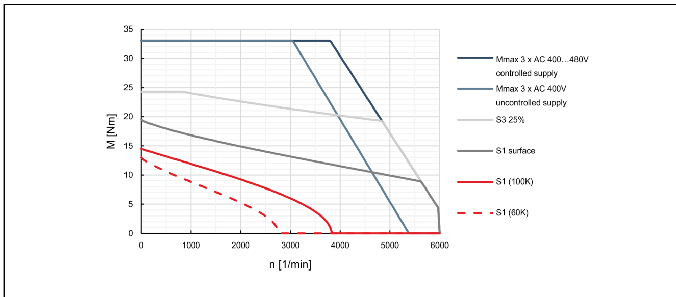
Fig. 4-26: Characteristic curves of motor MSK070C-0450
