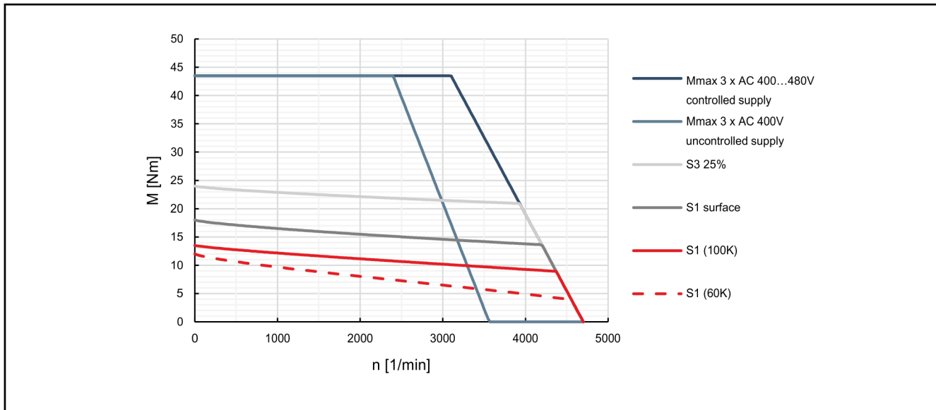
Fig. 4-51: Characteristic curves of motor MSK076C-0300
