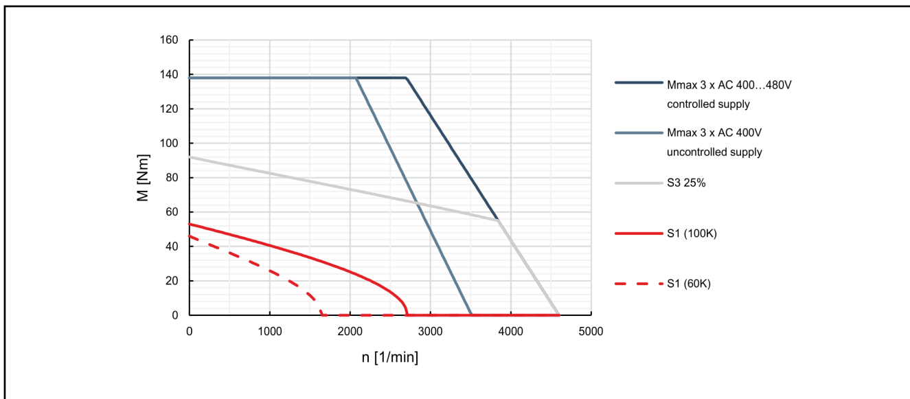
Fig. 4-77: Characteristic curves of motor MSK103D-0300
