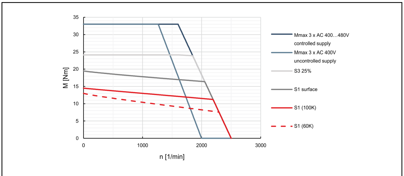
Fig. 4-24: Characteristic curves of motor MSK070C-0150
