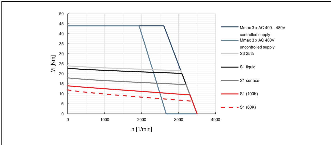
Fig. 4-33: Characteristic curves of motor MSK071C-0200
