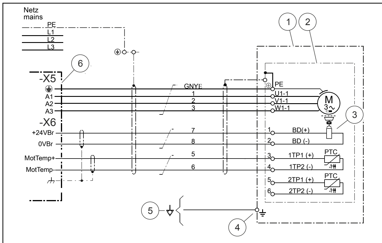
Fig. 12-3: Connection points
