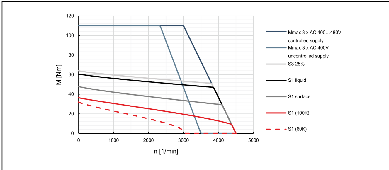
Fig. 4-67: Characteristic curves of motor MSK101C-0300
