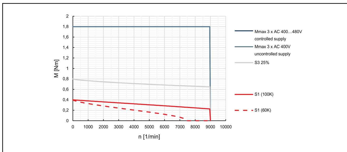
Fig. 4-3: Characteristic curves of motor MSK030B-0900
