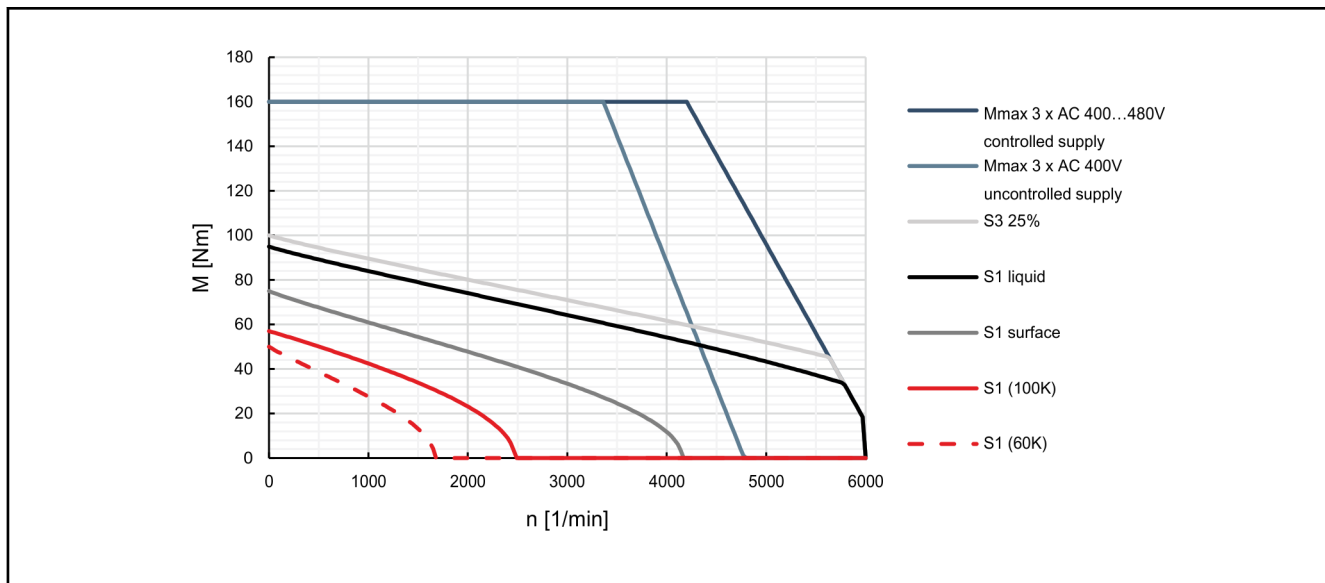
Fig. 4-71: Characteristic curves of motor MSK101D-0450
