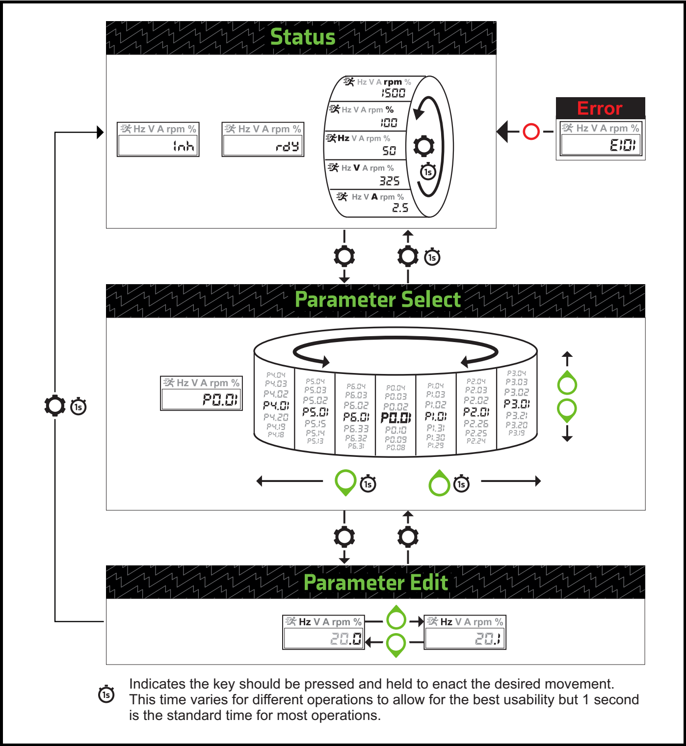
Figure 5-4 Menu structure
