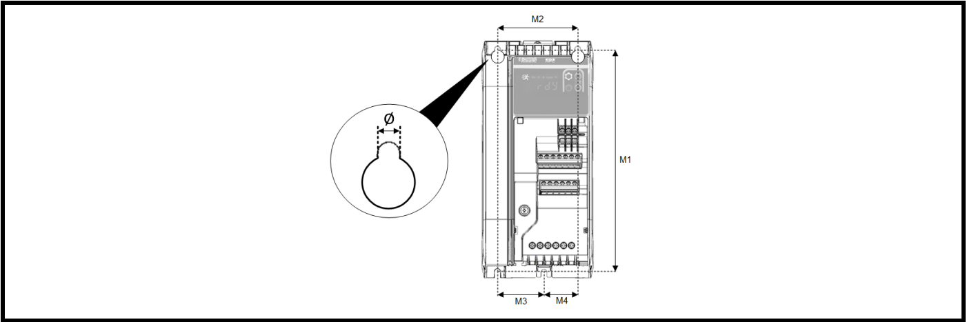
Figure 3-6 Mounting dimensions
