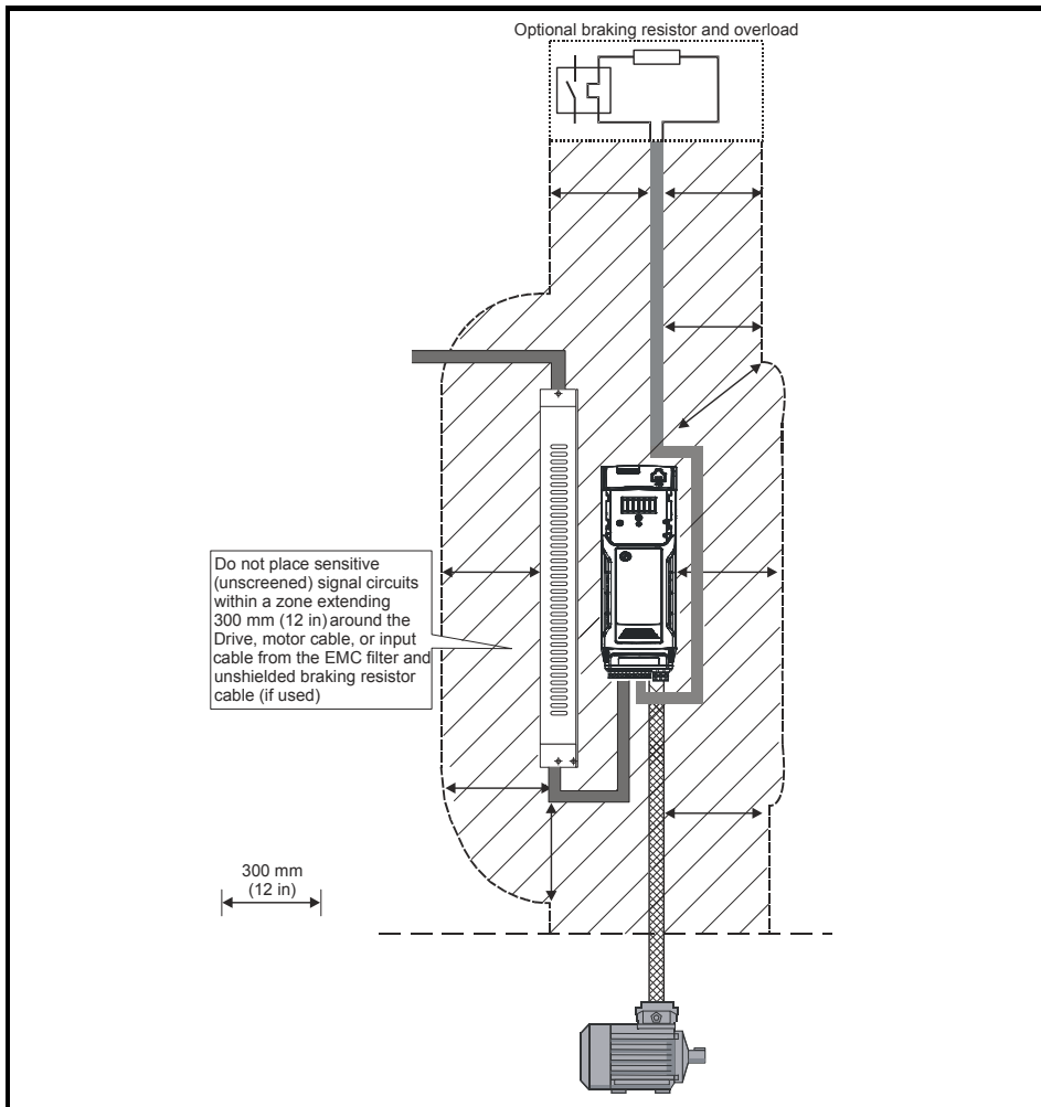
Figure 4-18 Drive cable clearances
