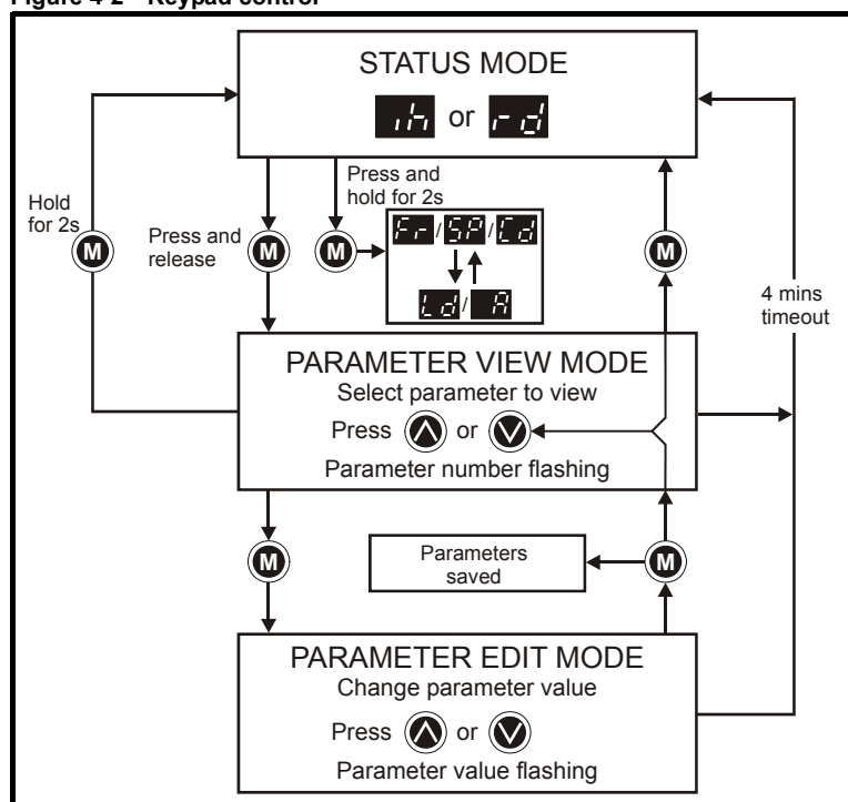
Figure 4-2 Keypad control
