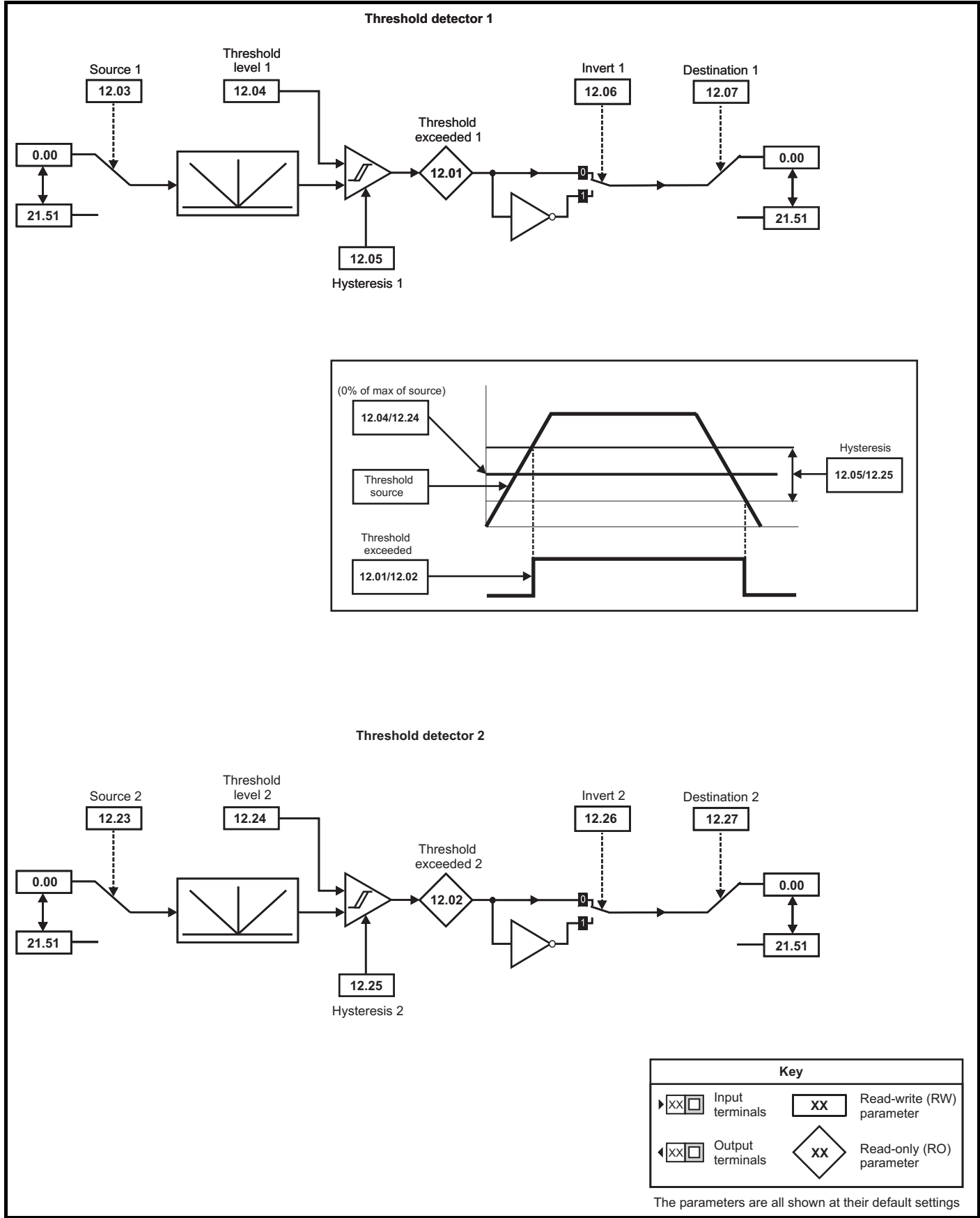
Figure 10-36 Menu 12A logic diagram
