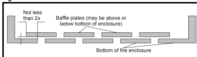
Figure 5-54 Fire enclosure baffle construction
