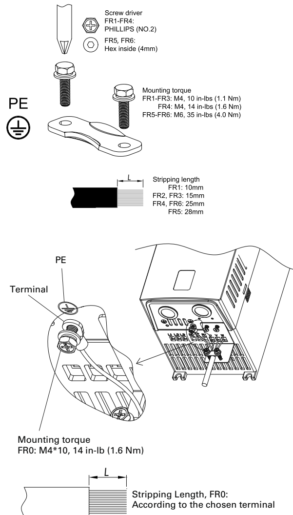
Figure 32. Grounding
