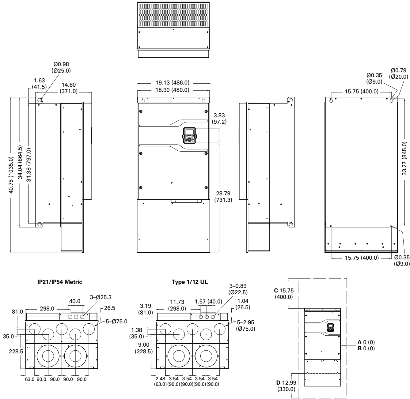
Figure 51. FR6 Dimensional drawing
