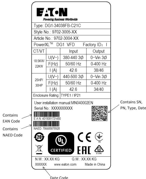
Figure 4. Carton label—DG1
