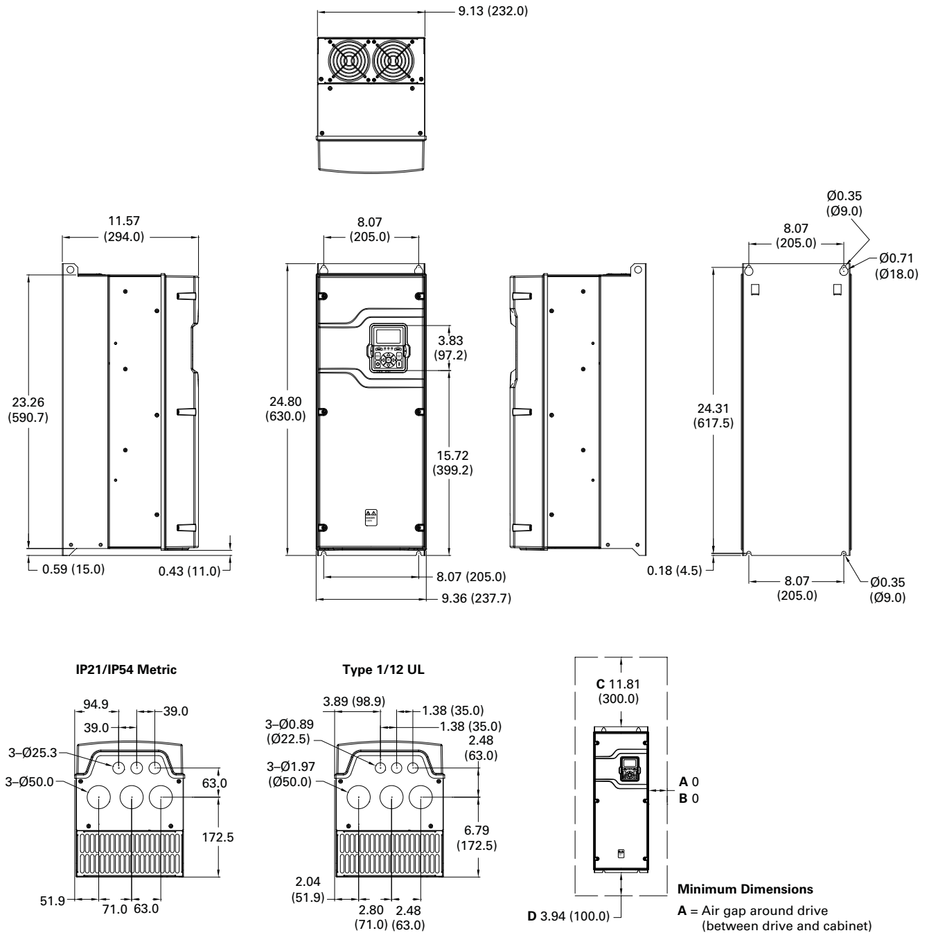
Figure 47. FR4 Dimension drawing
