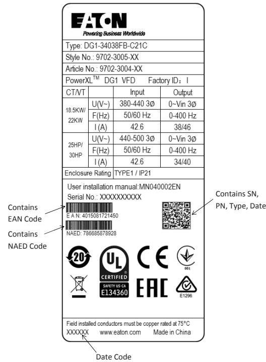
Figure 2. Rating label—DG1
