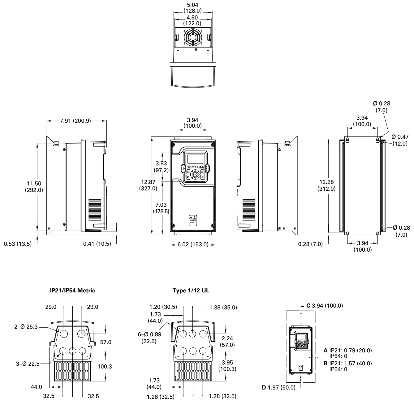
Figure 41. FR1 Dimension drawing
