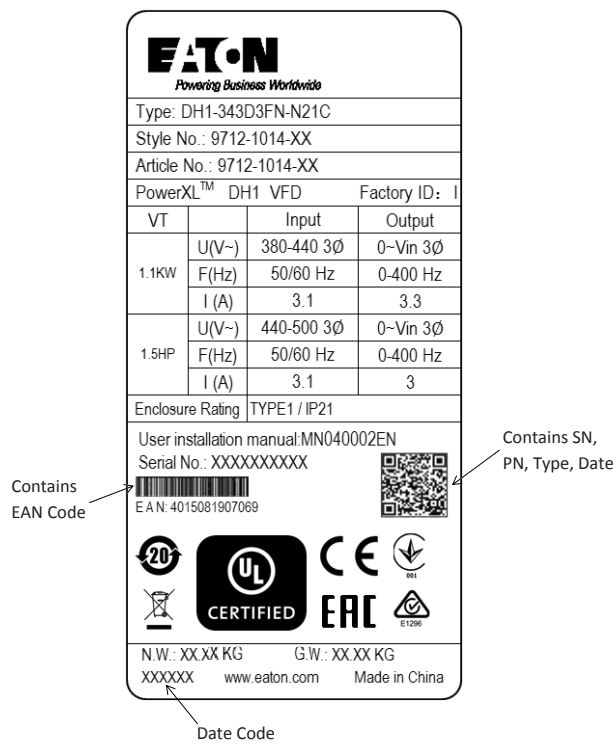
Figure 5. Carton label—DH1
