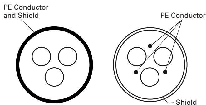
Figure 35. Cable description
