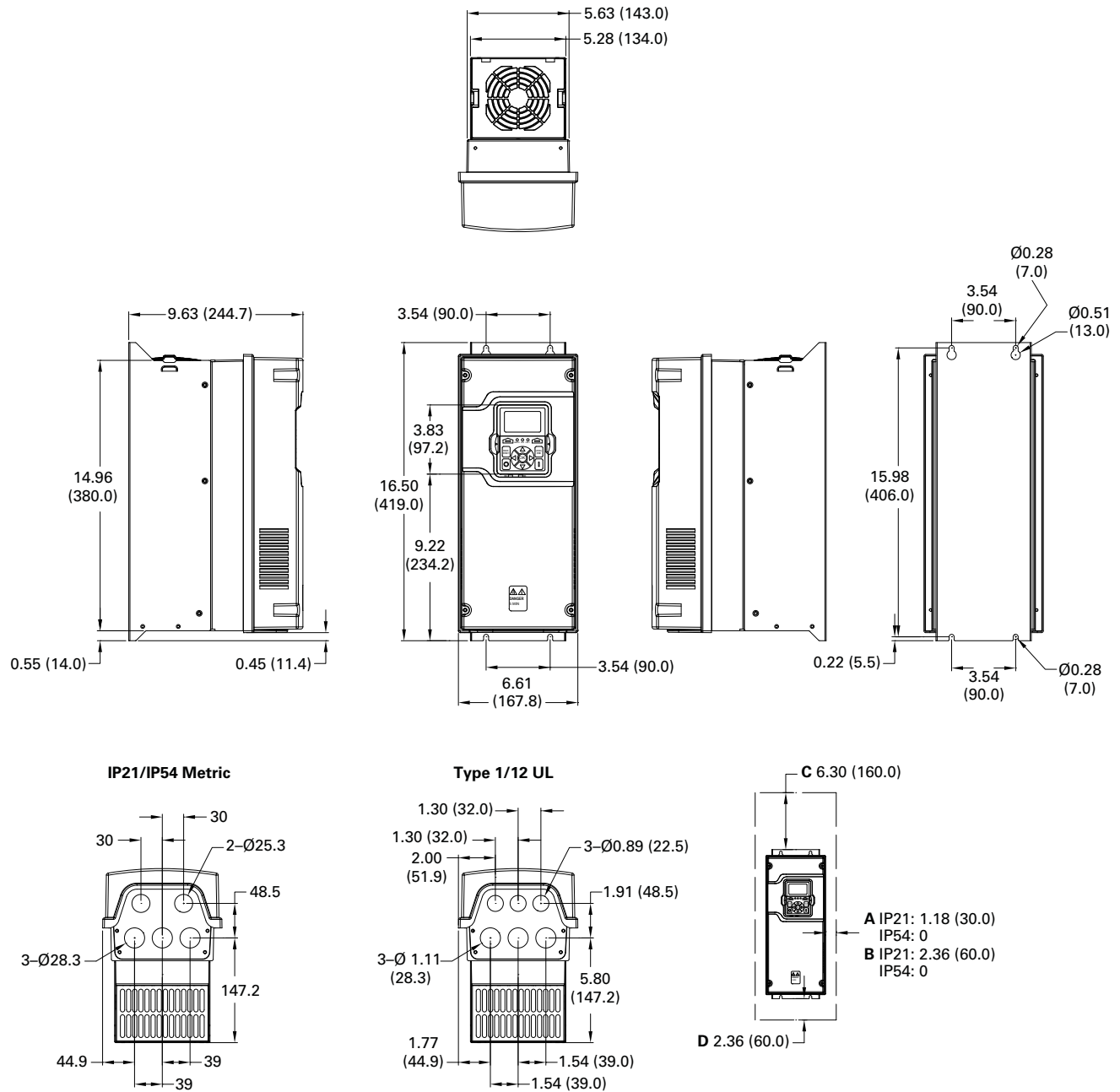
Figure 43. FR2 Dimension drawing
