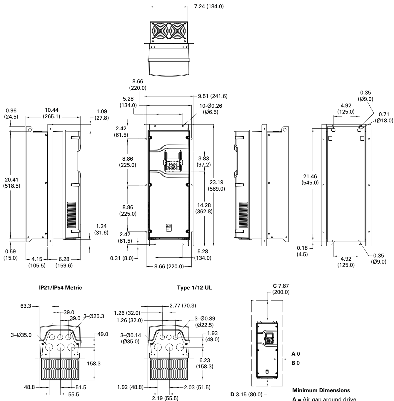
Figure 46. FR3 Dimension drawing flange mount
