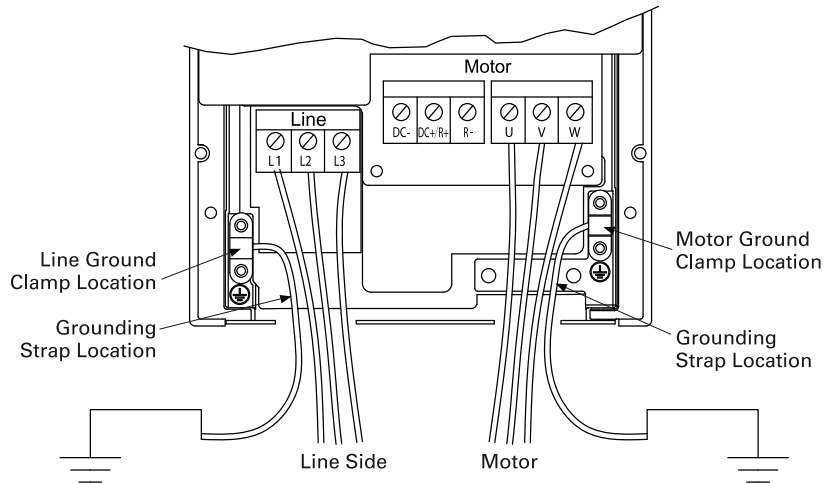
Figure 24. Ground wiring
