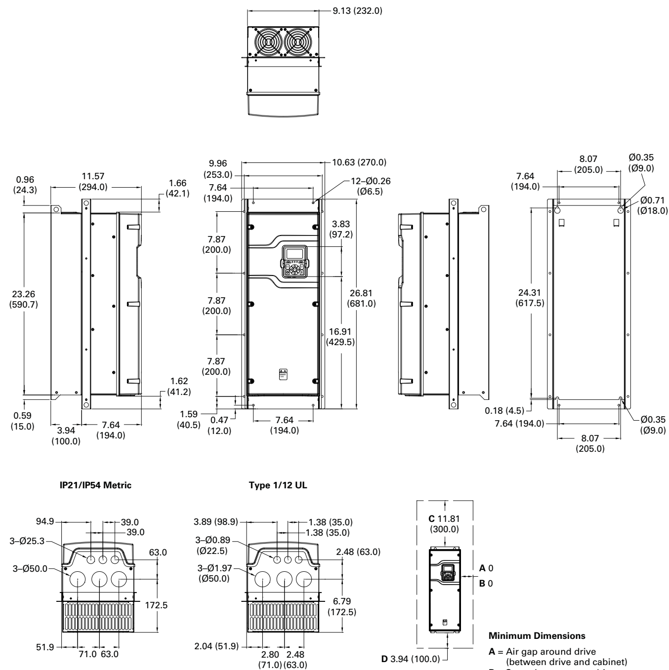
Figure 48. FR4 Dimension drawing flange mount
