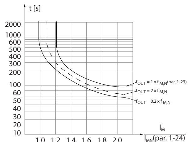
Illustration 2.18 ETR Characteristics
