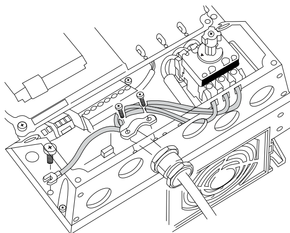
Illustration 8.3 Mains and Grounding with Disconnecter (for S2 variants in enclosure size B2, the extra terminal block must be used for mains connection).
