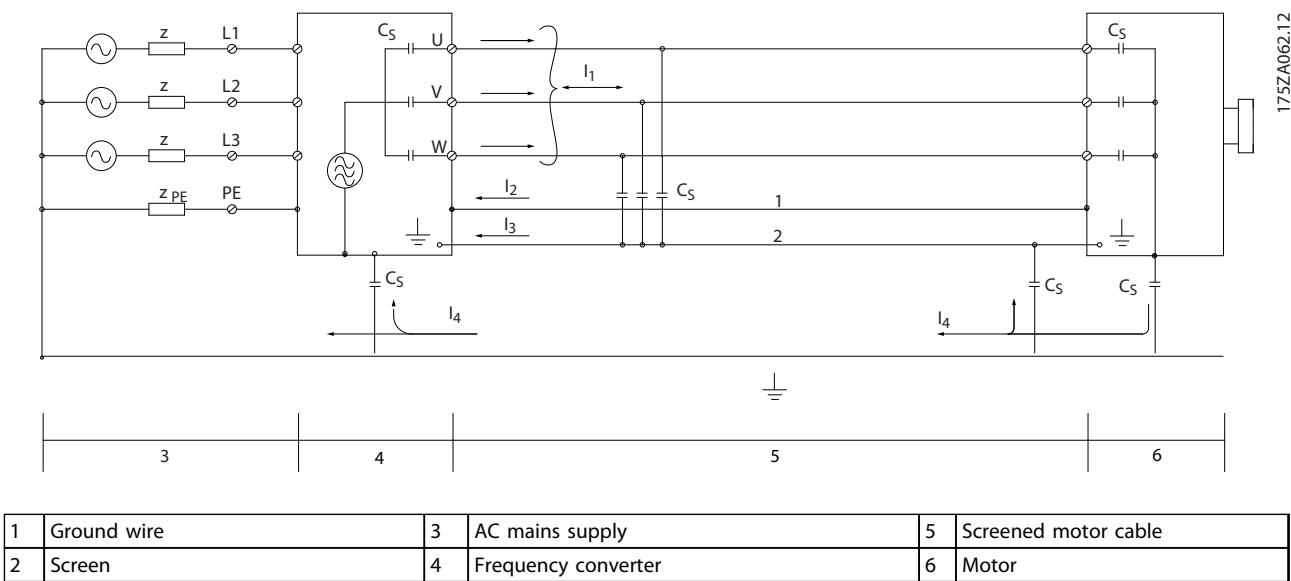
Illustration 3.2 Generation of Leakage Currents
