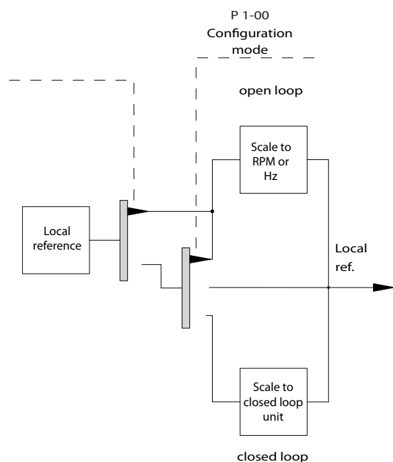
Illustration 2.14 Configuration Mode
