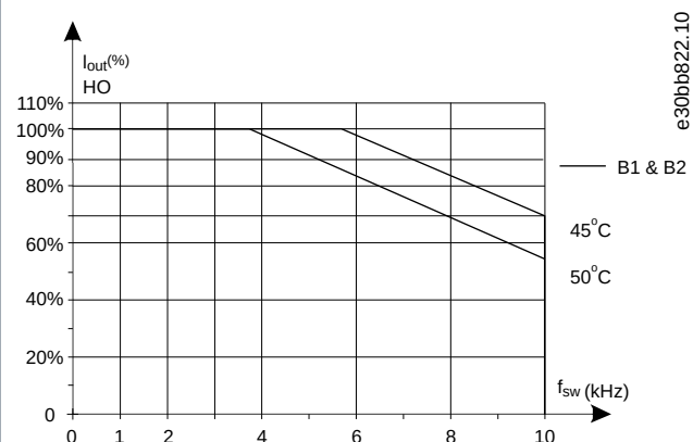
Illustration 74: Output Current Derating with Switching Frequency and Ambient Temperature for 600 V drives, for Enclosure Size B, using 60° AVM
