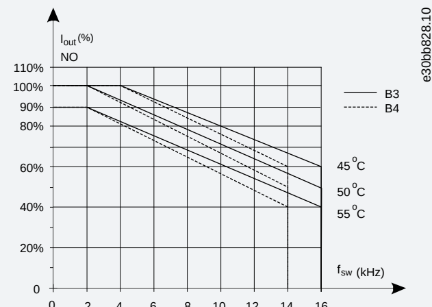
Illustration 69: Derating of I_{out} for Different T_{amb,max} for Enclosure Sizes B3 and B4, using 60° AVM
