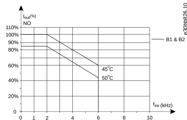
Illustration 77: Output Current Derating with Switching Frequency and Ambient Temperature for 600 V Drives, Enclosure Size B; SFAVM
