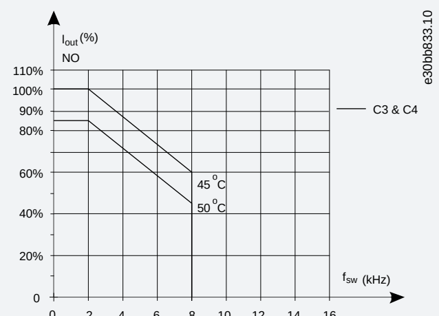
Illustration 87: Derating of I_{out} for Different T_{amb,max} for Enclosure Sizes C3 and C4, using SFAVM
