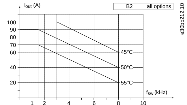
Illustration 79: Output Current Derating with Switching Frequency and Ambient Temperature for Enclosure Sizes B2 and B4, using SFAVM
