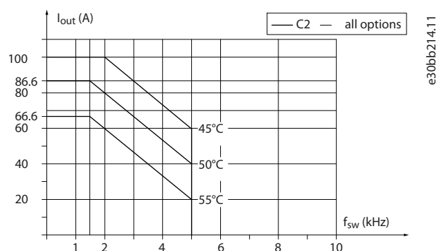
Illustration 93: Output Current Derating with Switching Frequency and Ambient Temperature for Enclosure Size C2, using SFAVM
