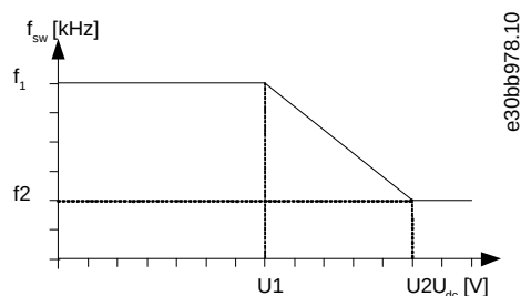
Illustration 31: Derating of switching frequency according to voltage on the DC link. f_1 , f_2 , U_1 , and U_2 are coded in EEPROM.
