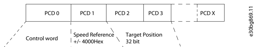
Illustration 16: Positioning: Default settings (PCD 1 = Fieldbus REF 1)
