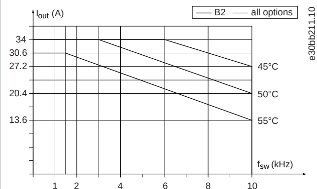
Illustration 78: Output Current Derating with Switching Frequency and Ambient Temperature for Enclosure Sizes B2 and B4, using 60° AVM
