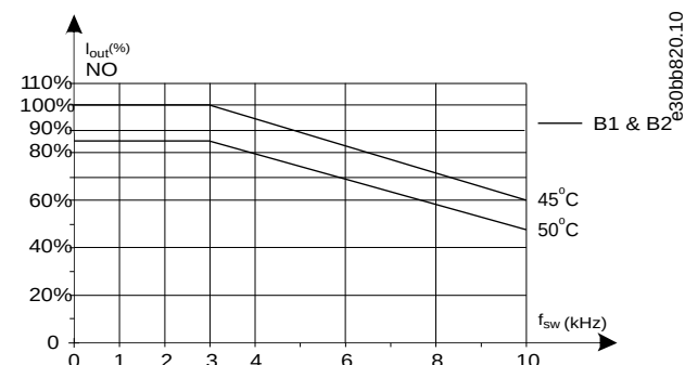
Illustration 75: Output Current Derating with Switching Frequency and Ambient Temperature for 600 V drives, for Enclosure Size B, using 60° AVM
