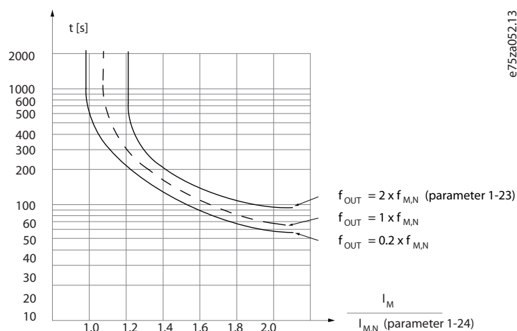
Illustration 35: ETR Characteristics
