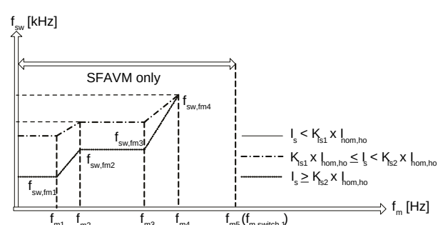
Illustration 33: Switching Frequency ( f_{sw} ) Variation for Different Stator Frequencies ( f_m )
