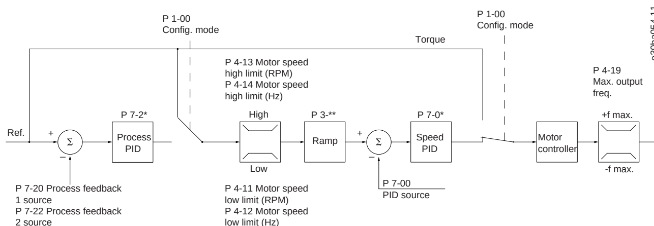
Illustration 151: Control Structure in Flux with Motor Feedback
