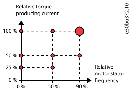
Illustration 7: Operating Point according to IEC 61800-9-2 (EN 50598)
