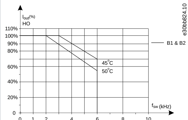
Illustration 76: Output Current Derating with Switching Frequency and Ambient Temperature for 600 V Drives, Enclosure Size B; SFAVM
