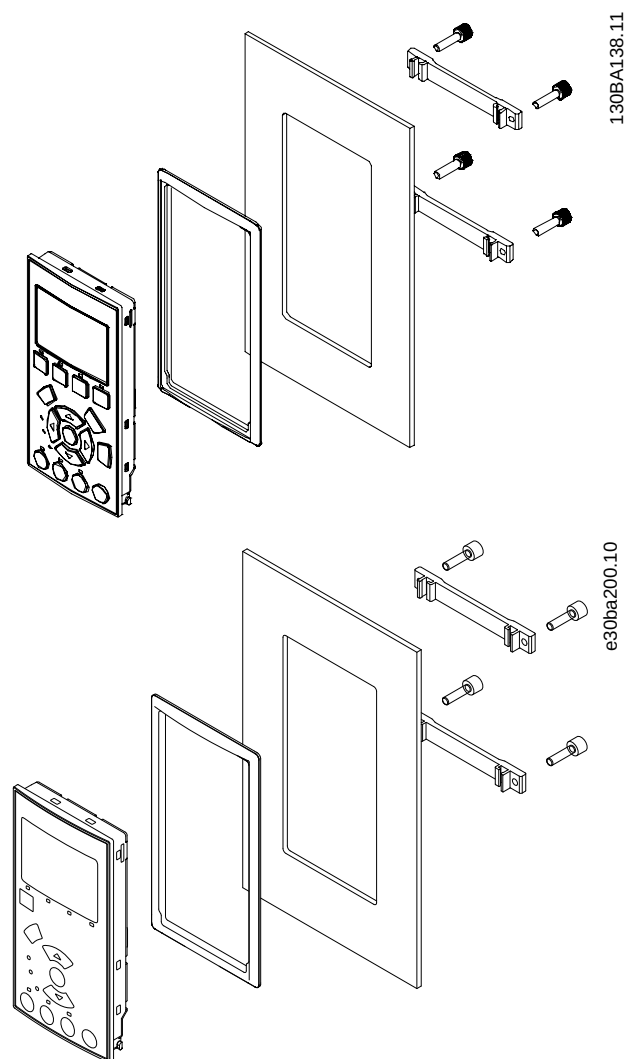
Illustration 49: Panel Mounting Kit for LCP 102, LCP 101, and LCP 103
