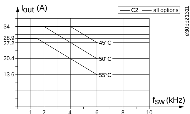
Illustration 92: Output Current Derating with Switching Frequency and Ambient Temperature for Enclosure Size C2, using 60° AVM
