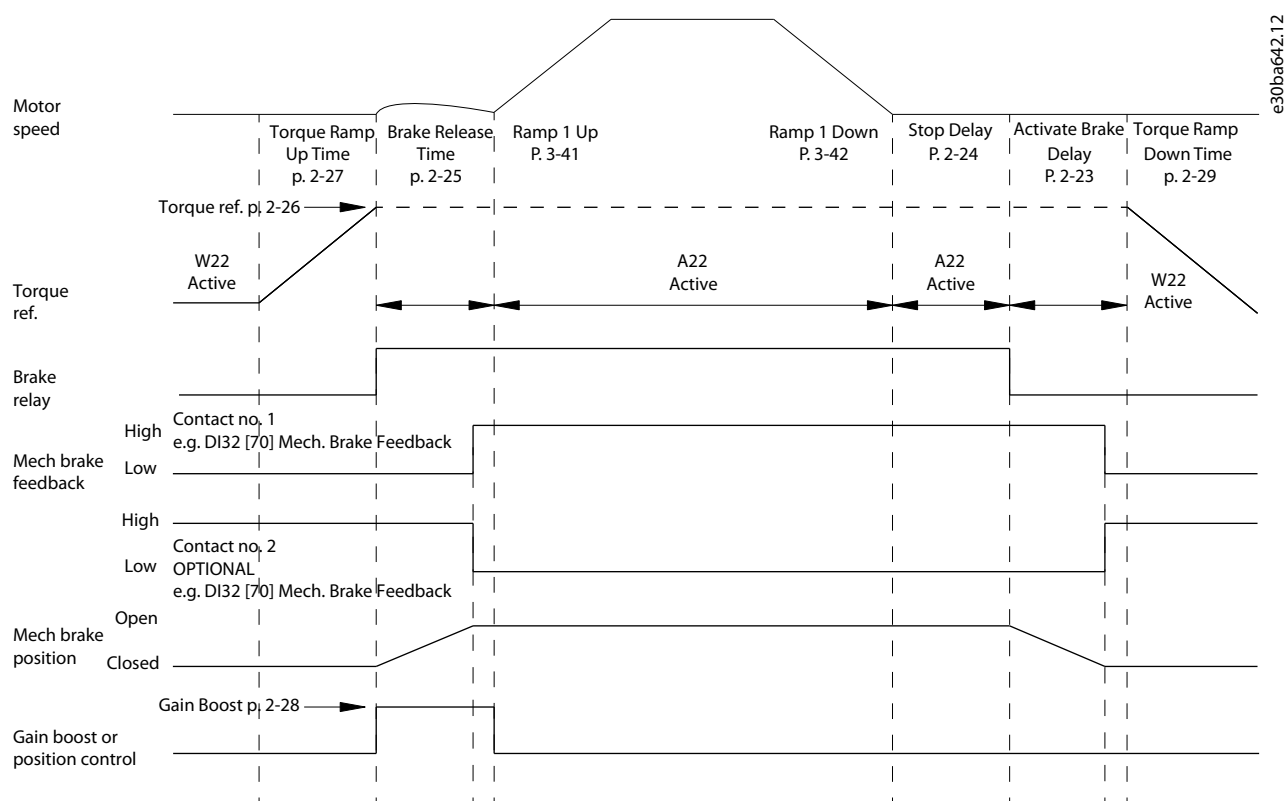
Illustration 42: Brake Release Sequence for Hoist Mechanical Brake Control
