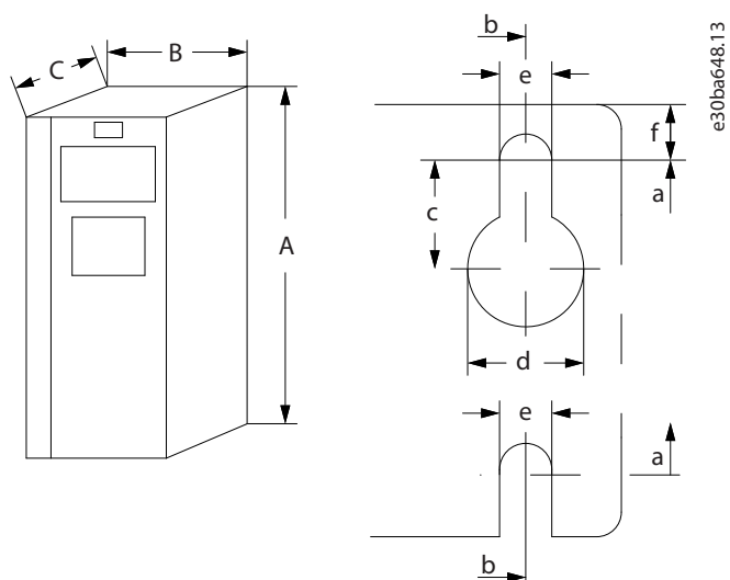
Illustration 53: Top and Bottom Mounting Holes
