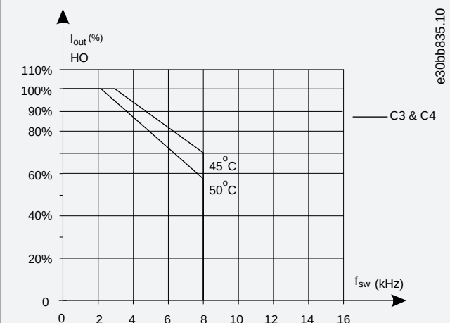
Illustration 86: Derating of I_{out} for Different T_{amb,max} for Enclosure Sizes C3 and C4, using SFAVM
