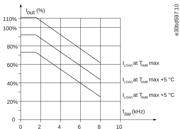
Illustration 94: Output Current Derating with Switching Frequency and Ambient Temperature for Enclosure Size C3
