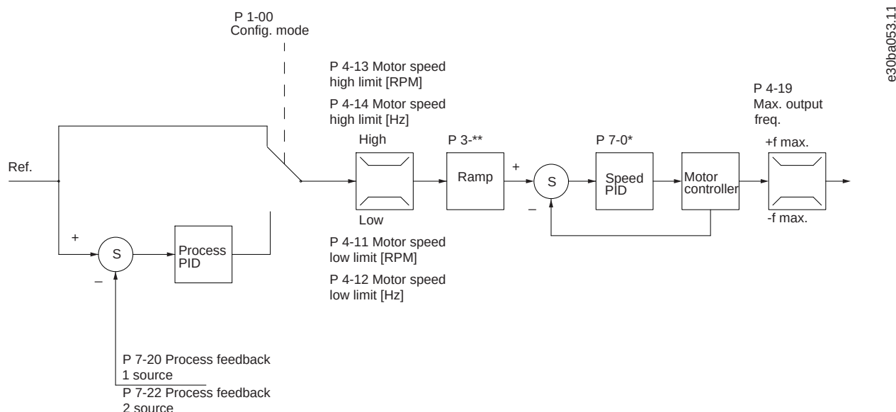
Illustration 150: Control Structure in Flux Sensorless
