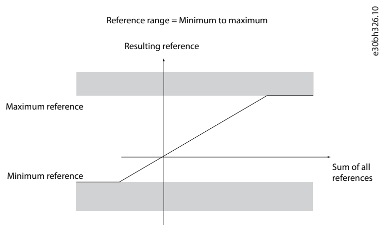
Illustration 145: Sum of all References when Configuration Mode is set to Process
