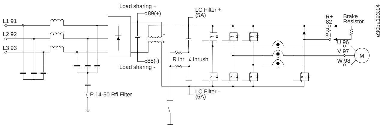
Illustration 148: Control Principle, FC 302
