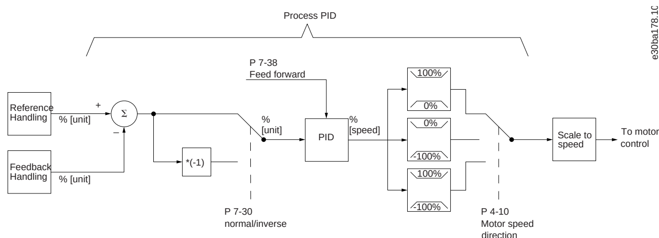
Illustration 146: Process PID Control Diagram
