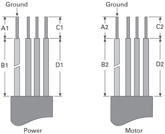
Figure 19. Input power and motor cable stripping lengths
