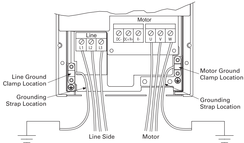
Figure 20. Ground wiring
