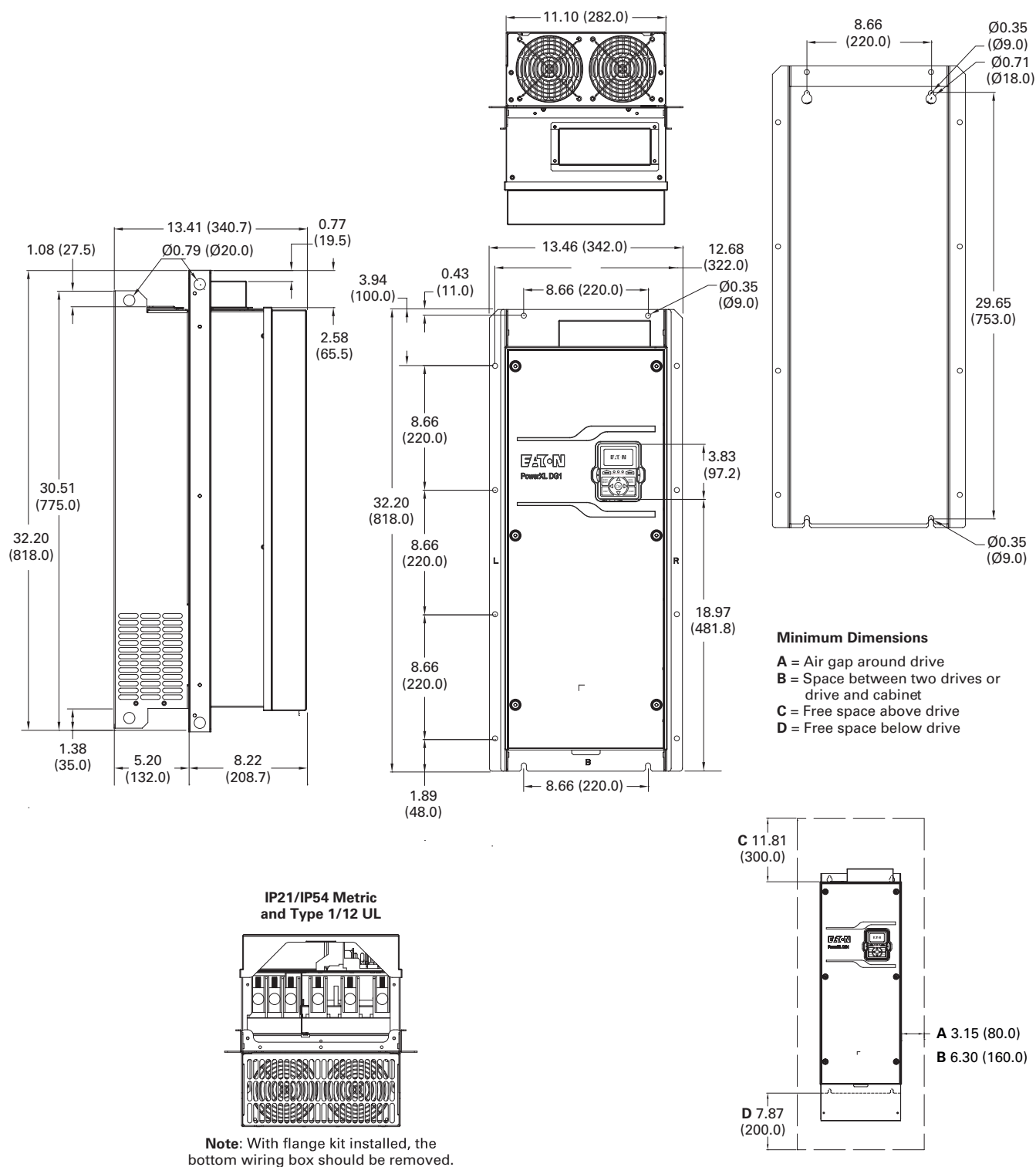
Figure 44. FR5 Dimension drawing flange mount
