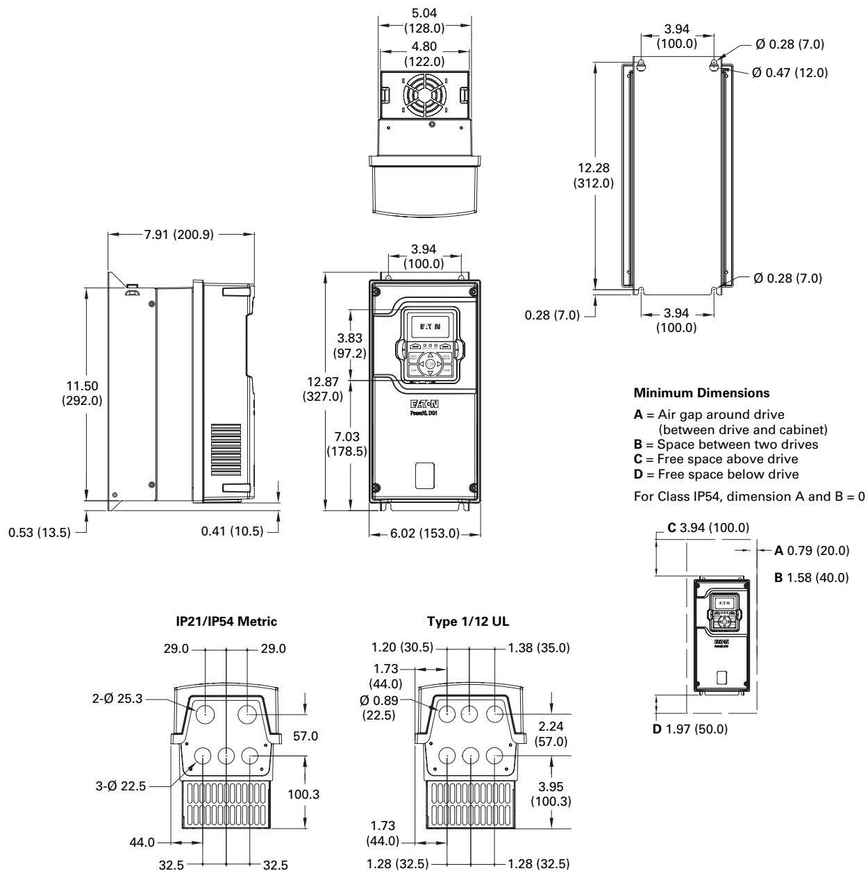
Figure 35. FR1 Dimension drawing
