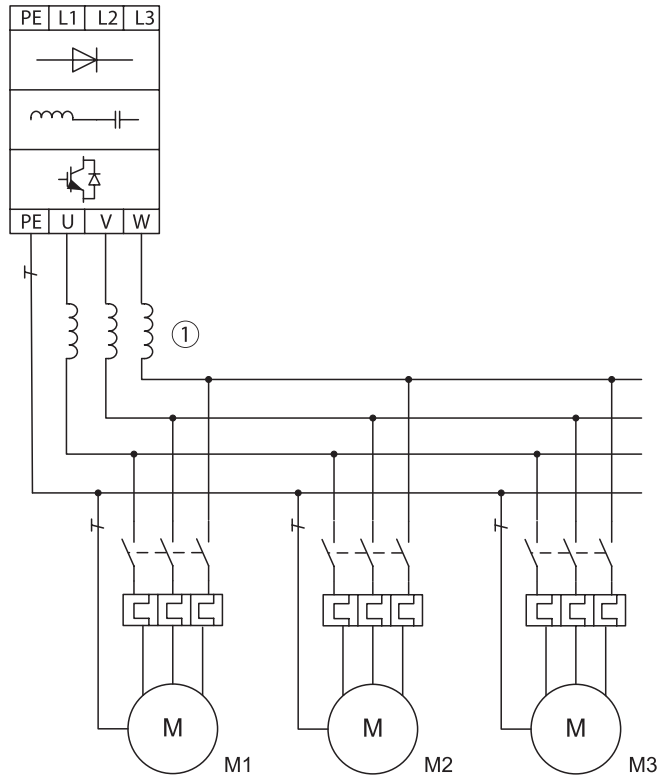
Figure 11. Parallel connection
