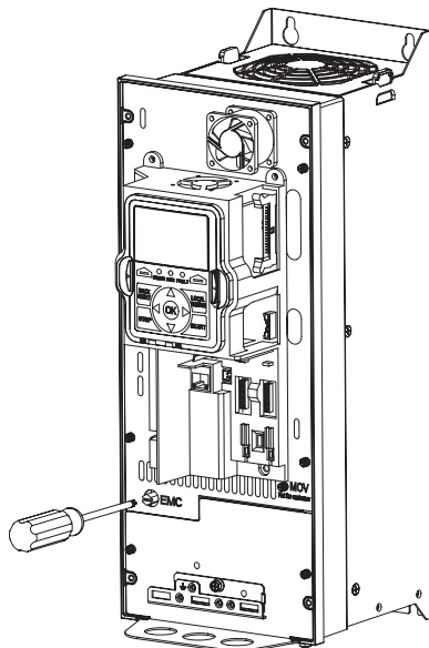
Figure 32. Locations of the EMC Screw in Frame 1 and Frame 3
