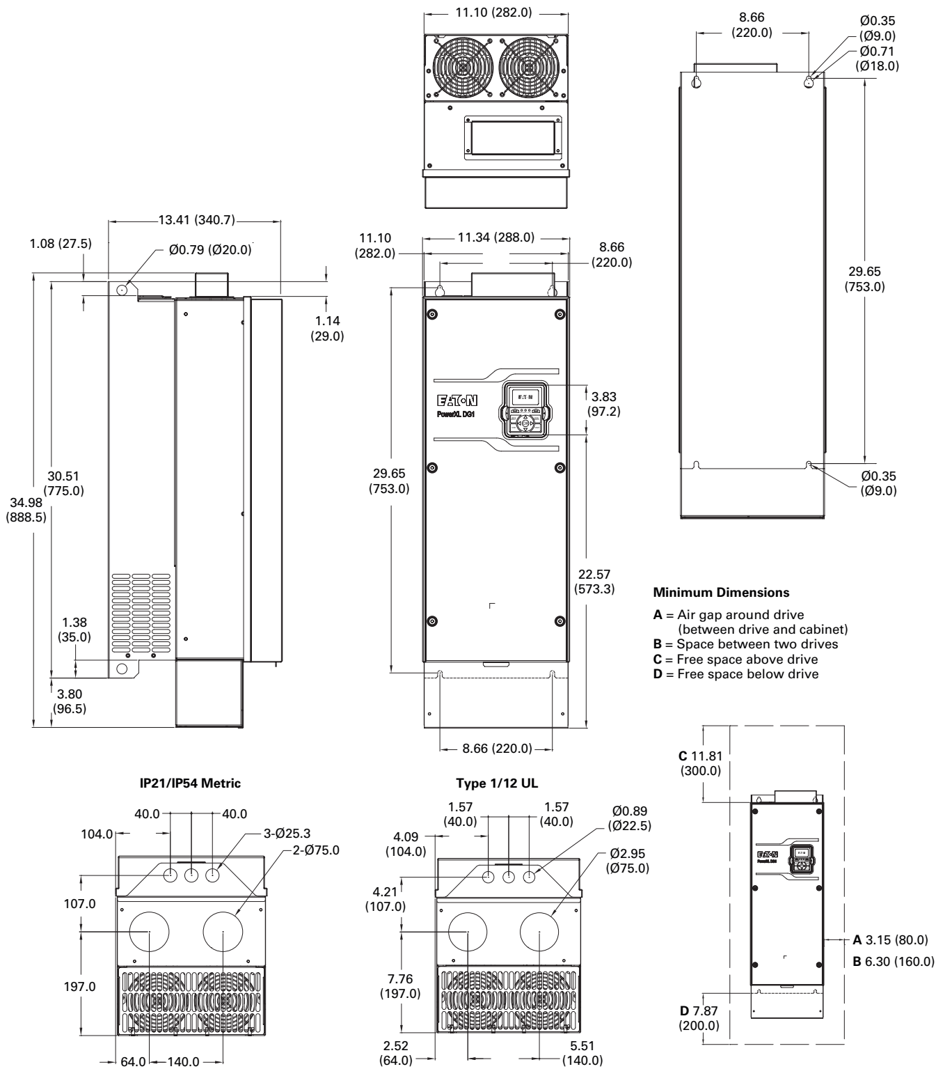
Figure 43. FR5 Dimension drawing
