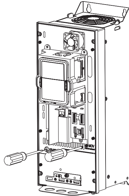
Figure 34. Locations of the EMC Screws in Frame 5 and Frame 6
