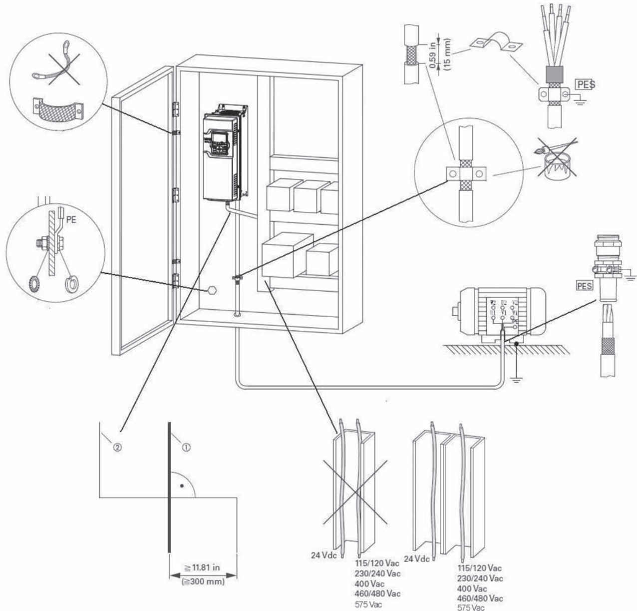
Figure 30. EMC-Compliant Setup—230 Vac, 460/480 Vac, 600 Vac
