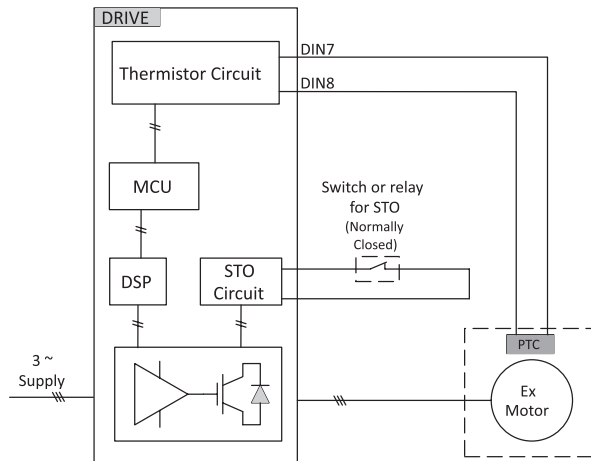
Figure 24. Thermistor/STO wiring diagram
