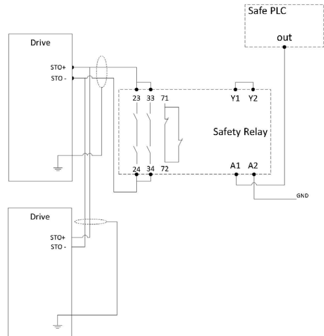
Figure 26. Example of Wiring a STO with the internal 24V supply to multiple drives.
