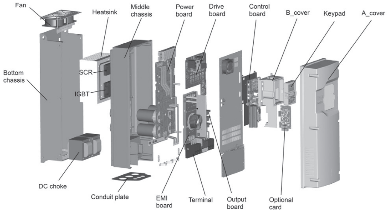
Figure 6. Description of the DG1 series
