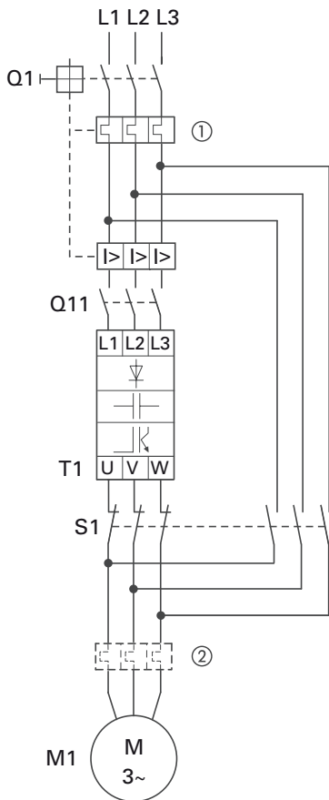
Figure 15. Bypass motor control (example)
