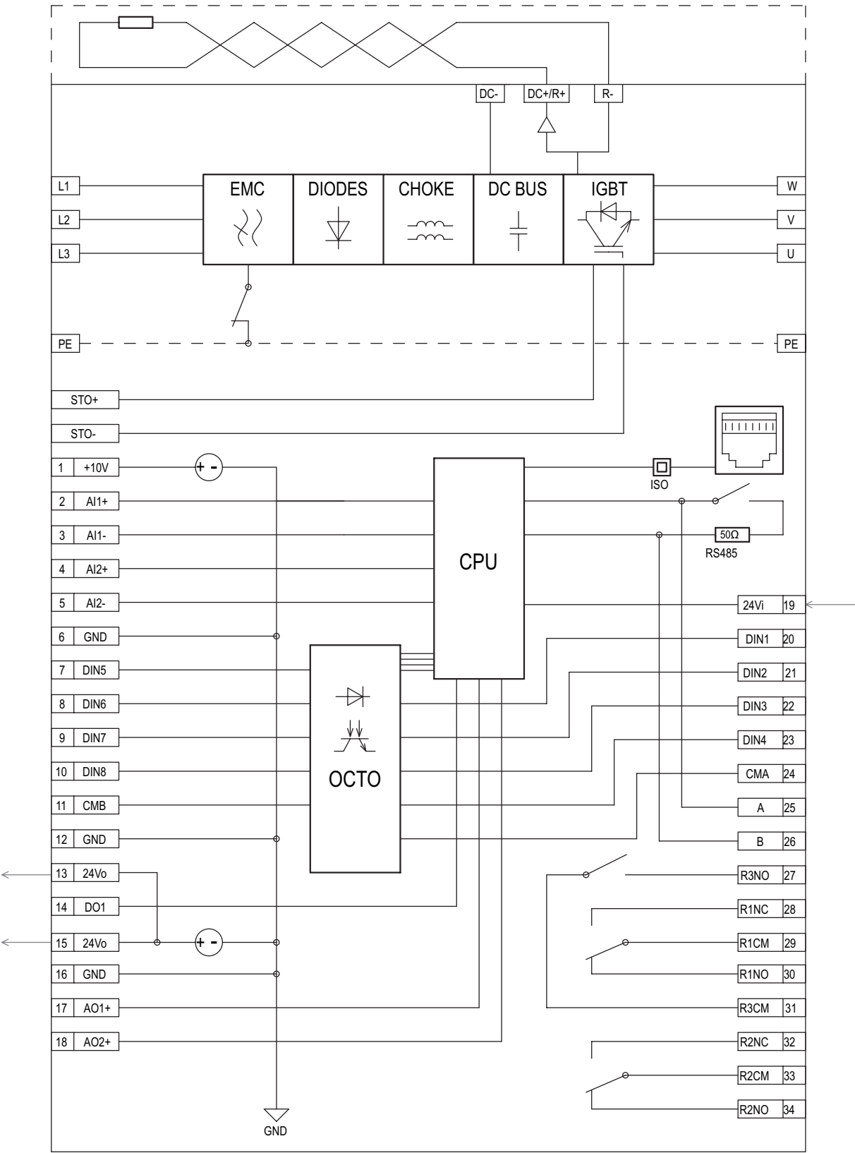
Figure 22. Basic internal control wiring diagram
