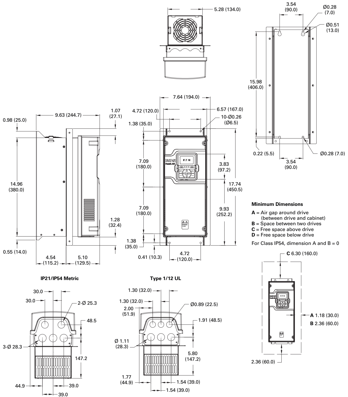
Figure 38. FR2 Dimension drawing flange mount
