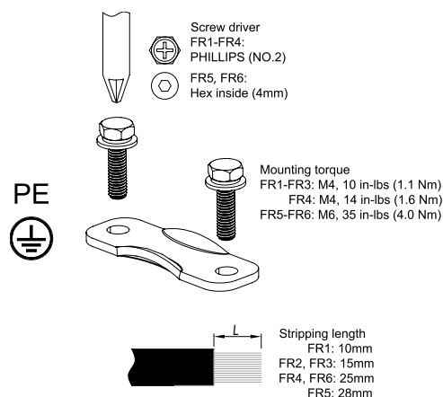
Figure 28. Grounding
