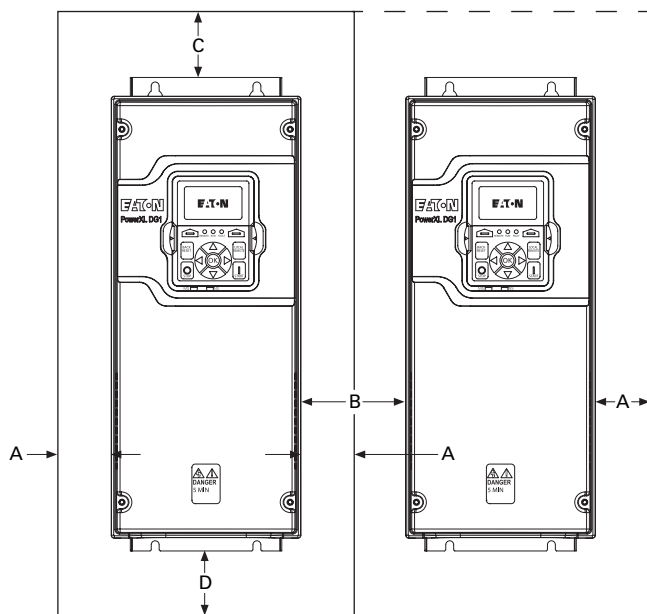
Figure 16. Mounting space
