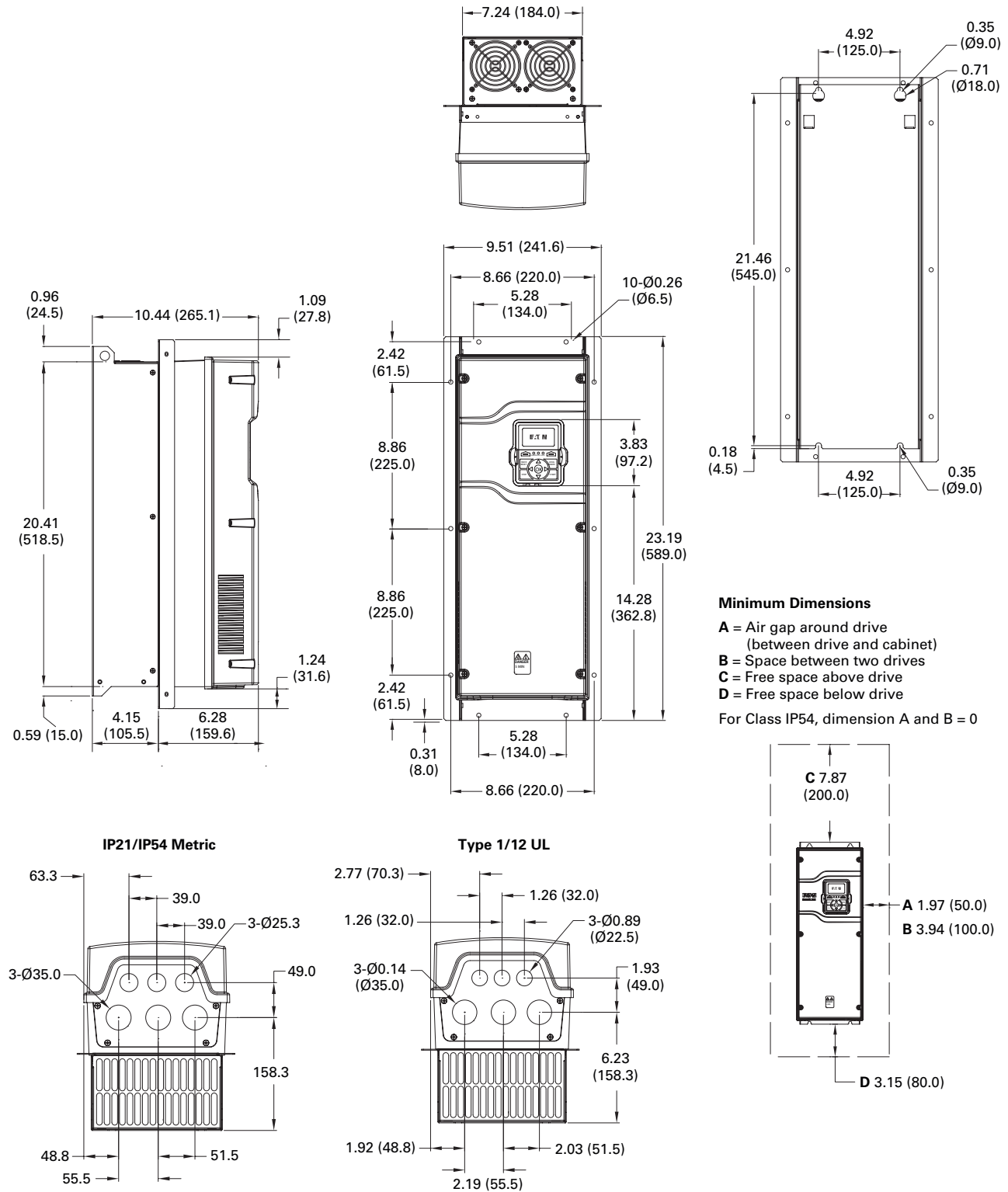
Figure 40. FR3 Dimension drawing flange mount
