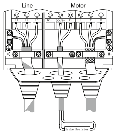
Figure 18. Brake resistor wiring
