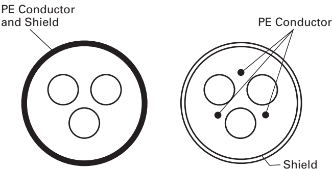
Figure 31. Cable description
