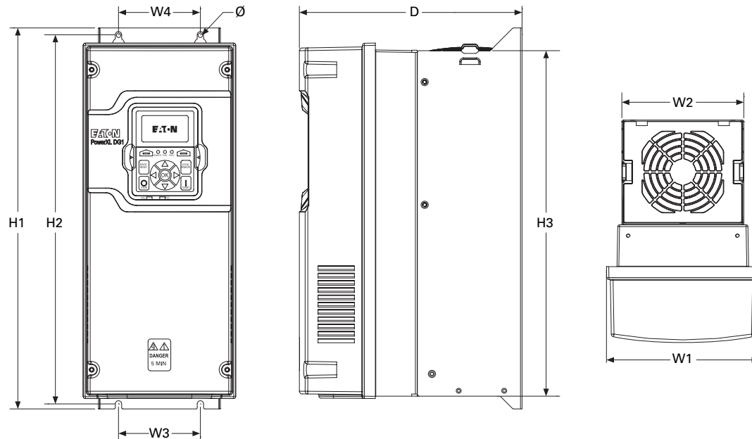
Figure 17. Type 1/12 open drives
