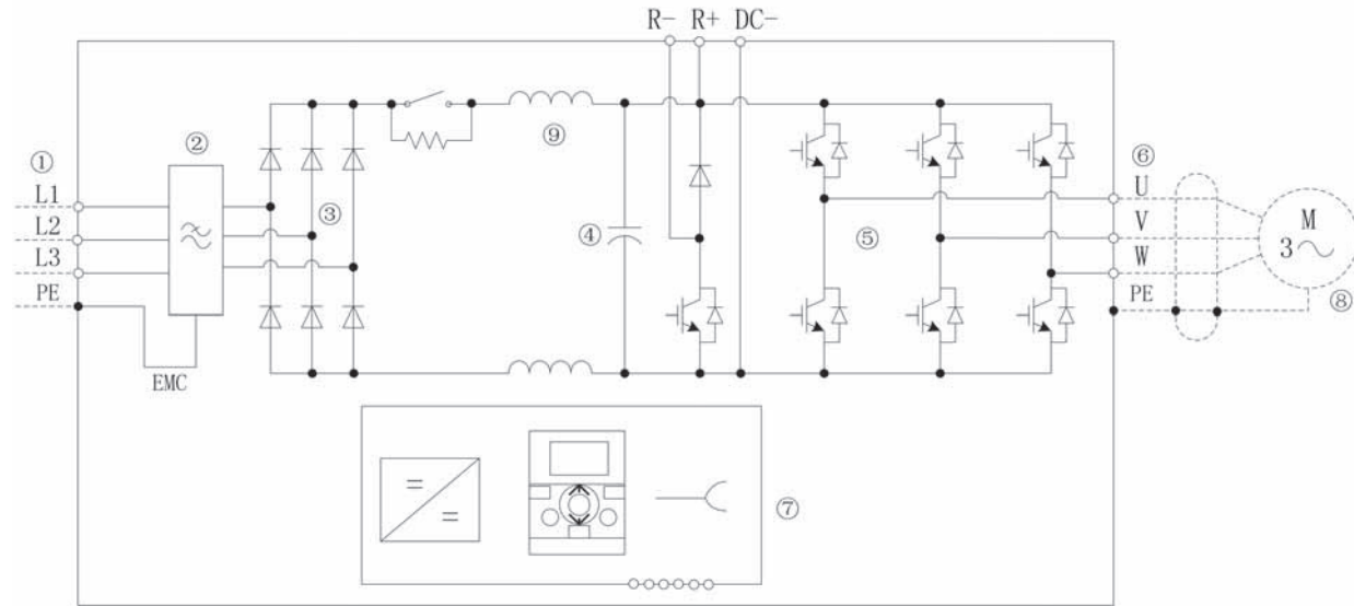
Figure 7. Block diagram, elements of DG1 frequency inverters
