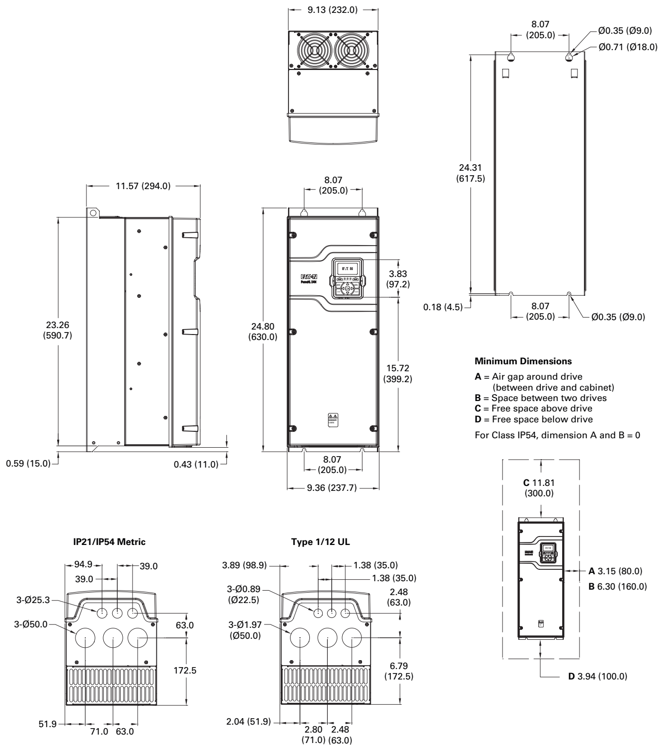
Figure 41. FR4 Dimension drawing
