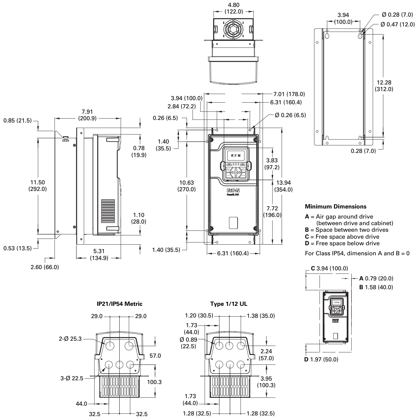
Figure 36. FR1 Dimension drawing flange mount
