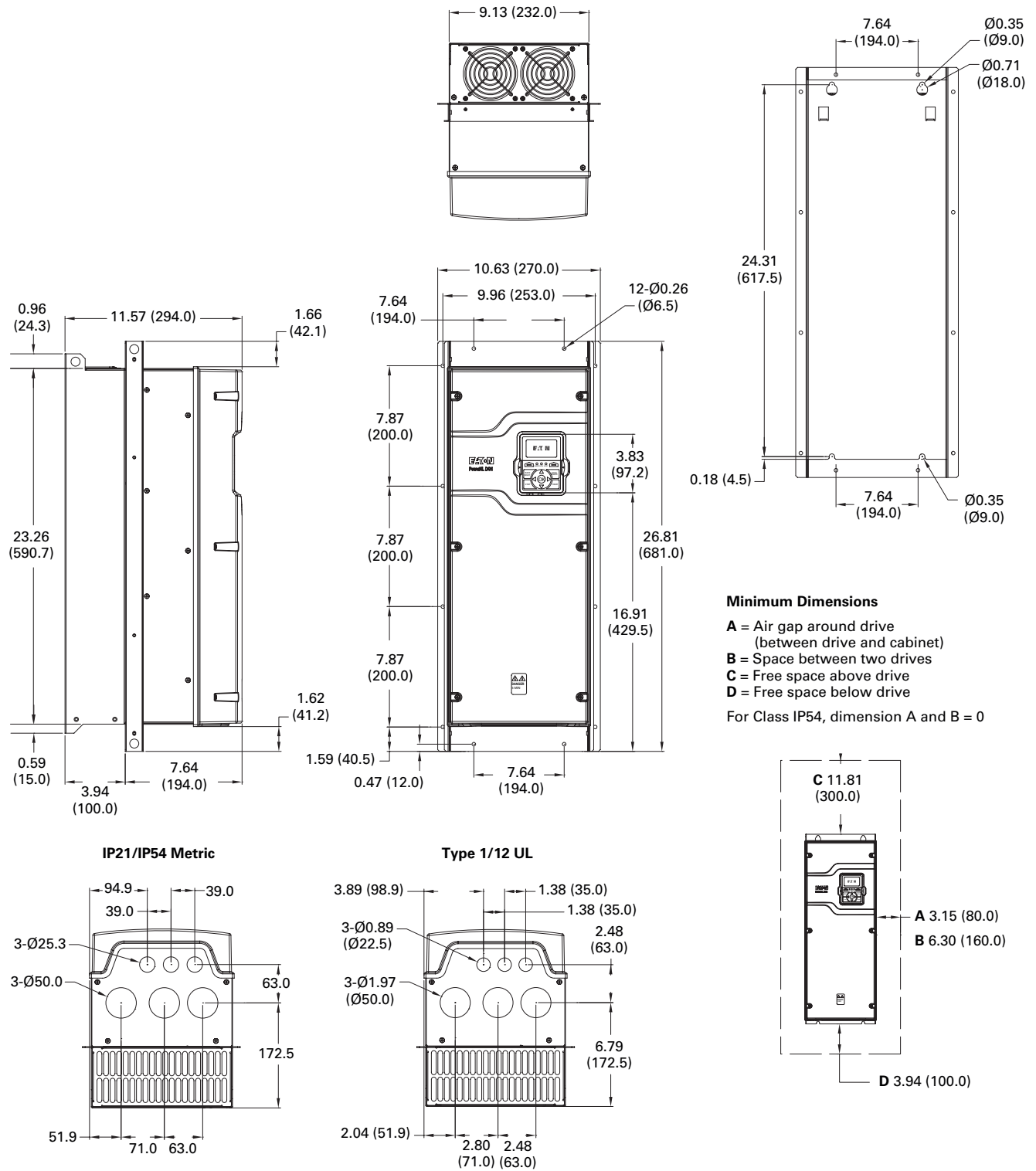
Figure 42. FR4 Dimension drawing flange mount
