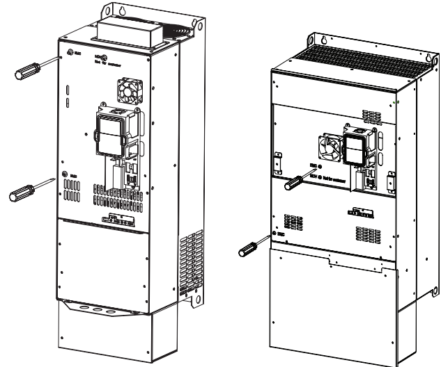
Figure 34. Locations of the EMC Screws in Frame 5 and Frame 6
