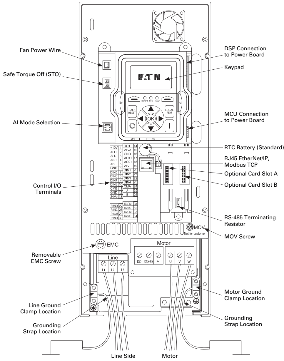
Figure 23. DG1 series adjustable frequency drive
