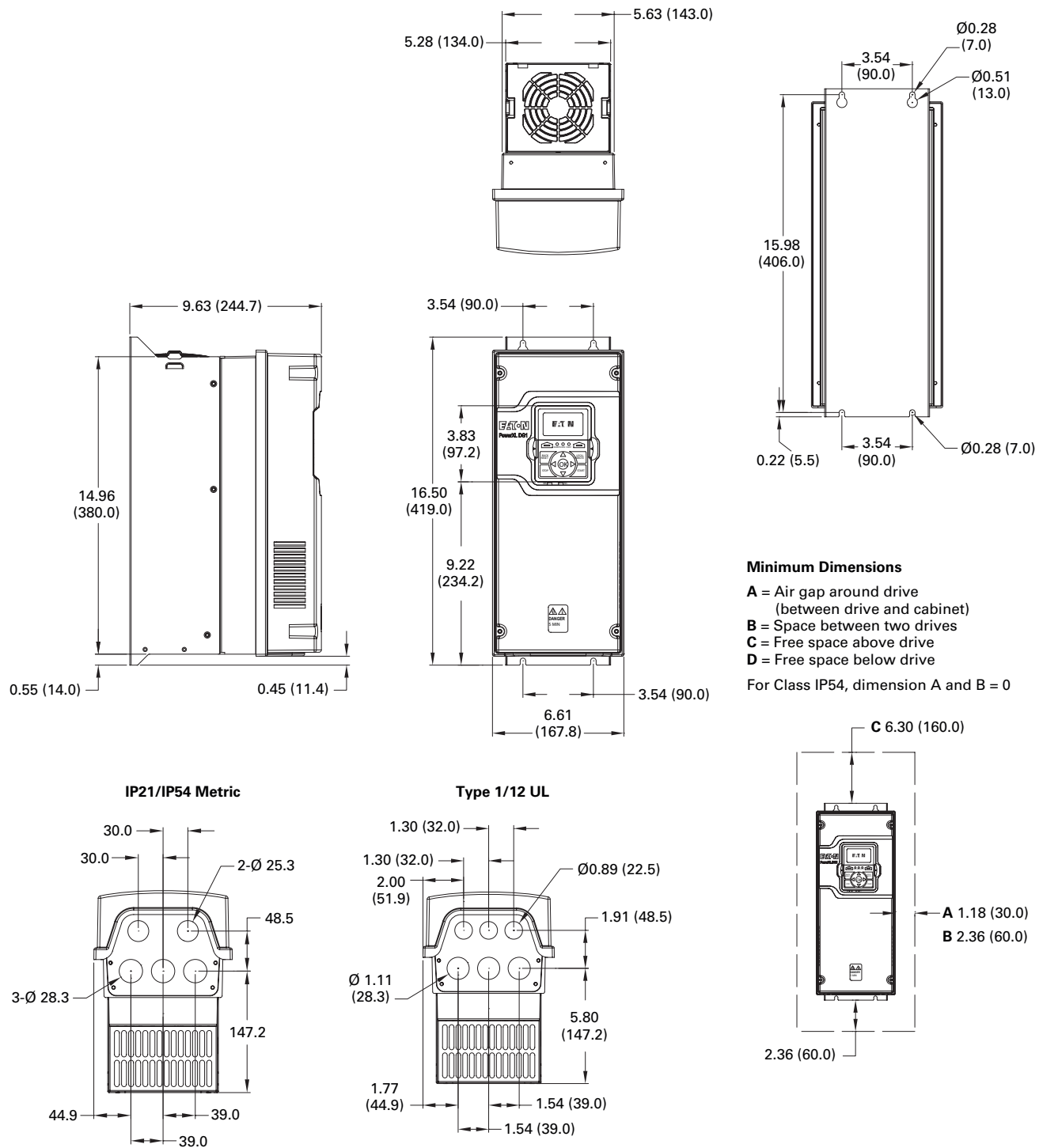
Figure 37. FR2 Dimension drawing
