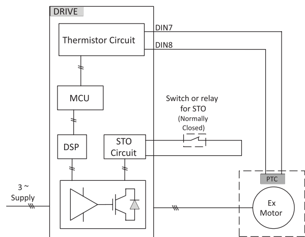
Figure 49. Thermistor STO wiring diagram
