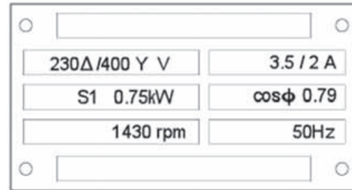
Figure 12. Example of a motor ratings plate
