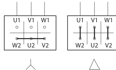
Figure 13. Star and delta circuit types
