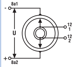
Sealed winding with 2 opposite tappings and 2 opposite wipers continuous rotation
