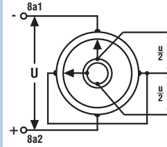
Sealed sin/cos functional windings with 90° offset wipers
