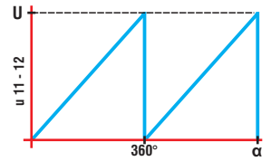
Wiper continuous rotation, without reactive winding, only at beginning and end led out separately
