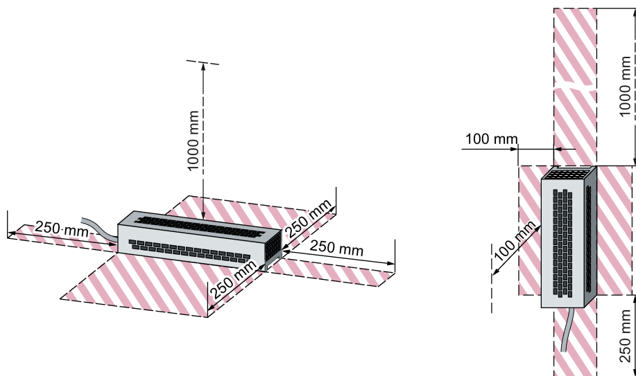
Figure 8-3 Minimum clearances for the braking resistor when mounting on a flat surface and for wall/panel mounting
