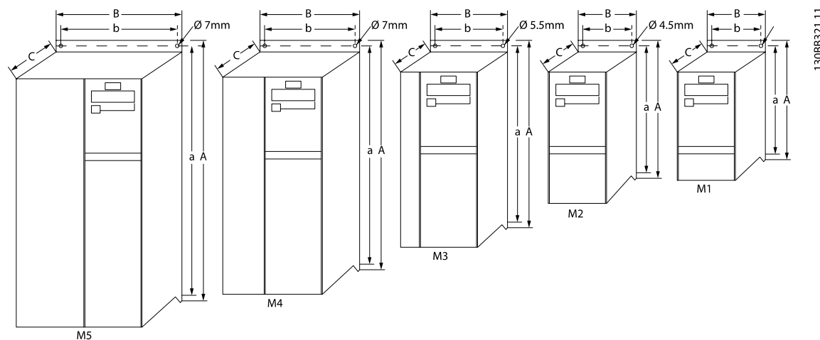
Illustration 1.1: Mechanical dimensions.
