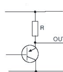
Status output circuit
