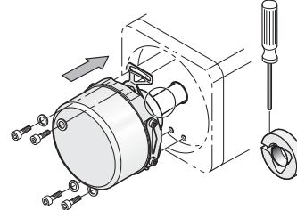
ECN/EQN/ERN 400 e.g. with standard stator coupling
