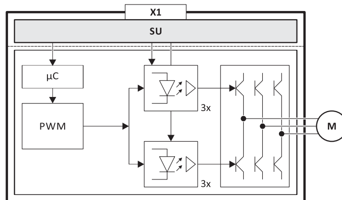
Fig. 1: Operating principle of safety unit
