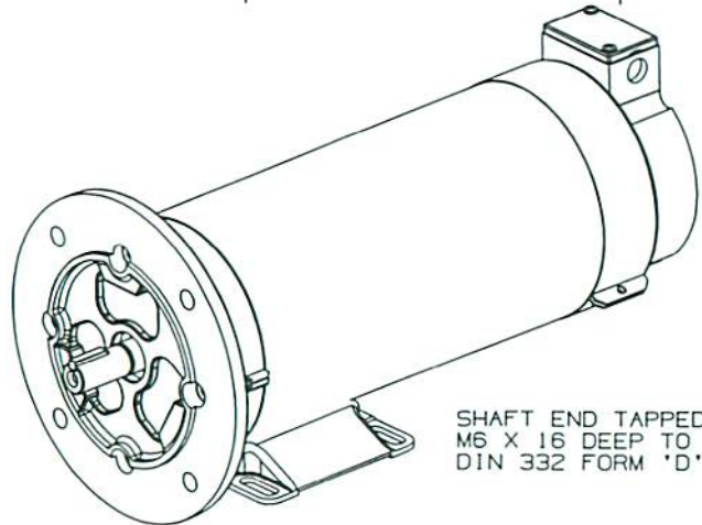
SHAFT END DETAILS
