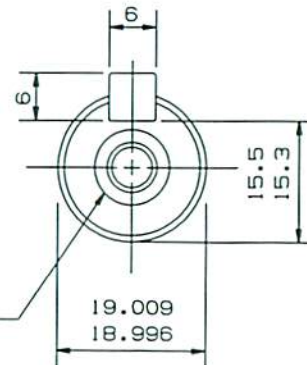
SHAFT END DETAILS
