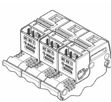
3 auxiliary microswitches 3 x CMS22W1
