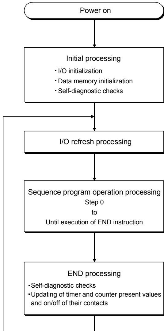
Fig 3.1 Operation Processings of Built-in PLC function
