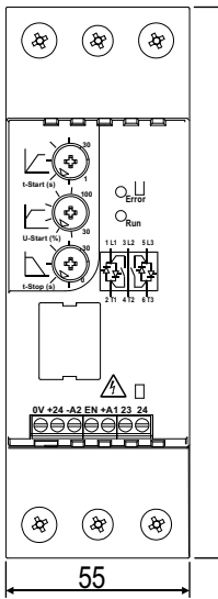
Mounting Centres 40mm x 155mm
