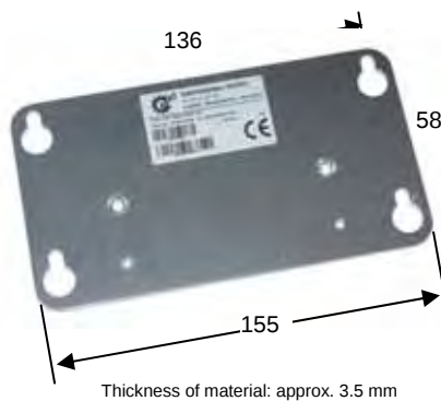
Fig.: SK TIE4-WMK-TU wall-mounting kit
