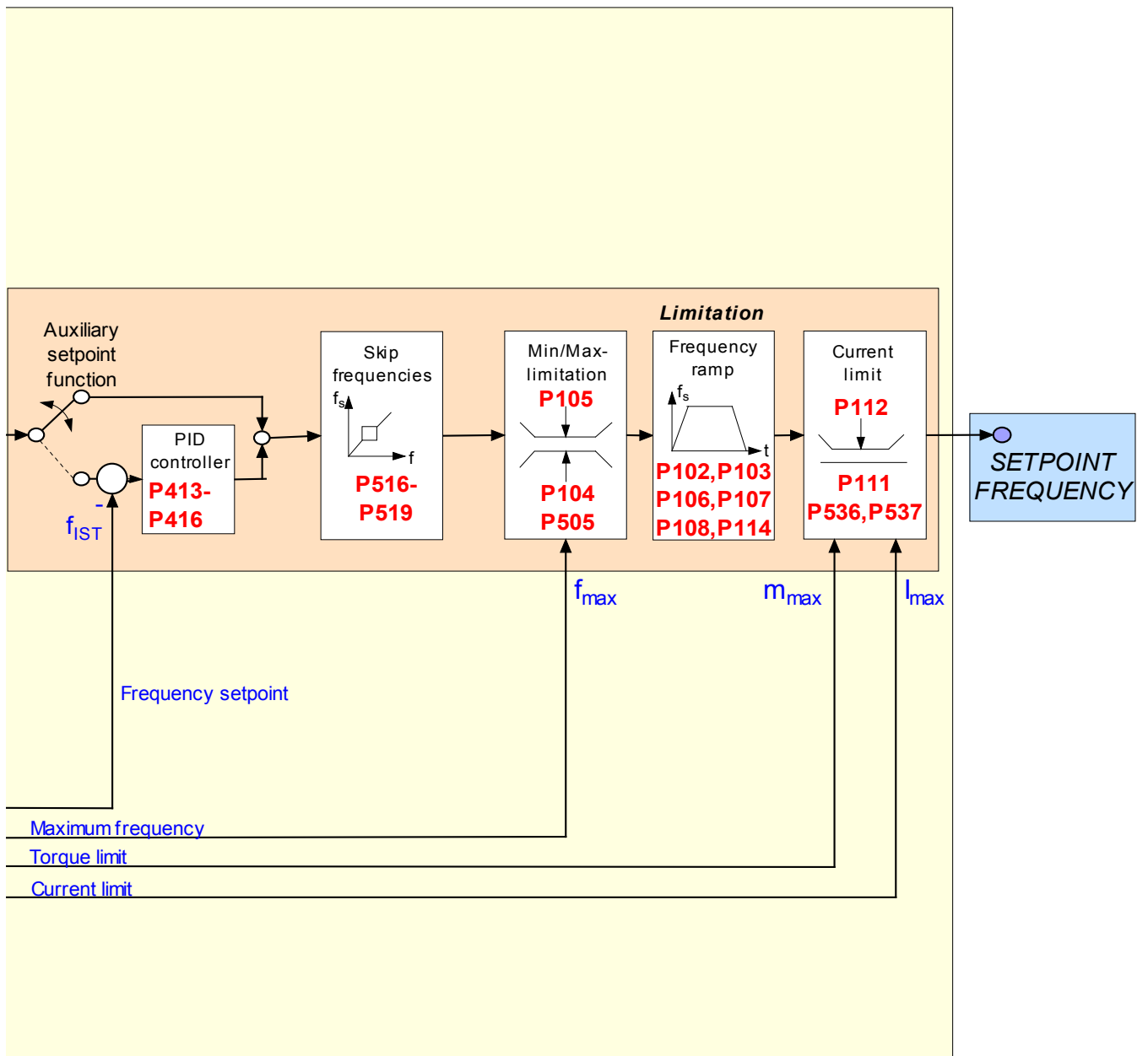
Fig. 14: Setpoint processing
