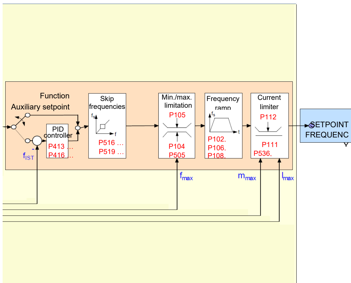
Illustration 7: Setpoint processing
