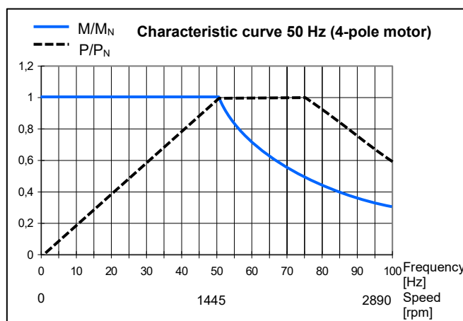
Illustration 14: Characteristic curve 50 Hz
