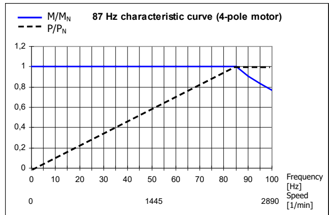
Figure 15: 87 Hz characteristic curve
