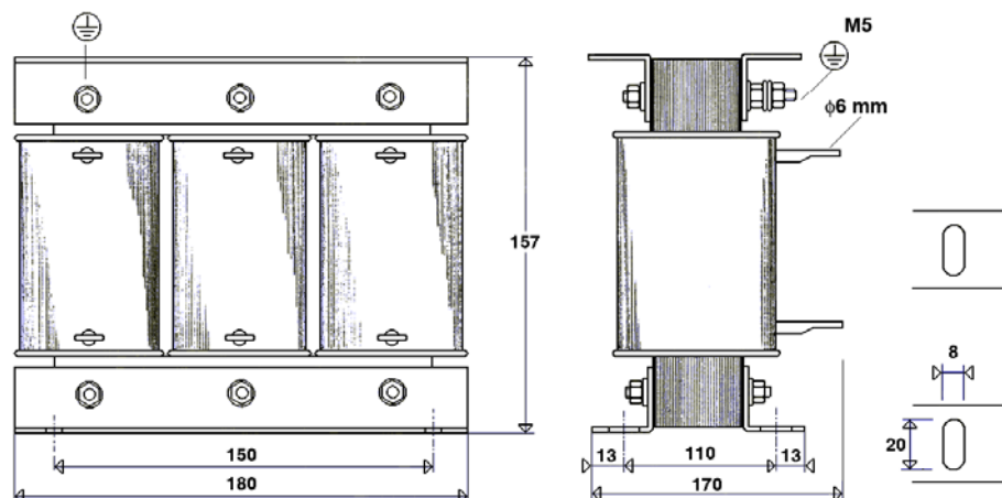
Dimensional drawing: LCG-0055-0.45 mH
