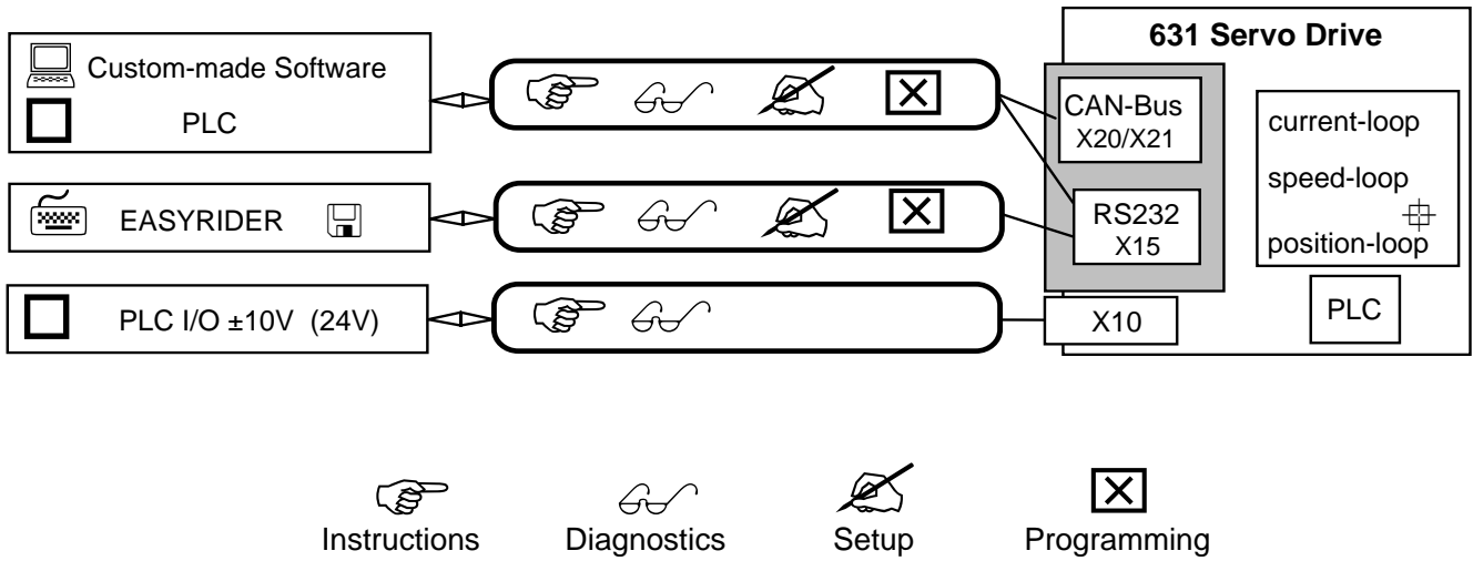
Figure 2-2 Communications Options
