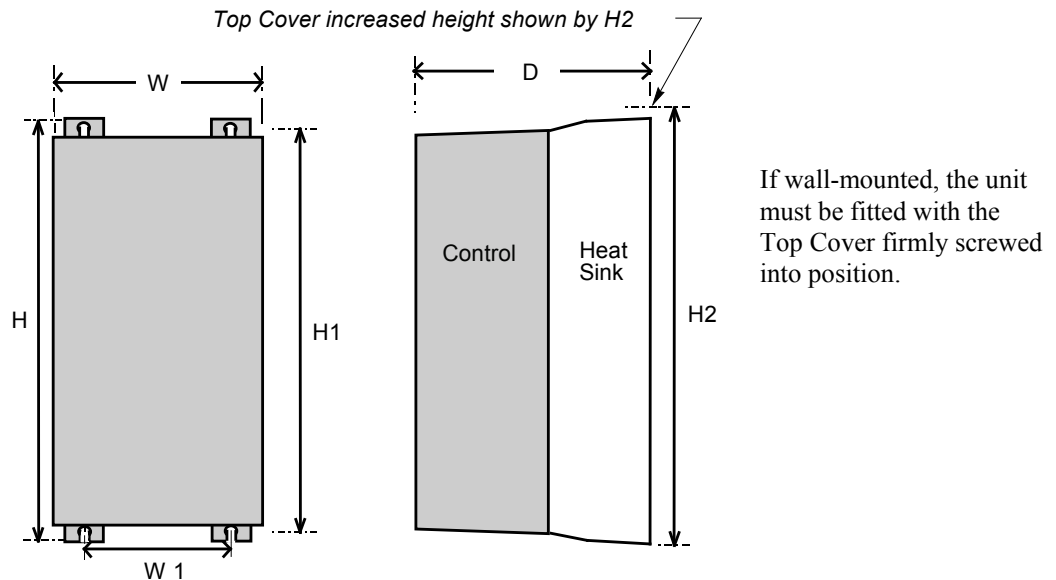
Figure Chapter 3 -1 Mechanical Dimensions for 650V Drives
