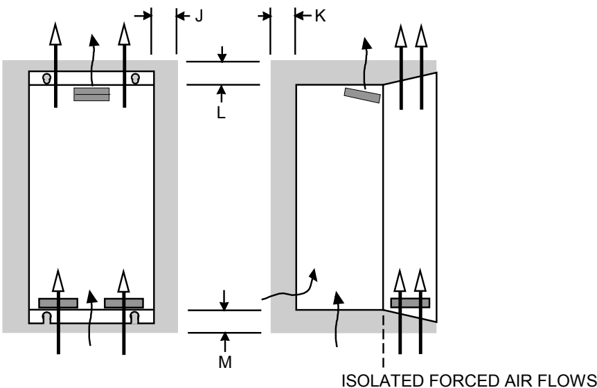
Figure Chapter 3 -5 Air Clearance for a Cubicle-Mount Product/Application
