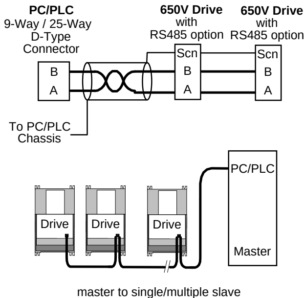
master to single/multiple slave RS485 Connections
