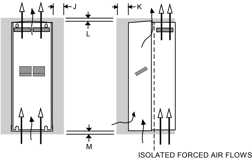
Figure Chapter 3 -8 Air Clearance for a Cubicle-Mount Product/Application
