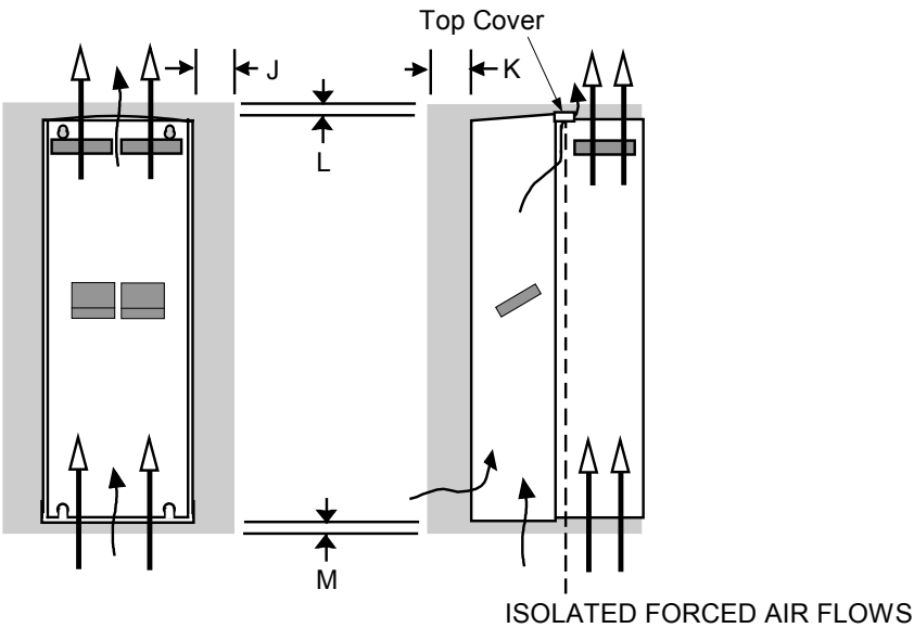
Figure Chapter 3 -9 Air Clearance for a Wall-Mount Product/Application
