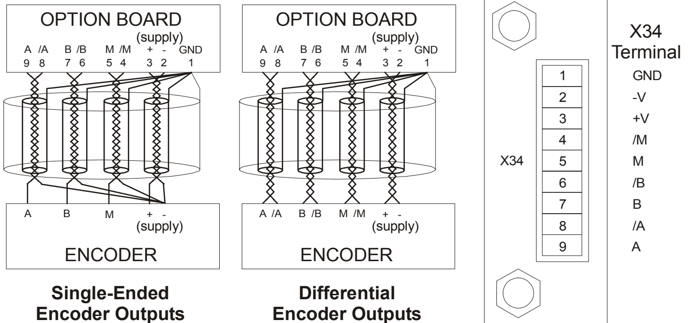
Figure 4 Wiring Diagram
