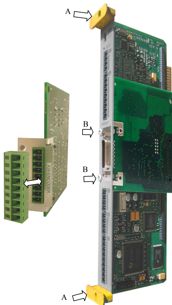
Figure 2 Control board showing Option correctly mounted
