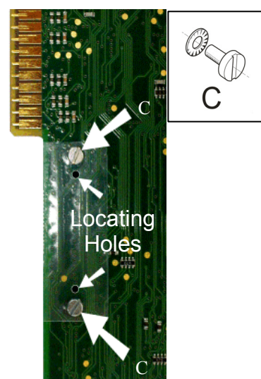
Figure 3 Rear of Control Board
