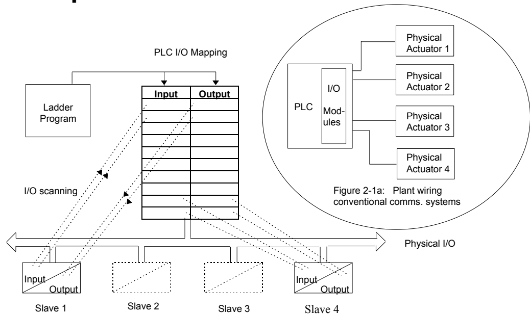
Figure 2 PROFIBUS compared with convetional comms. systems
