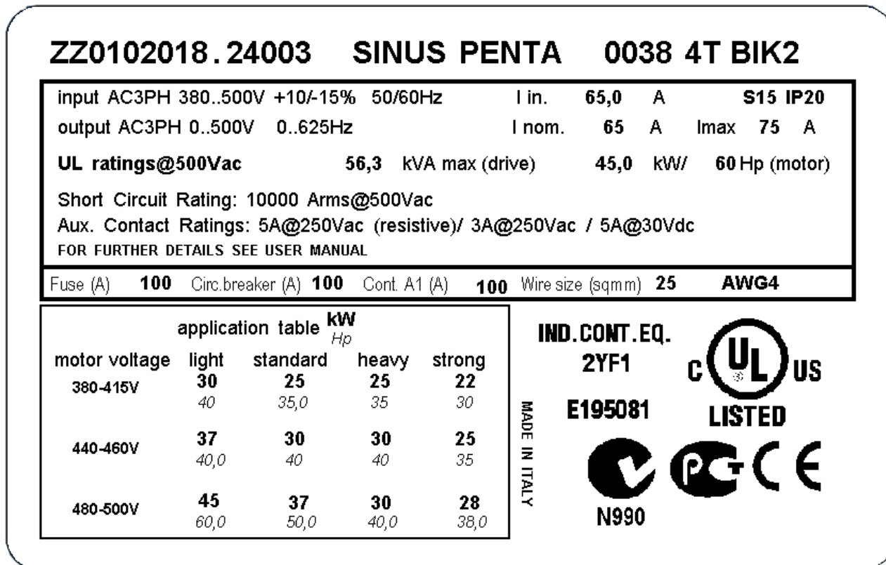
Figure 1: Nameplate of the SINUS PENTA Drive.
