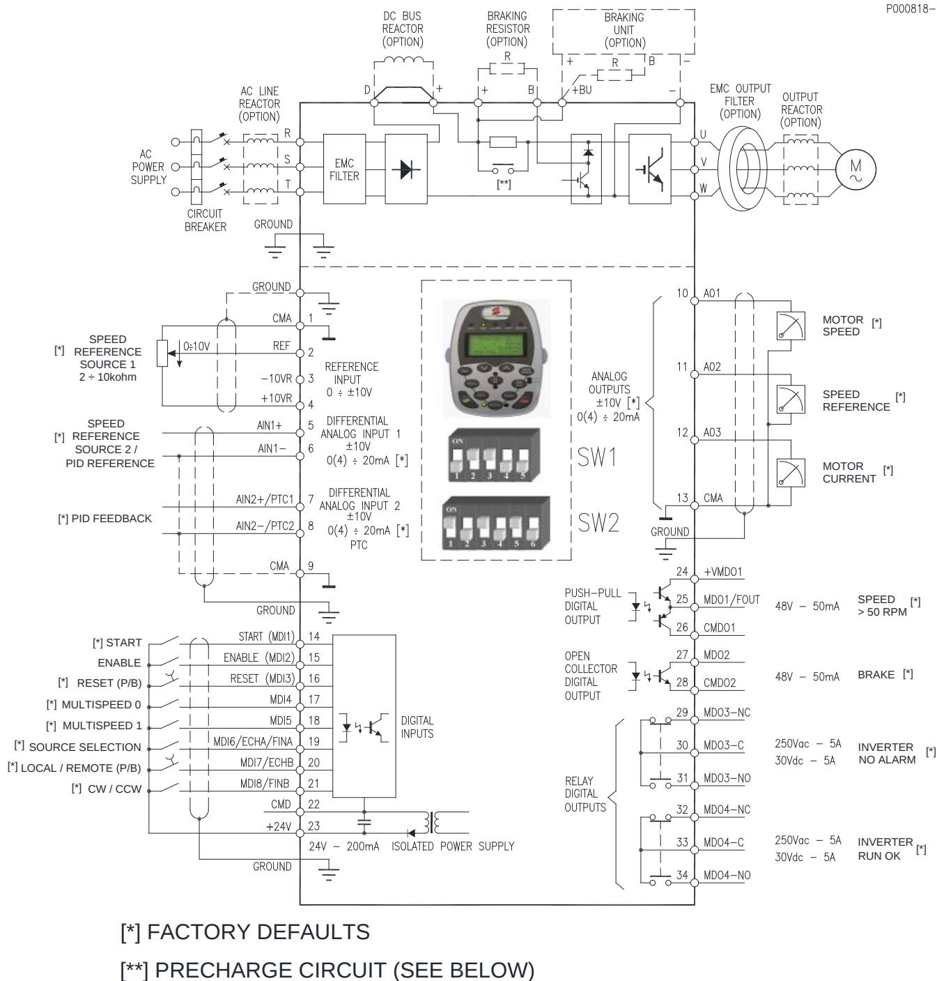
Figure 9: Wiring Diagram.
