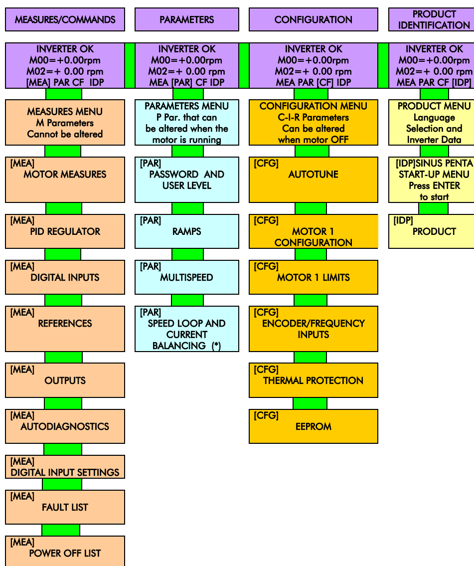
Figure 7: Menu Tree.
