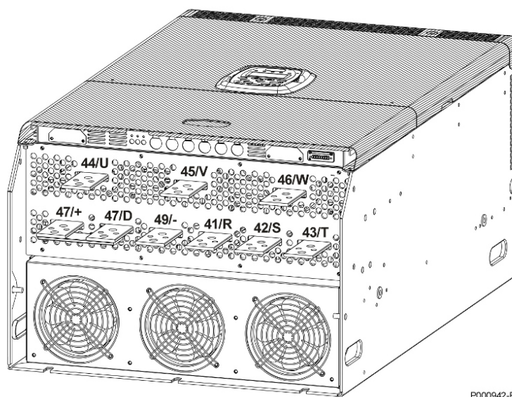
Figure 2: Connection bars in S41-S42-S51-S52
