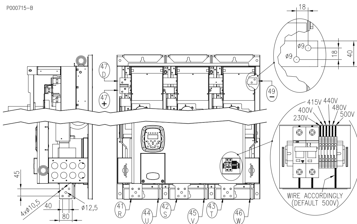
Figure 3: S60 Connection bars
