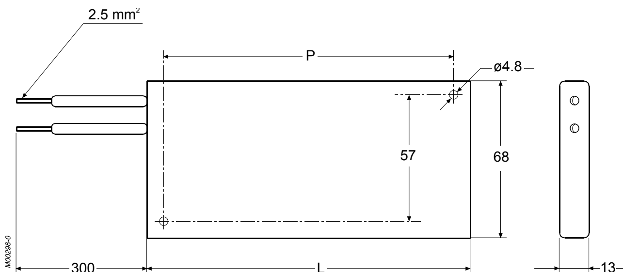
Figure 48: Overall dimensions and ratings for 75Ω/1300W braking resistor.
