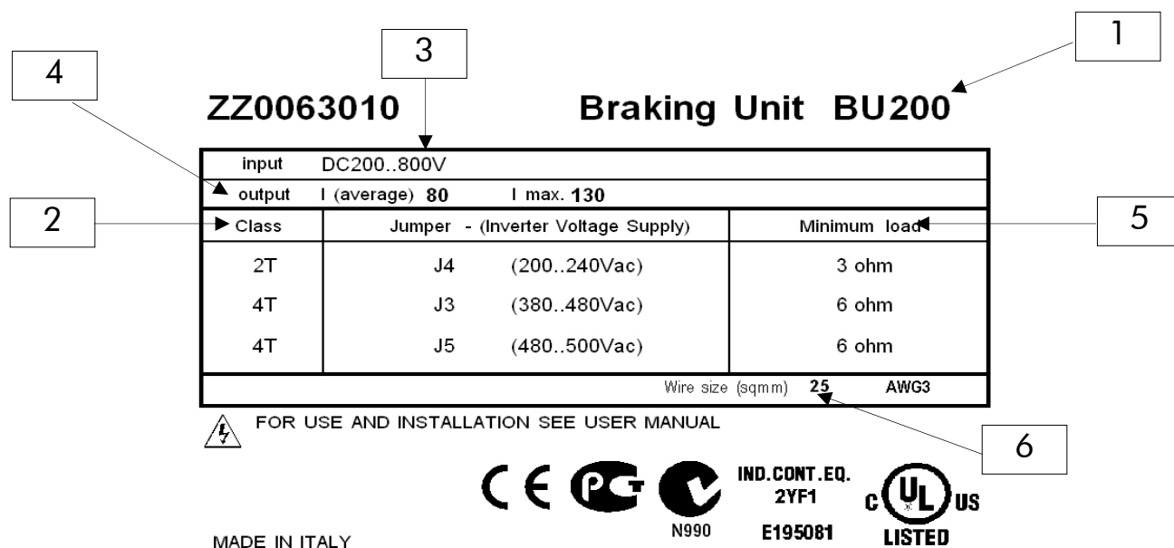
Figure 53: Nameplate of BU200.
