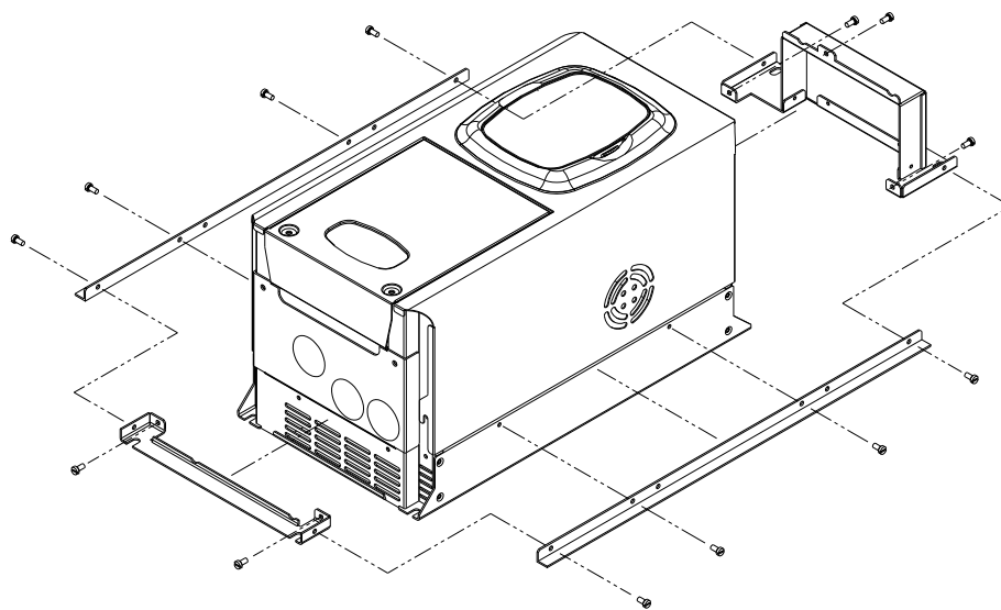
Figure 13: Mounting the accessories for the through-panel assembly of SINUS K S10.
