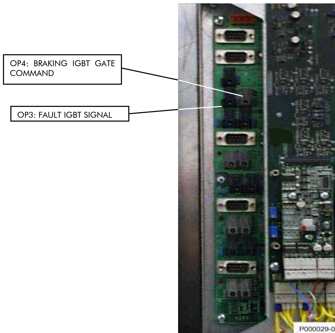
Figure 67: Wiring points of the optical fibres in ES482 control board.
