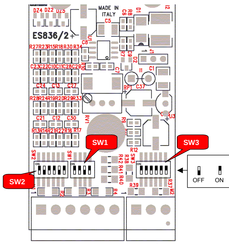
Figure 80: Positions and default settings of the configuration dip-switches.
