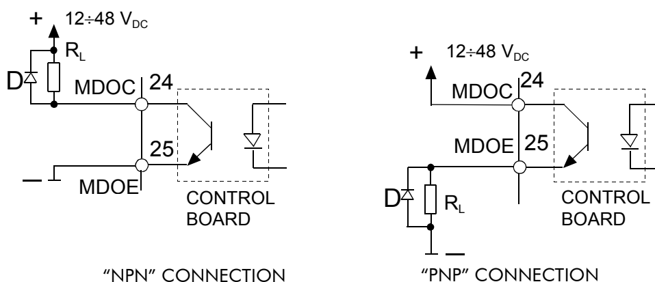
Figure 41: Connecting a relay to the OPEN COLLECTOR output.
