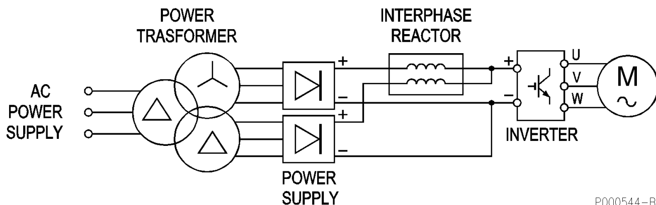
Figure 73: Lay-out of a 12-phase connection.
