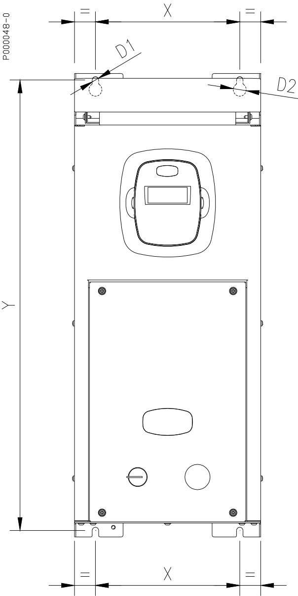
Figure 10: Fixing points for IP54 SINUS K.
