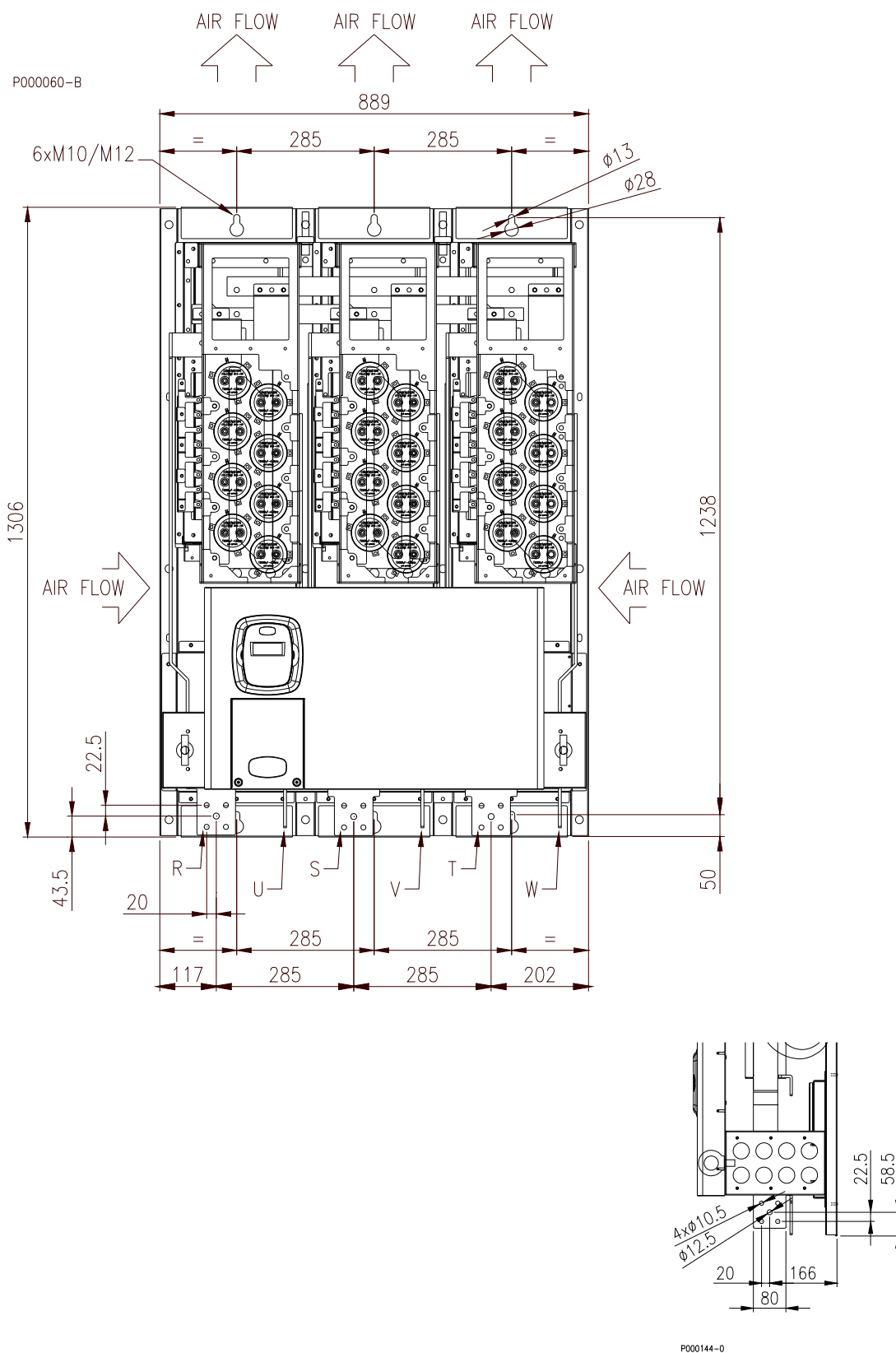
Figure 5: Fixing points for stand-alone models (S60).
