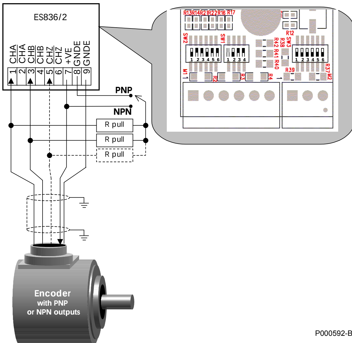
Figure 83: PNP or NPN encoder with single-ended outputs and load resistors with external wiring.
