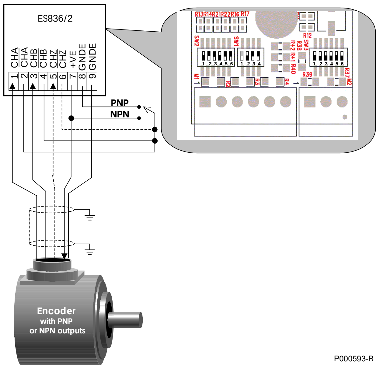
Figure 84: PNP or NPN encoder with single-ended outputs and internal load resistors.
