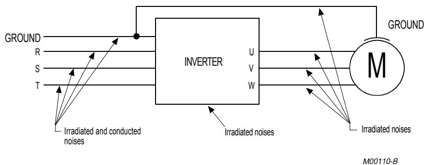
Figure 91: Disturbance sources in a power drive system equipped with an inverter.
