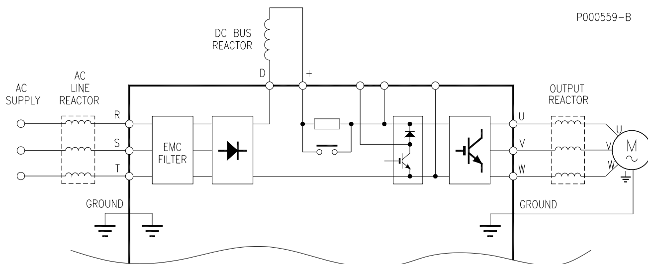
Figure 71: Wiring diagram for optional inductance.
