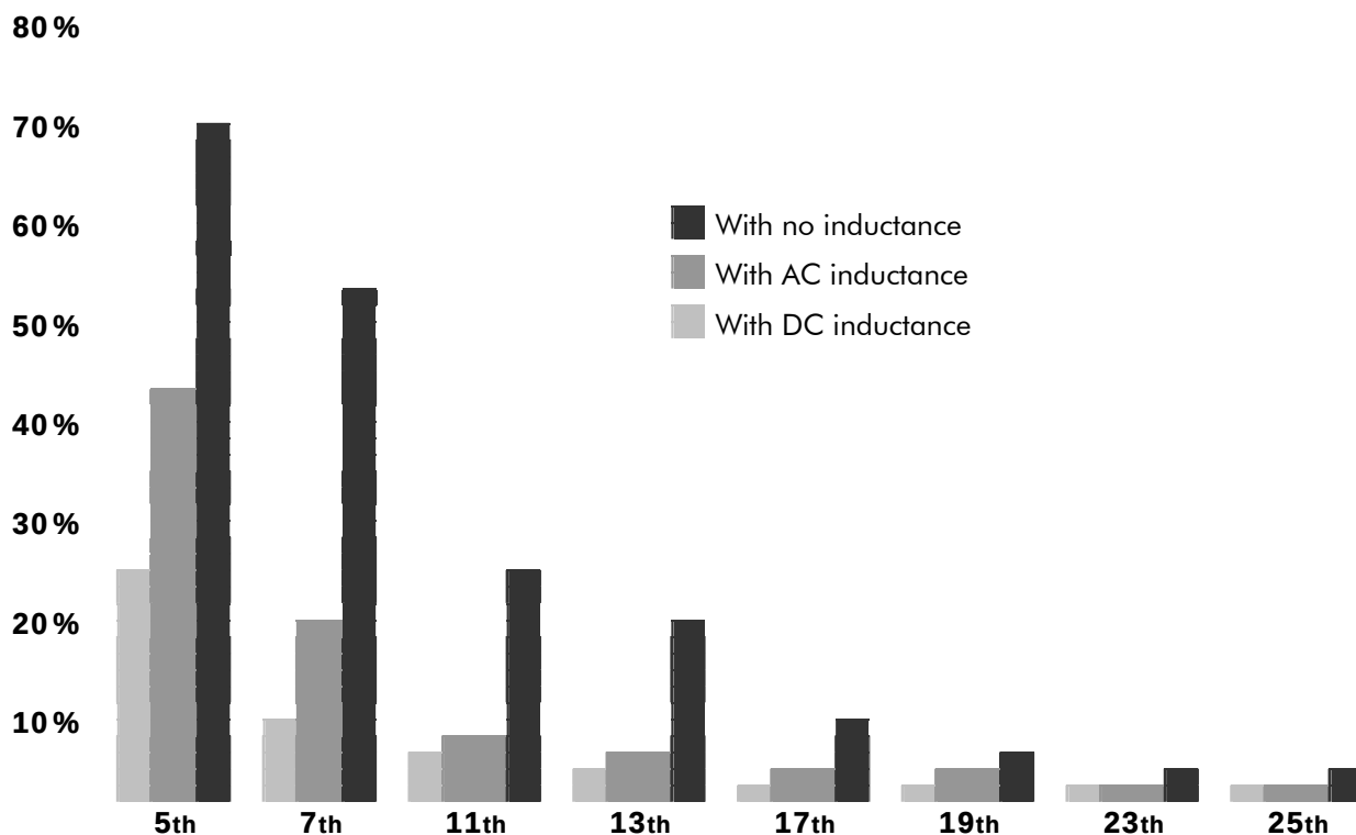
Figure 72: Amplitude of harmonic currents (approximate values)
