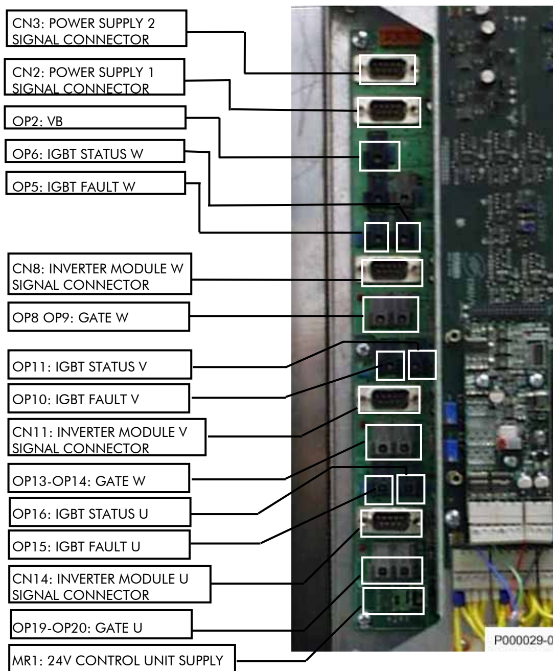
Figure 33: ES842 control unit.
