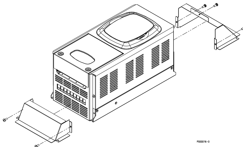
Figure 11: Mounting the accessories for the through-panel assembly of SINUS K S05.
