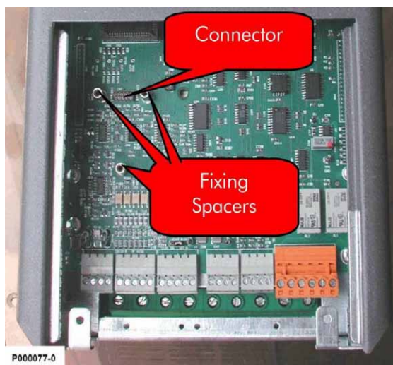
Figure 78: Position of the slot for the installation of the encoder board.
