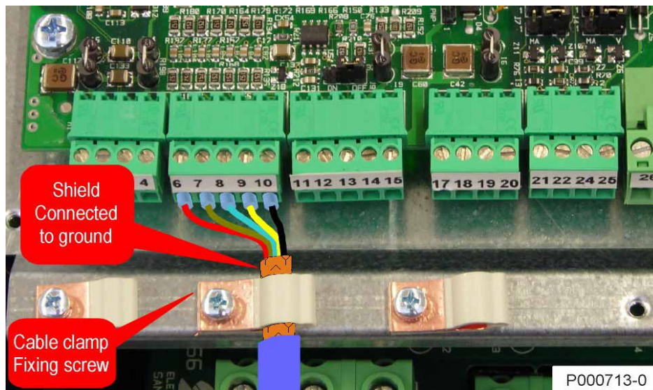
Figure 37: Tightening a signal screened cable.
