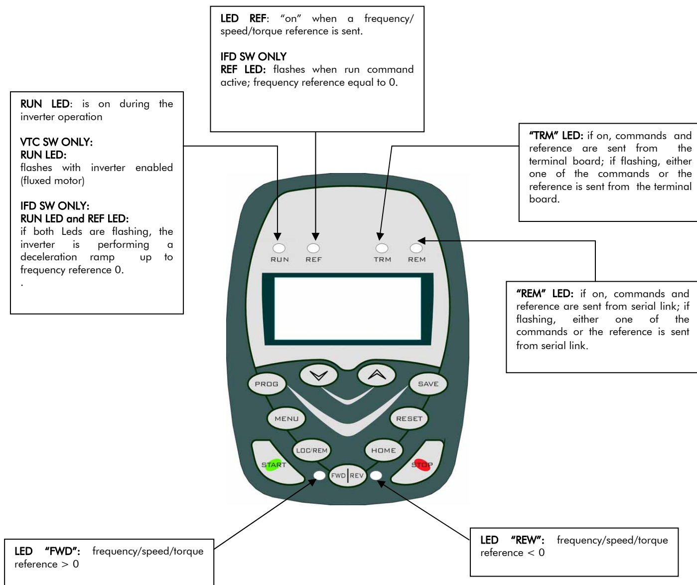
Figure 3: Keypad of SINUS K inverters.
