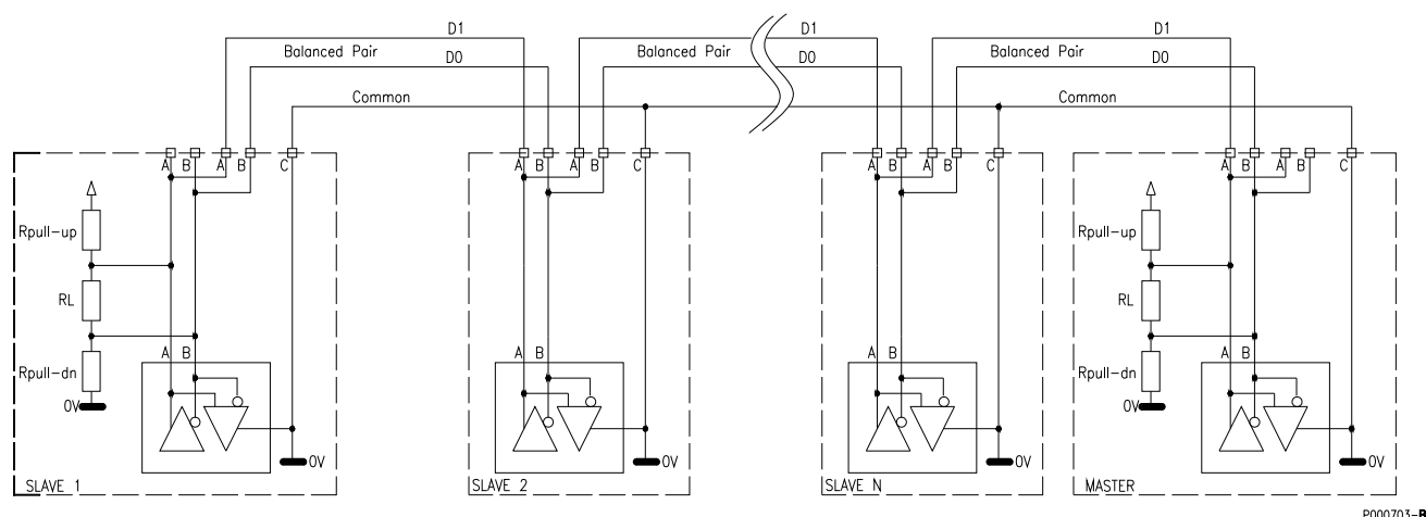
Figure 46: Recommended wiring diagram for "2-wire" MODBUS wiring.
