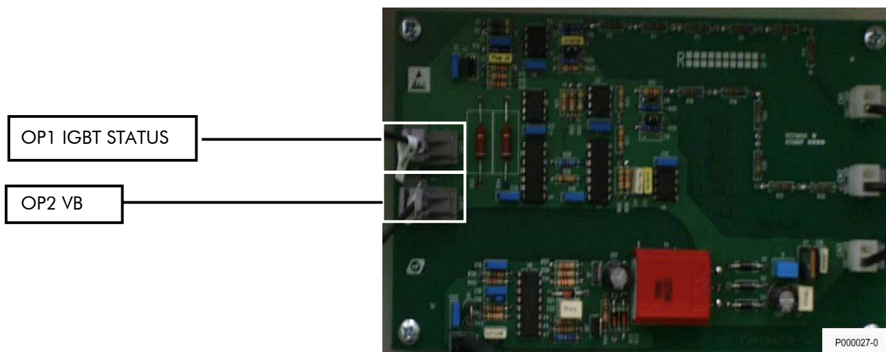
Figure 32: ES843 inverter module.
