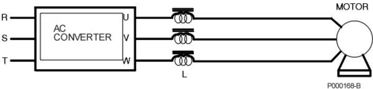
Figure 74: Connection of an output inductance.
