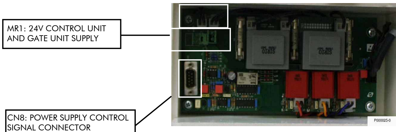
Figure 30: ES840 supply control board.
