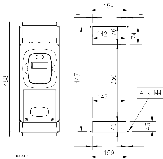
Figure 12: Fixing points of the mounting panel for the through-panel assembly of SINUS K S05.
