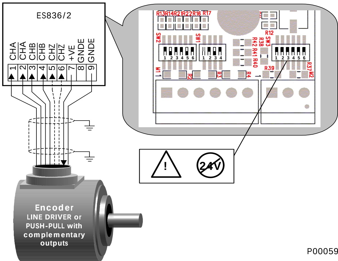
Figure 81: LINE DRIVER or PUSH-PULL encoder with complementary outputs.
