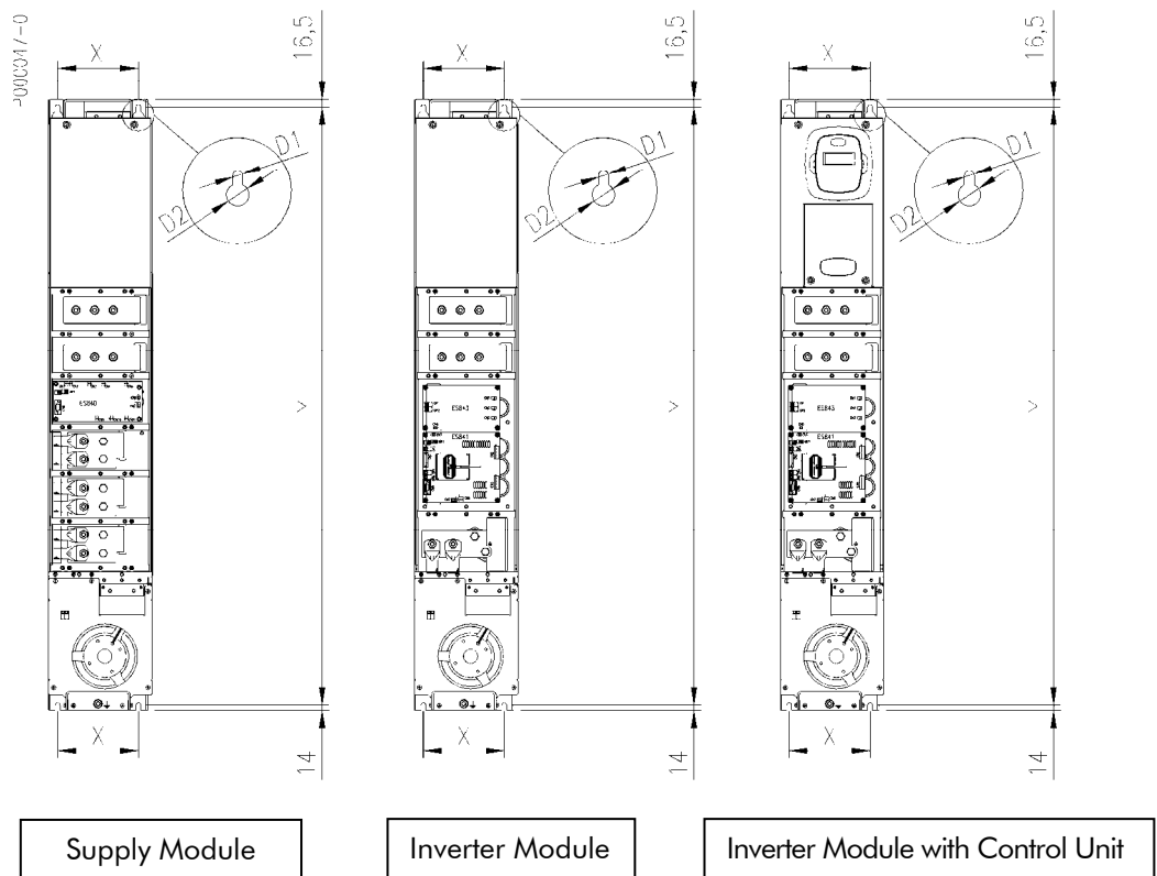
Figure 6: Fixing points for modular units.
