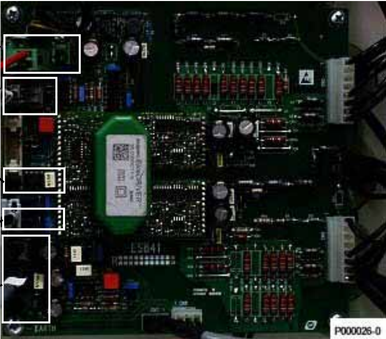
Figure 66: ES841 gate unit board for the braking unit.
