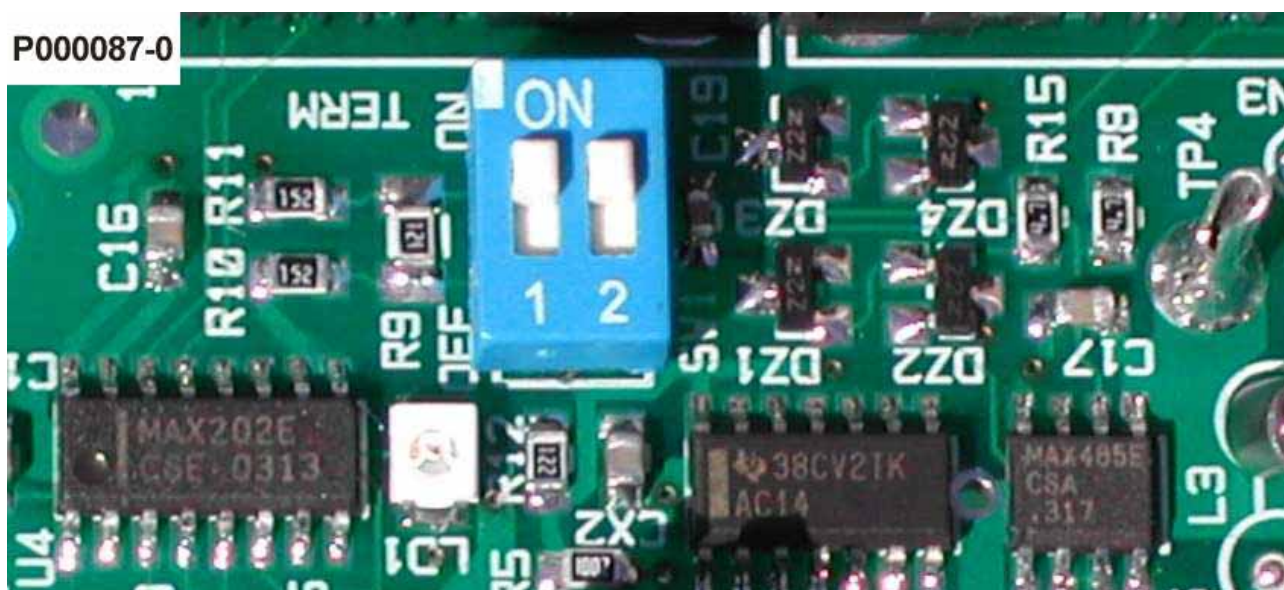
Figure 89: Configuring the dip-switch for RS485 terminator.
