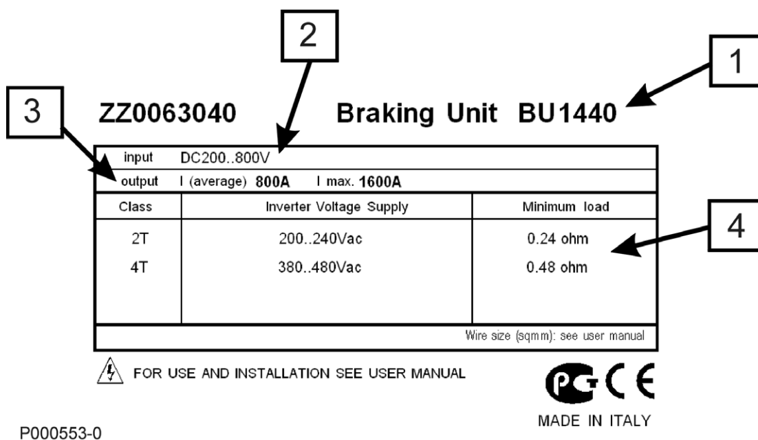
Figure 63: Nameplate of BU720-1440.
