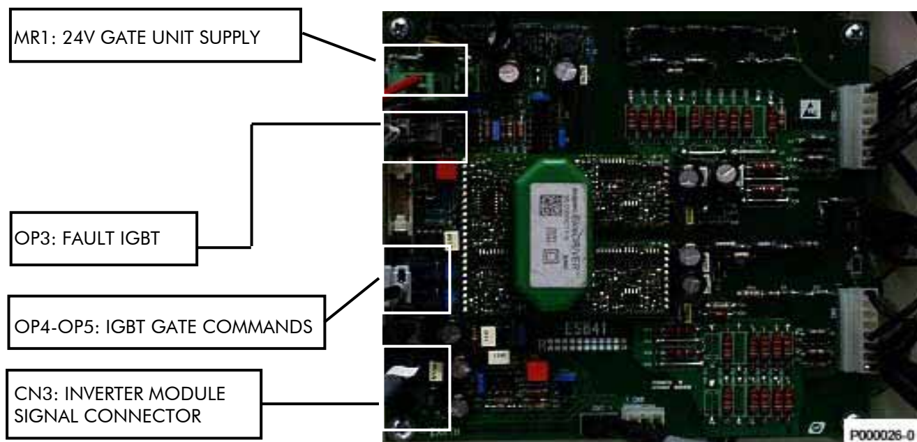
Figure 31: ES841 inverter module gate unit board.
