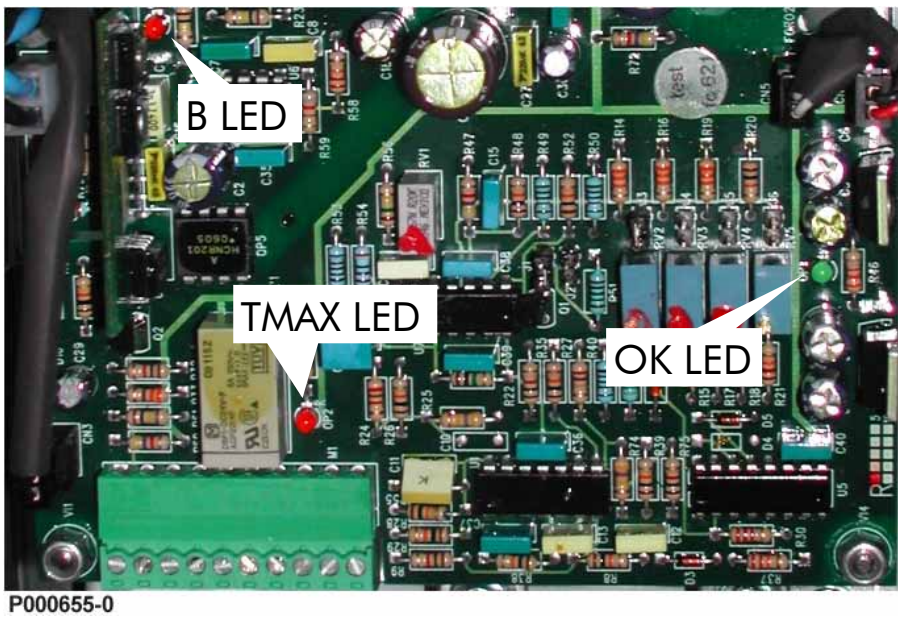
Figure 56: Position of the indicator LEDs.
