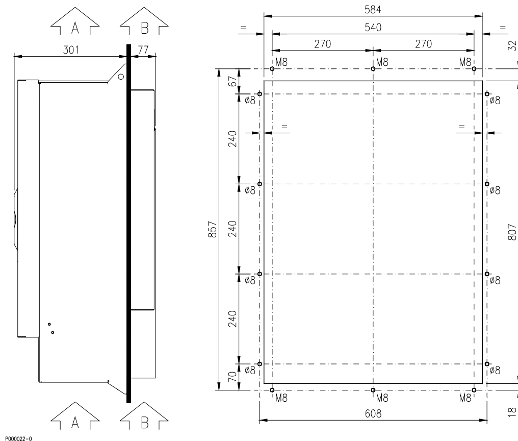
Figure 19: Through-panel assembly and fixing points for SINUS K S40.
