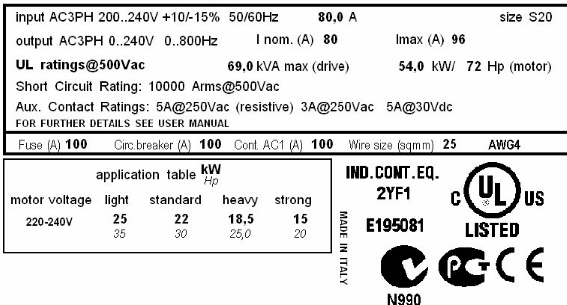
Figure 1: Example of a nameplate placed on a 2T SINUS K inverter.
