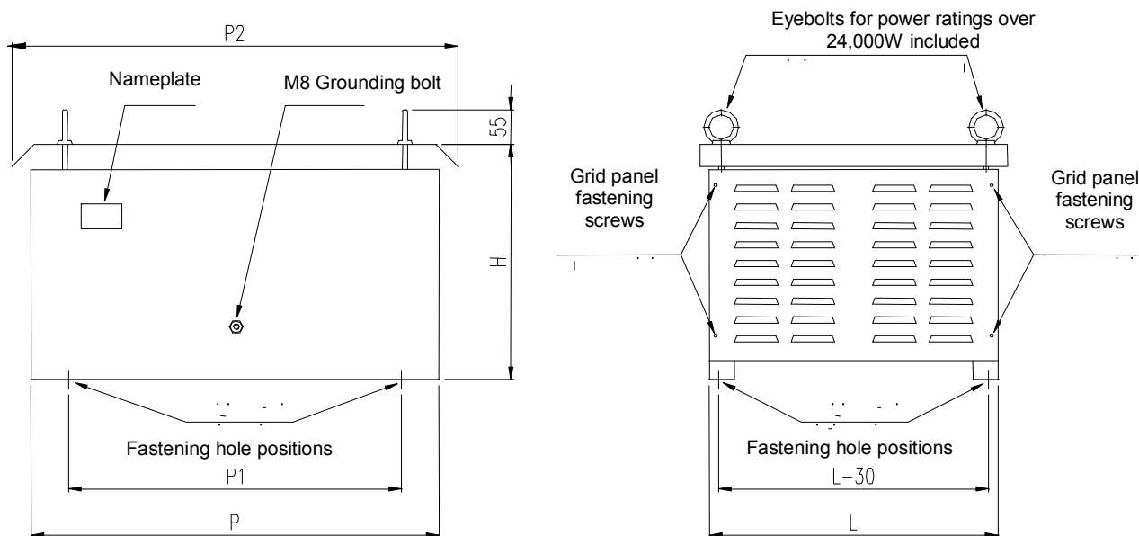
Figure 51: Overall dimensions for IP23 box resistors.
