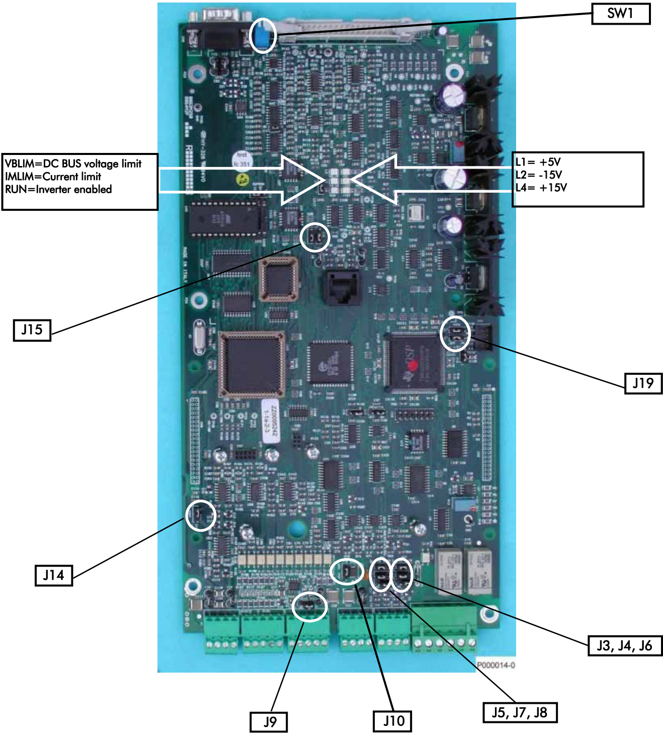
Figure 42: Location of the jumpers on ES778 control board.
