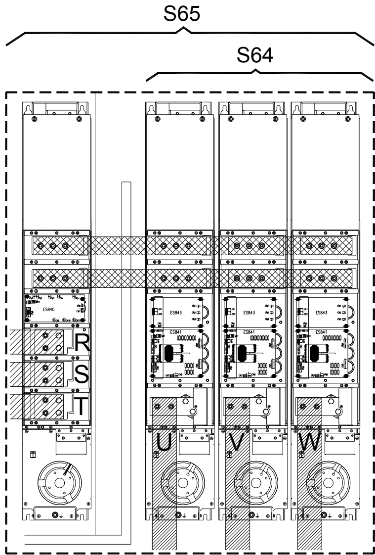
Figure 39: Connecting bars for S64 – S65.
