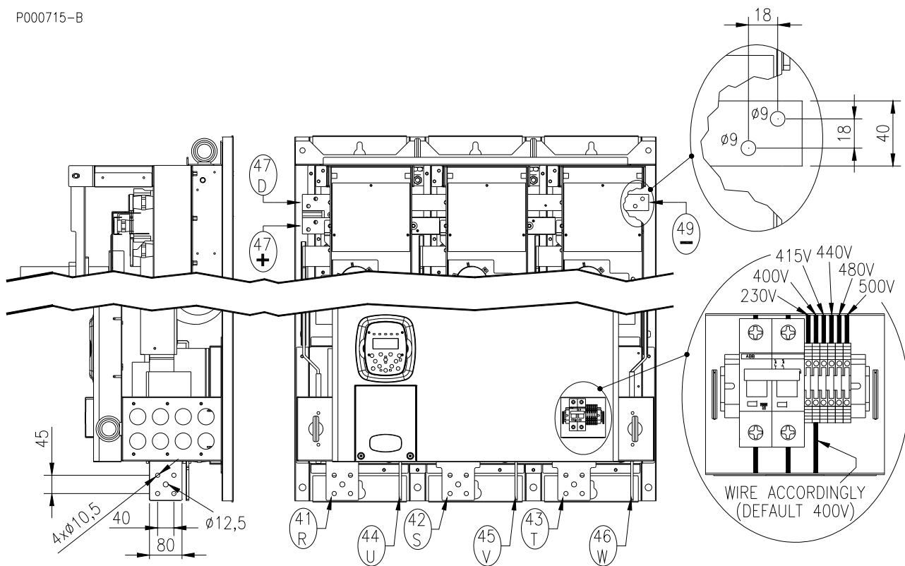
Figure 38: Connecting bars for S60.
