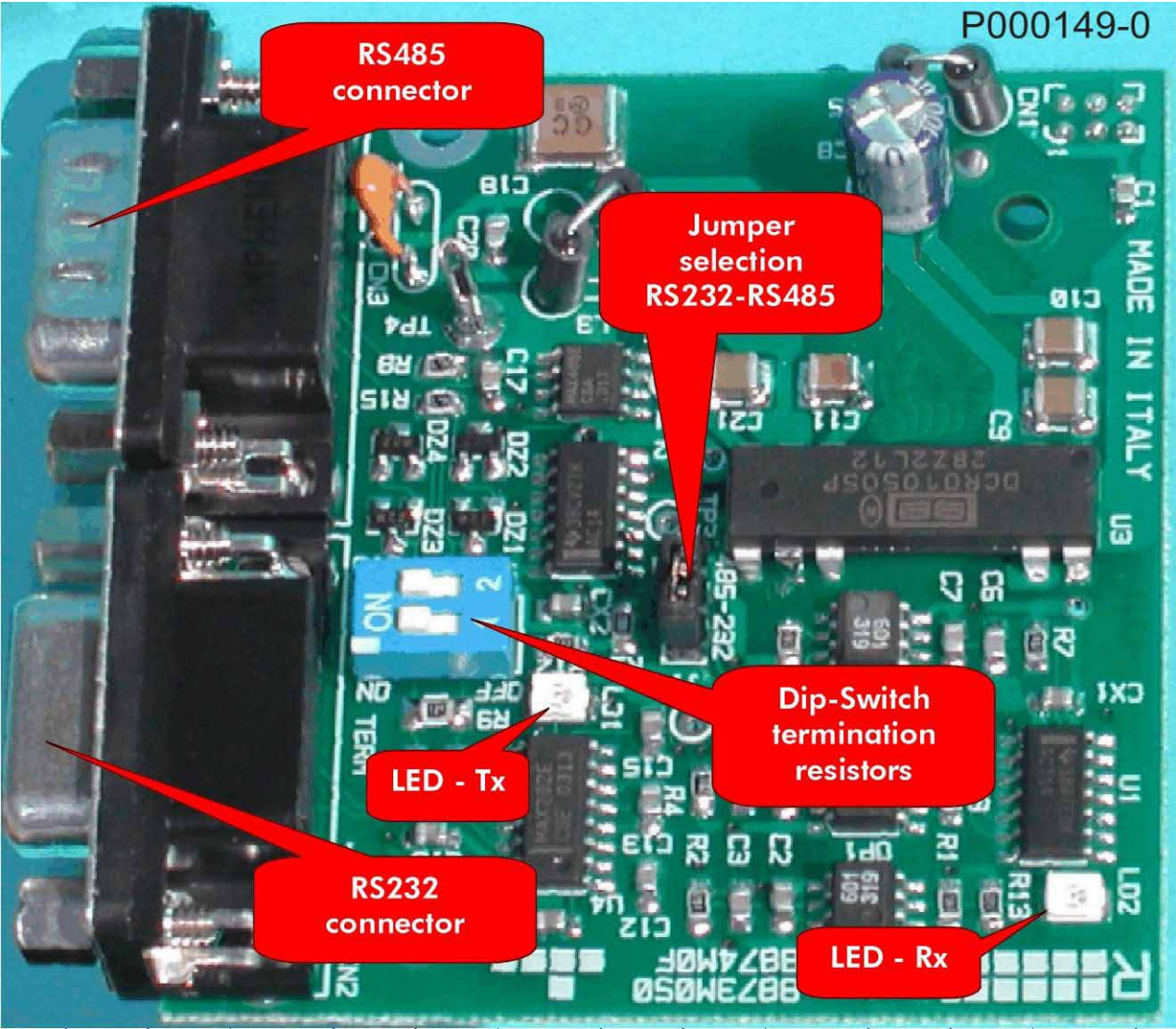
Figure 86: ES822 isolated board.
