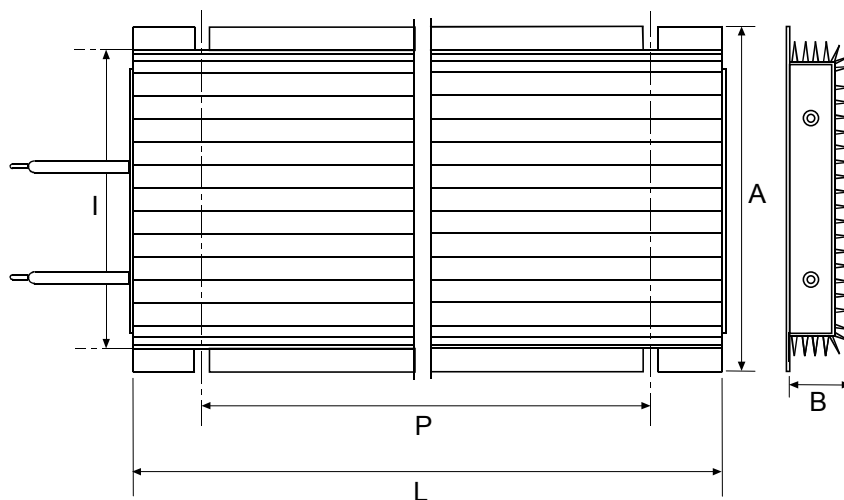
Figure 49: Overall dimensions and mechanical features for braking resistors from 1100W to 2200W.
