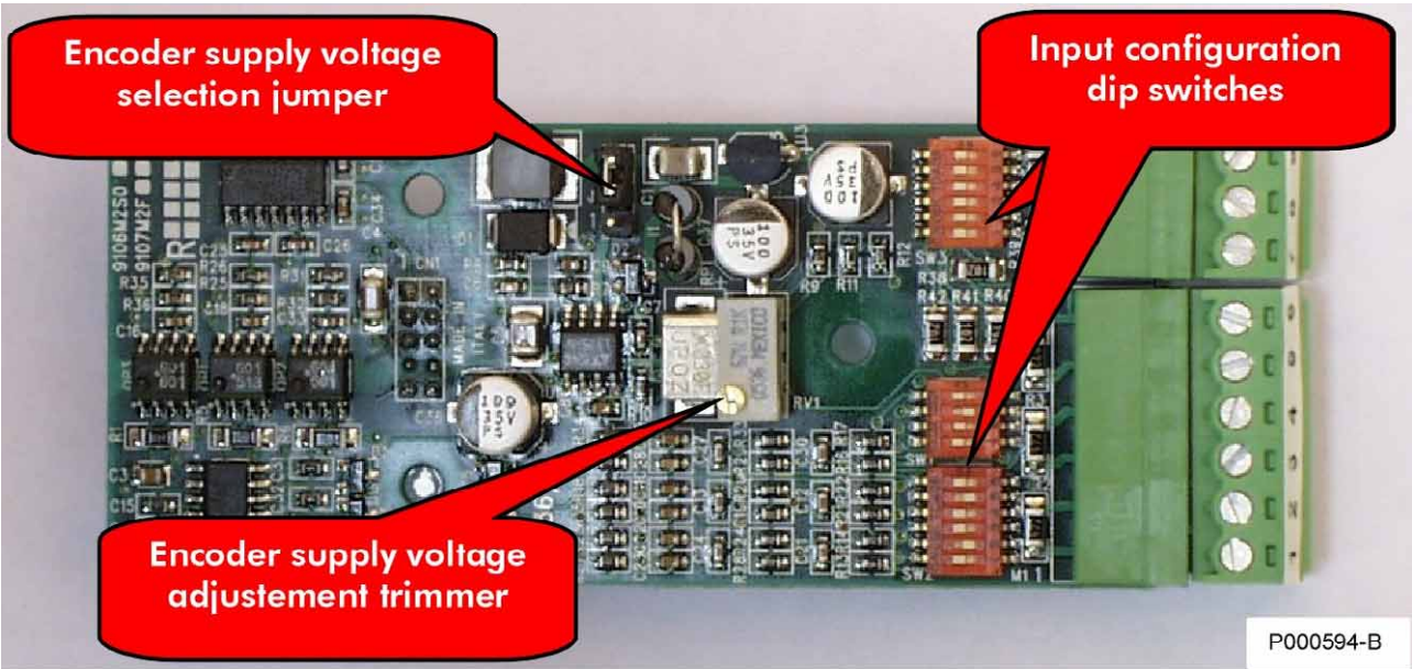
Figure 77: ES836/2 Encoder board.
