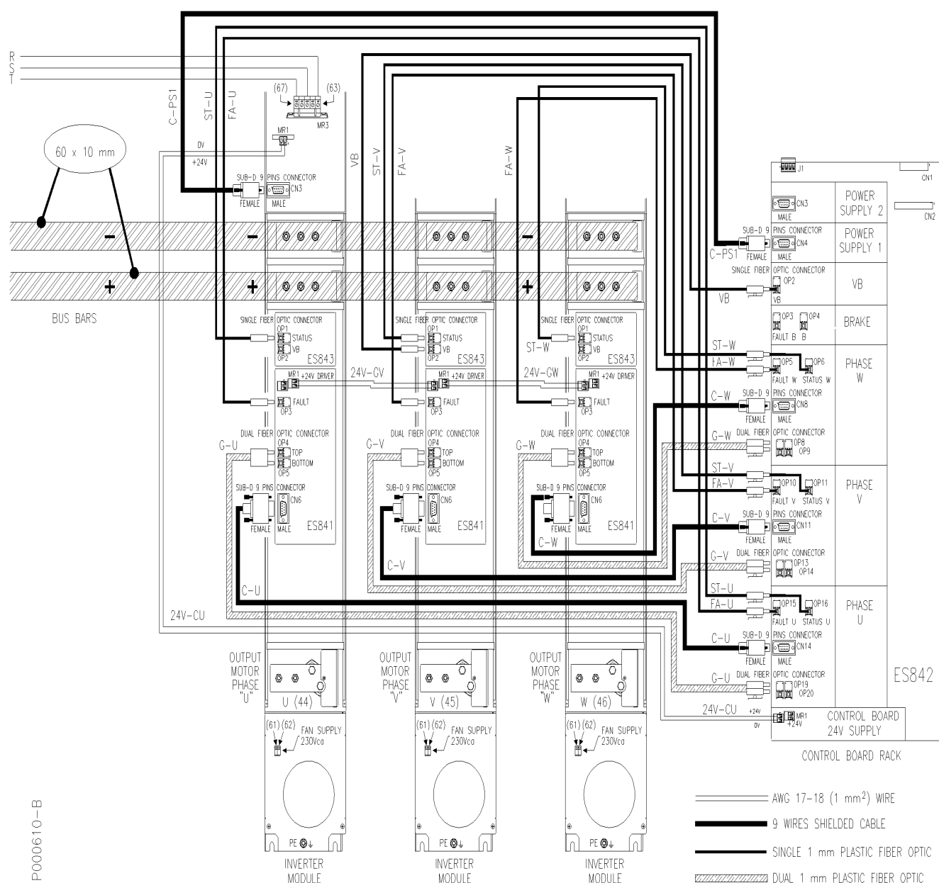
Figure 36: Internal wiring for S64 inverters.
