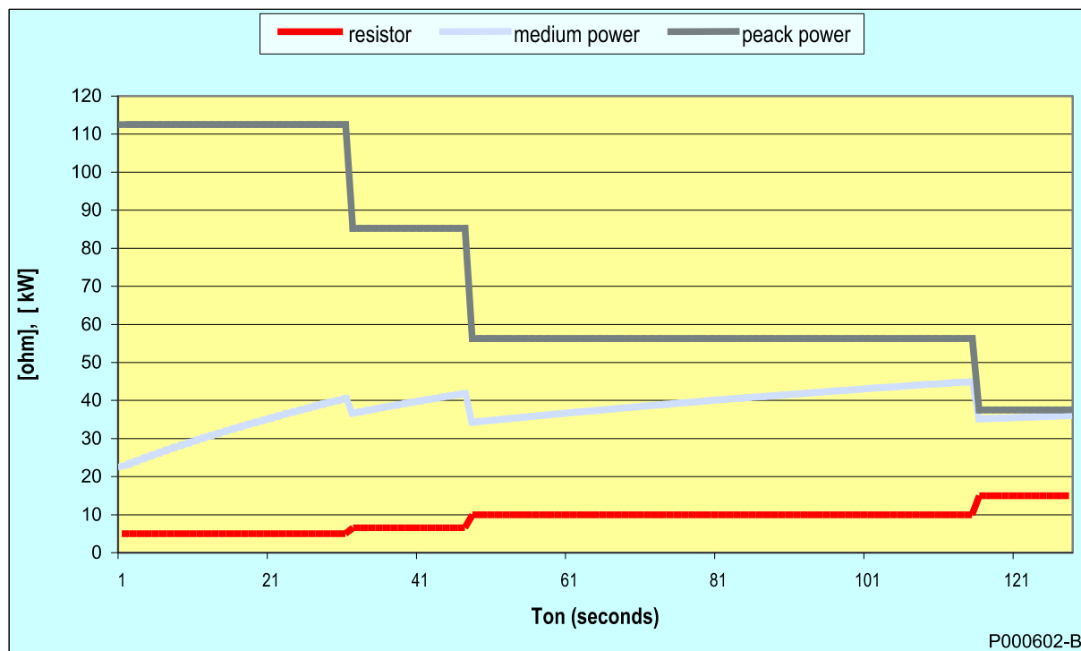
Figure 62: Peak power and average power (depending on Ton) dissipated to the braking resistor.
