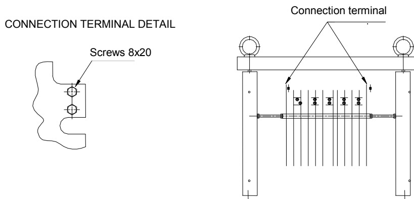
Figure 52: Position of the electrical connections in box resistors.
