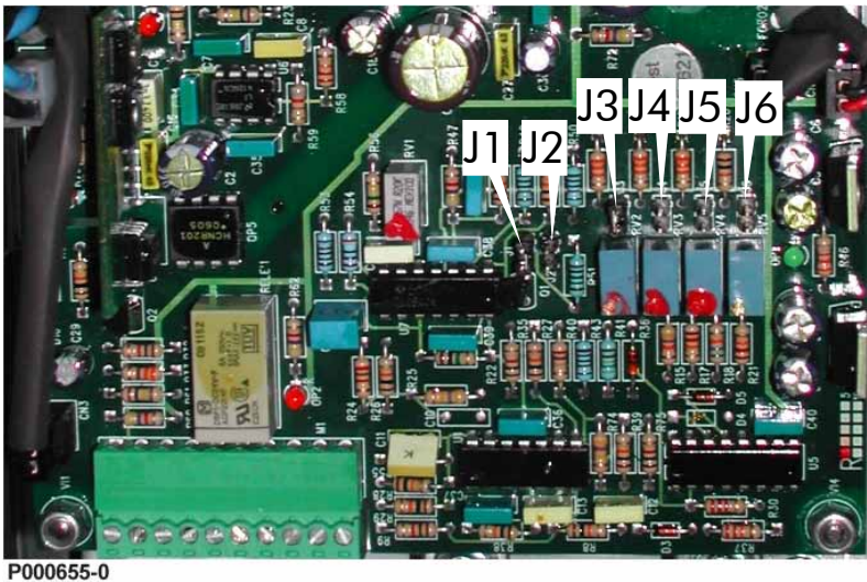
Figure 54: Position of the jumpers on ES839 BU200 control board.
