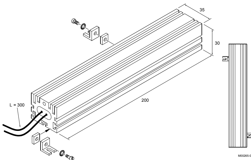
Figure 47: Overall dimensions for 56-100Ω/350W resistor.
