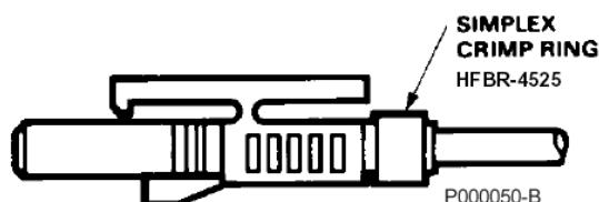
Figure 27: Single optical fibre connector.
