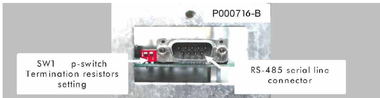
Figure 43: Location of SW1 dip-switch and RS485 connector for Sinus K S05 to S20.
