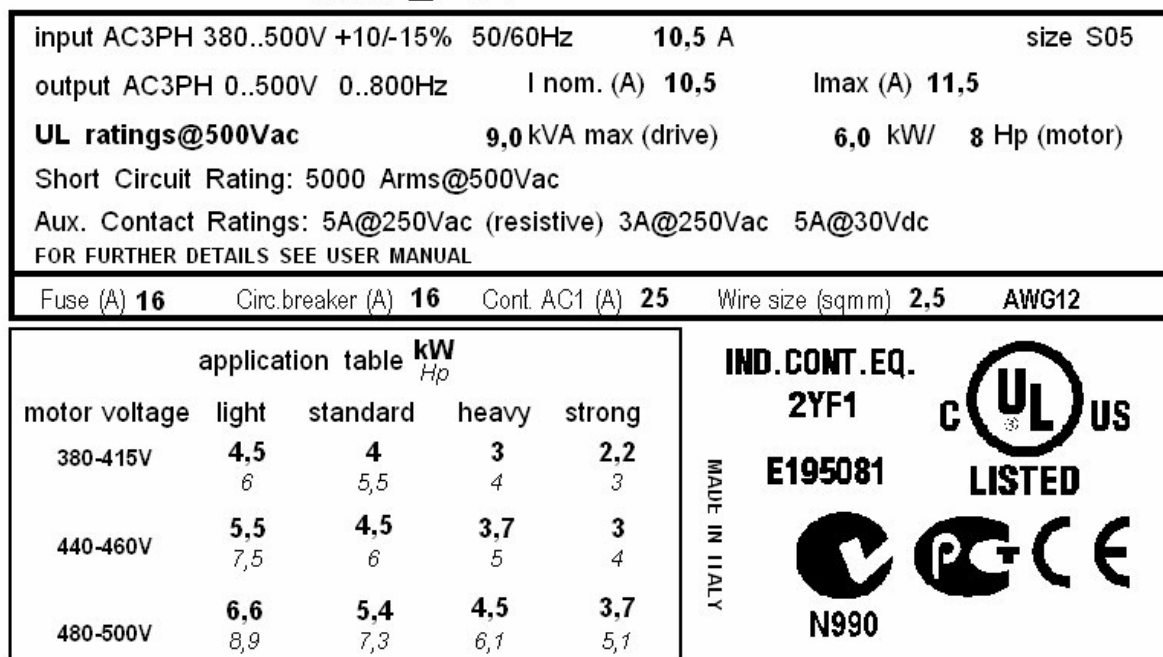
Figure 2: Example of a nameplate placed on a 4T SINUS K inverter.
