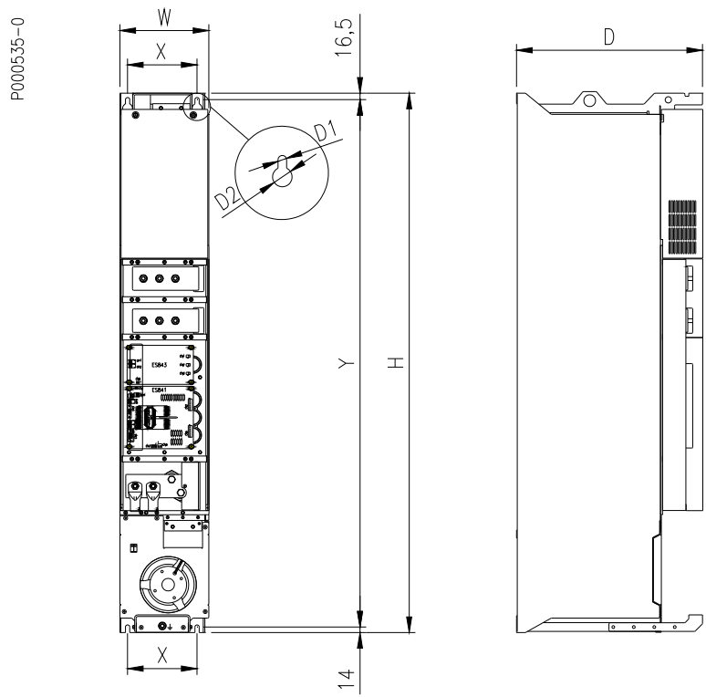
Figure 64: Dimensions and fixing points of BU720-1440.
