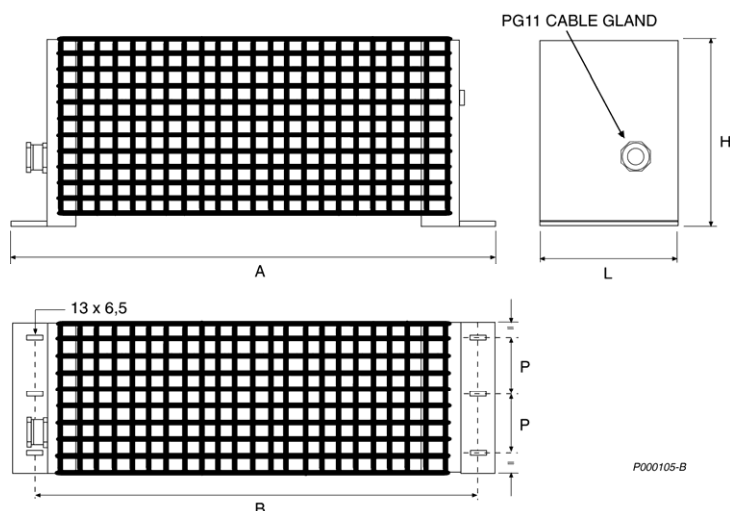
Figure 50: Overall dimensions for 4kW, 8kW, 12kW braking resistors.
