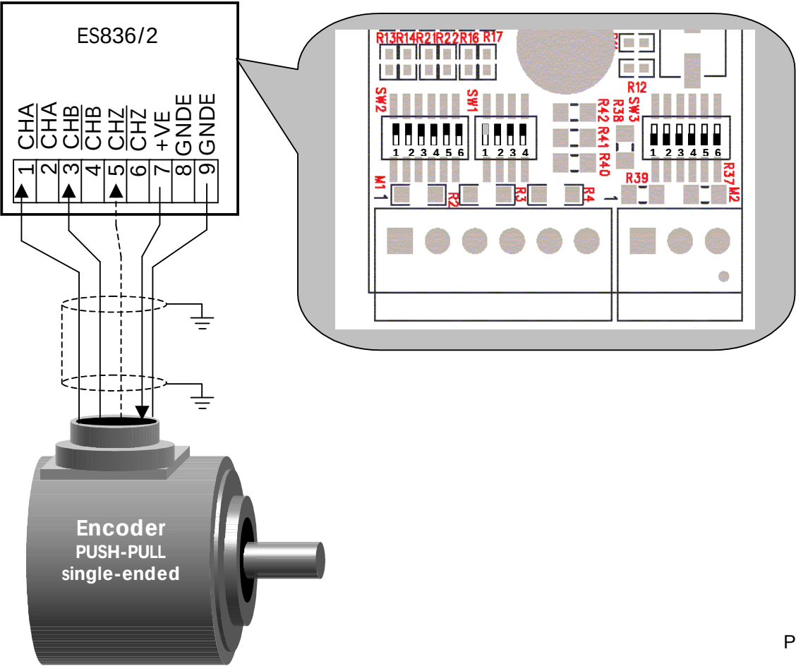
Figure 82: PUSH-PULL encoder with single-ended outputs.
