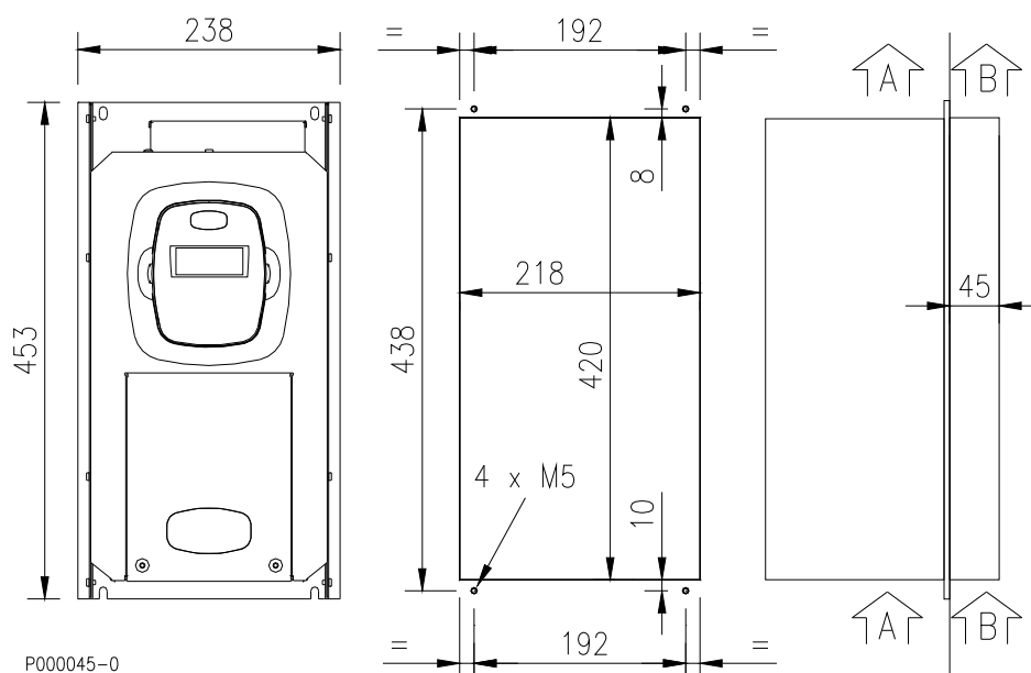
Figure 14: Fixing points of the mounting panel for the through-panel assembly of SINUS K S10.
