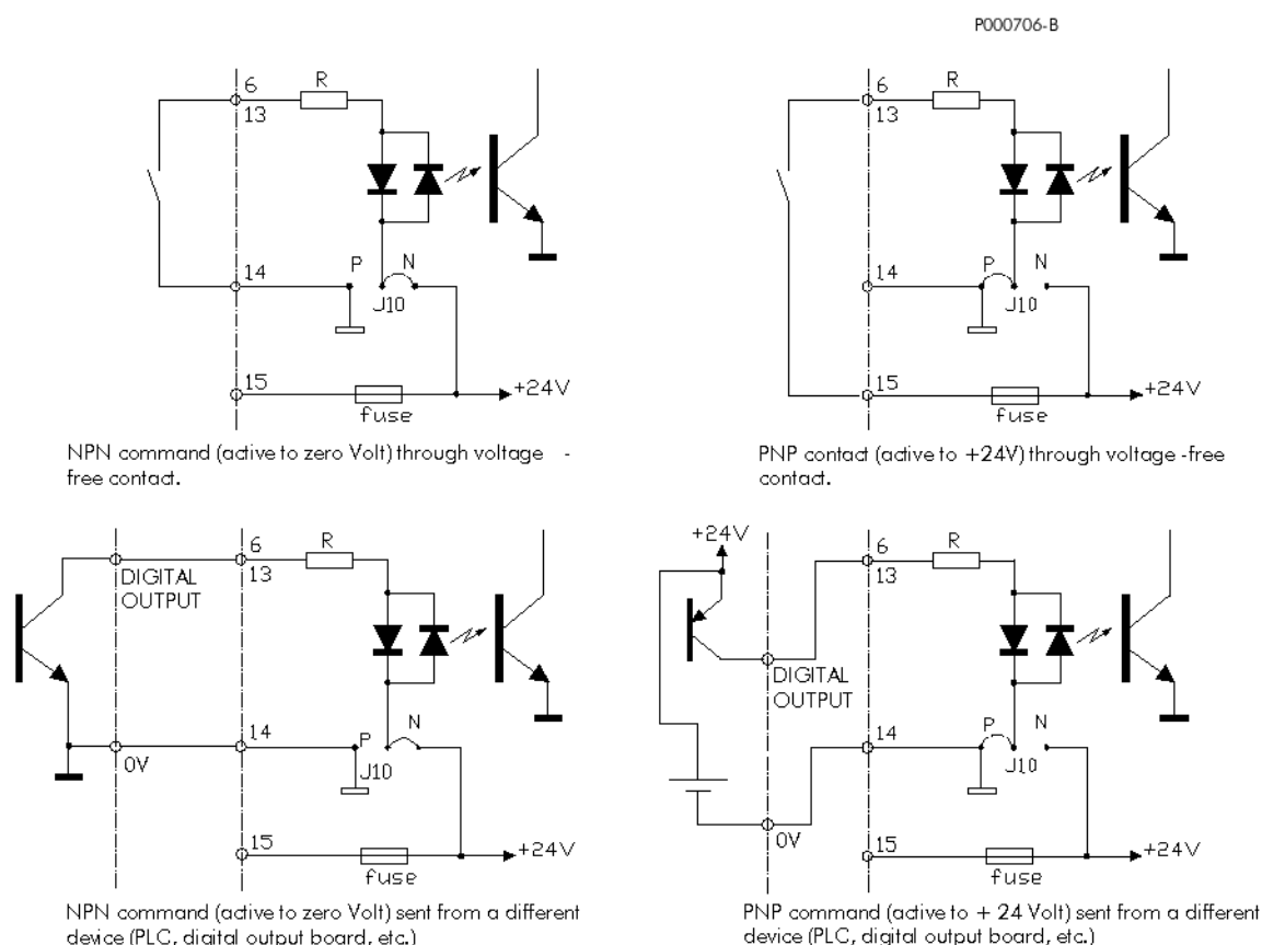
Figure 40: Control modes for the digital inputs.
