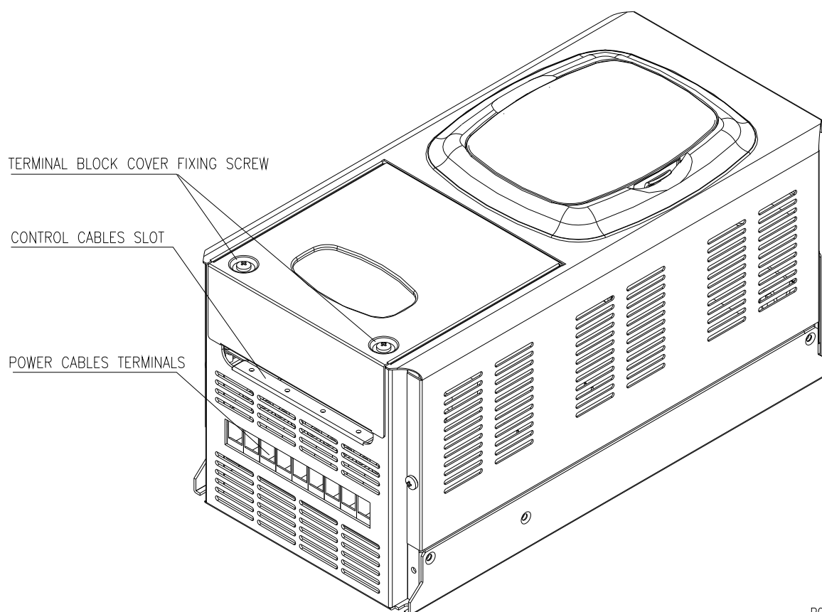
Figure 22: Access to the control terminals and power terminals.
