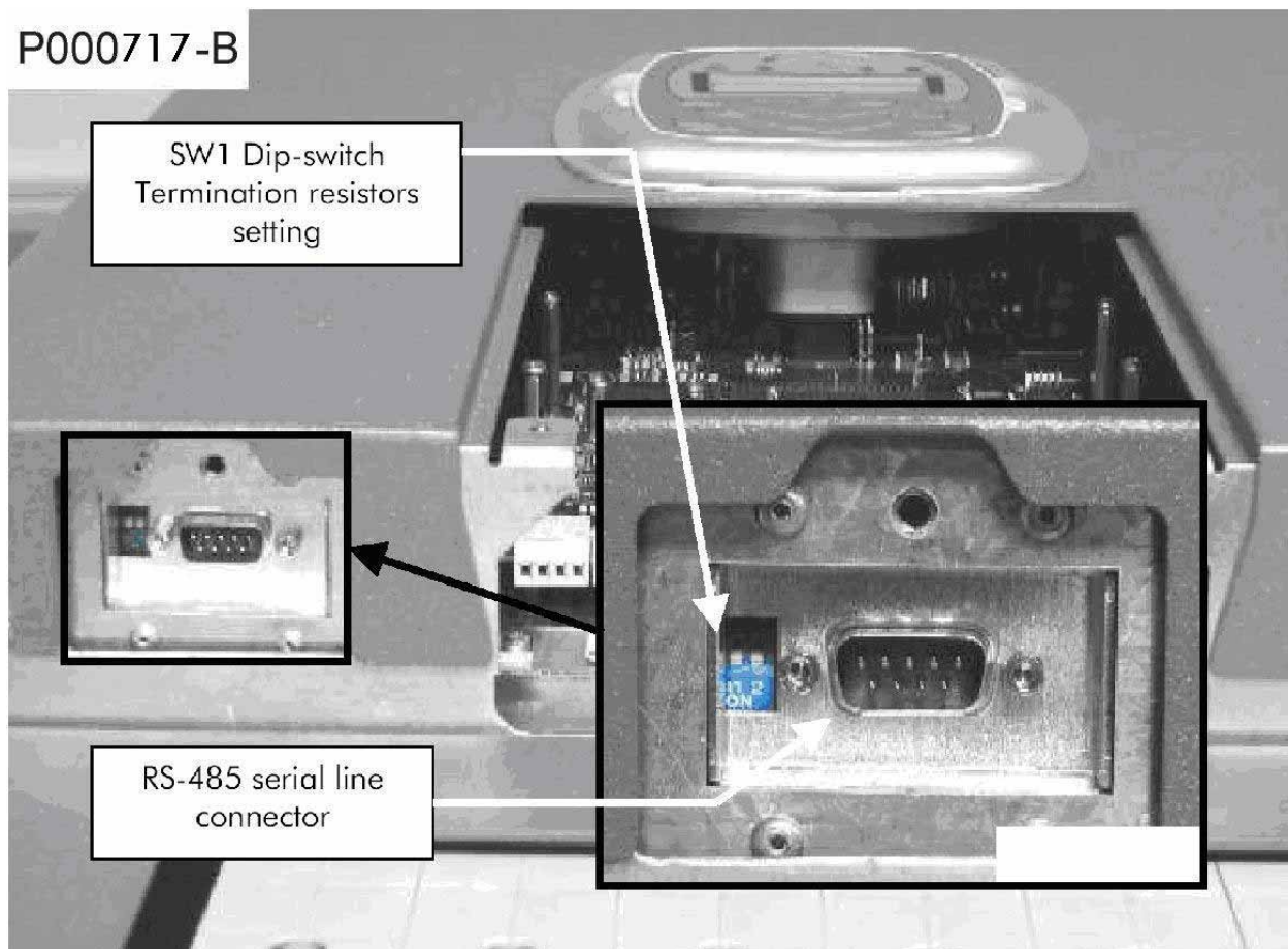
Figure 44: Location of SW1 dip-switch and RS485 connector for Sinus K S30 to S60.
