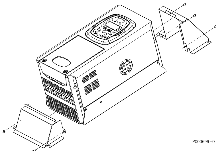
Figure 15: Fittings for the through-panel assembly for SINUS K S12.
