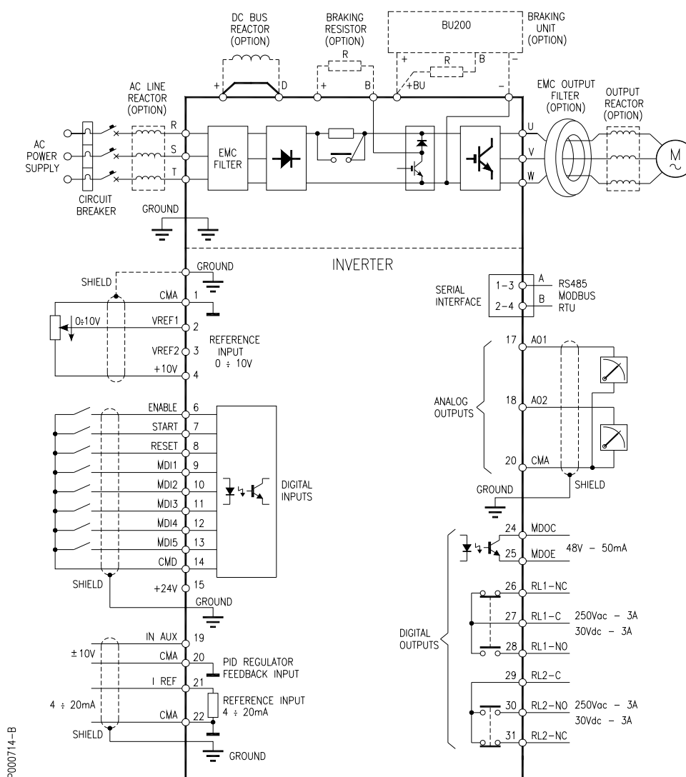
Figure 23: Wiring diagram for S05-S60.
