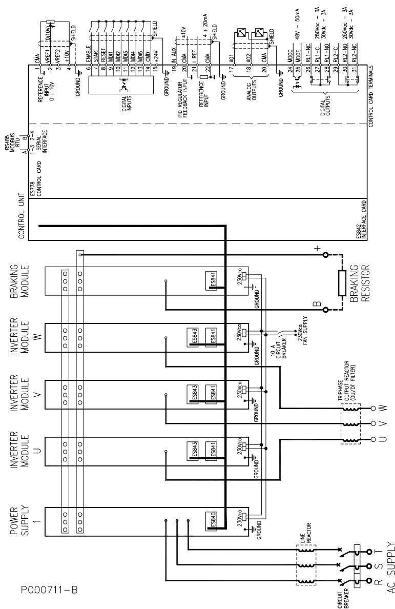
Figure 65: External power connections for S65 modular inverters provided with BU770-1440.
