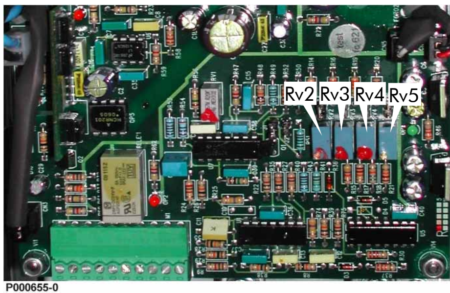
Figure 55: Positions of BU200 adjusting trimmers.
