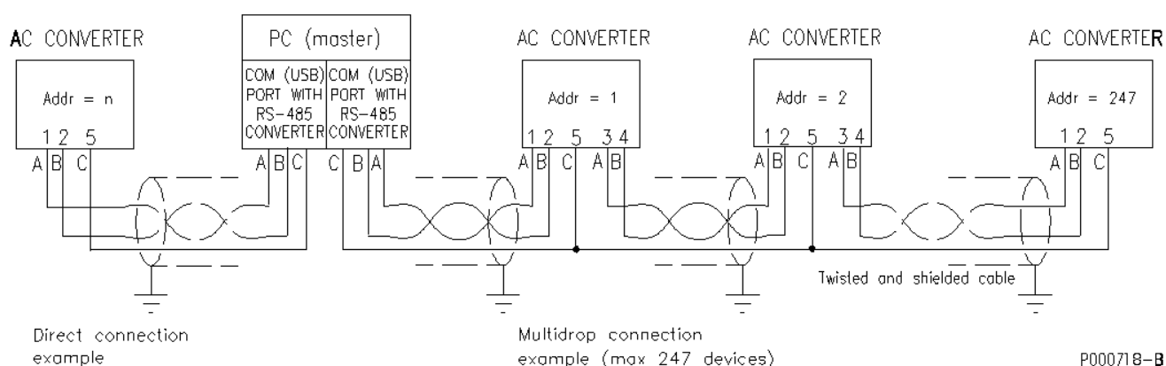
Figure 45: Example of multidrop and direct connection.
