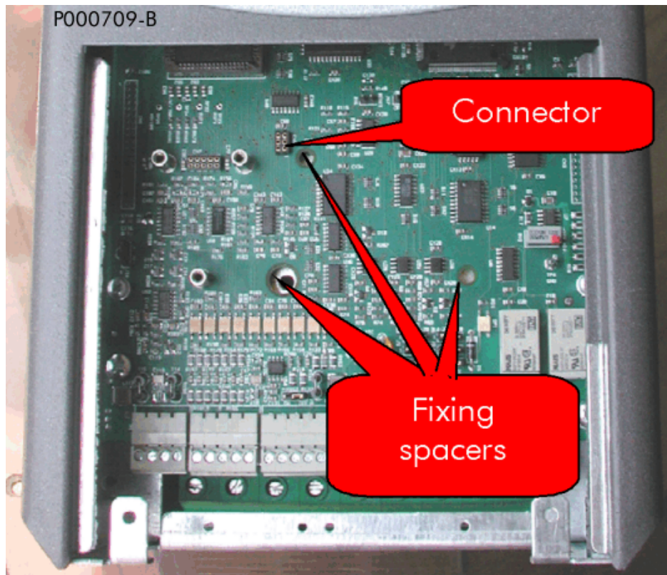
Figure 87: Position of the slot for the installation of the isolated serial board.
