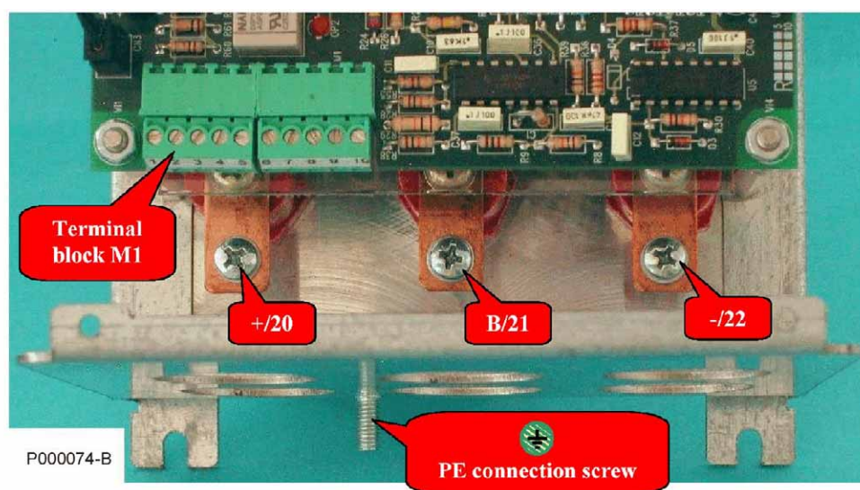
Figure 60: Terminals in BU200.
