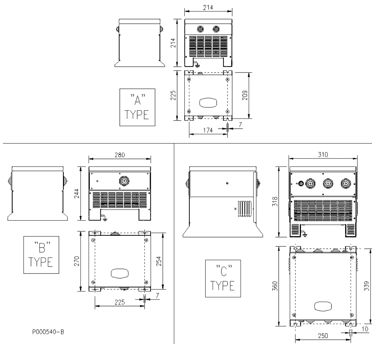
Figure 76: Mechanical features of an AC 3-phase inductance, 2T-4T Class in IP54 cabinet.
