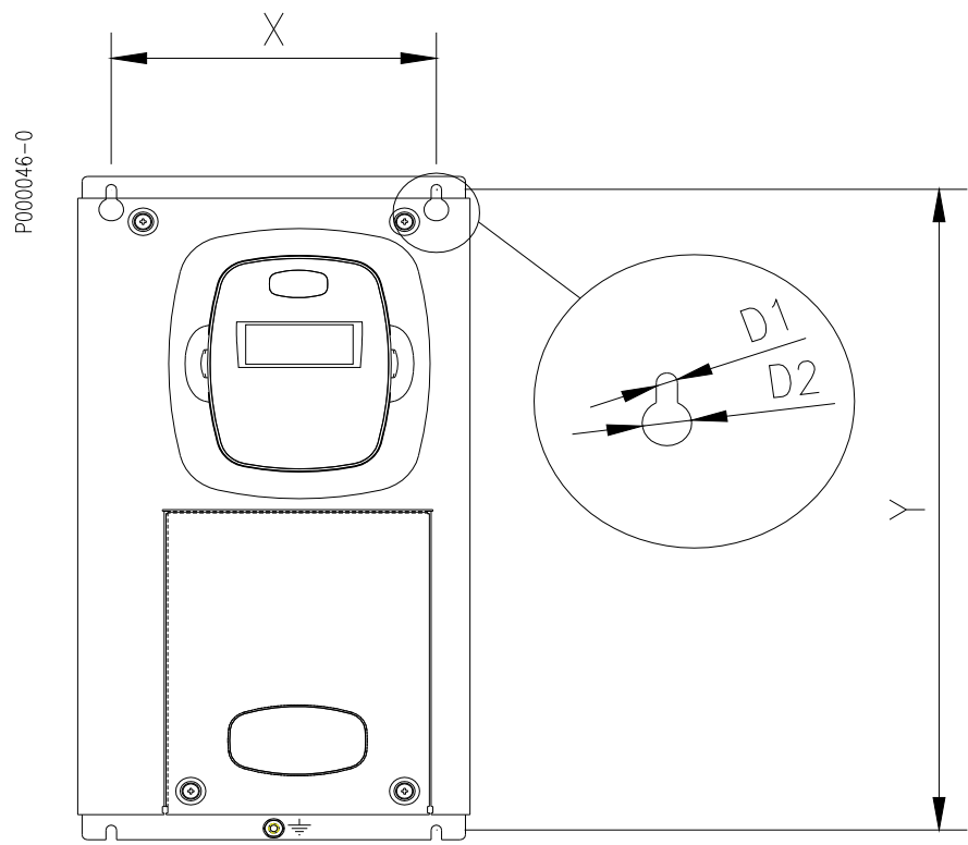
Figure 7: Fixing points for stand-alone control unit.
