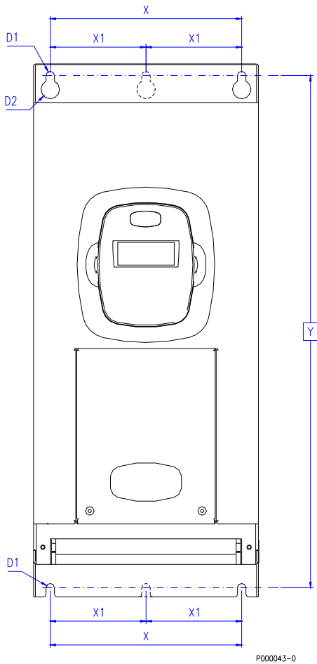
Figure 4: Fixing points for STAND-ALONE models from S05 to S50 included.
