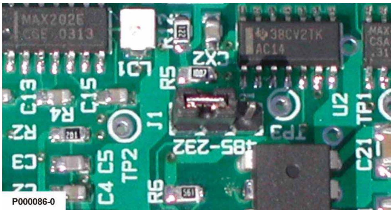
Figure 88: Configuration of the jumpers for RS232/RS485.
