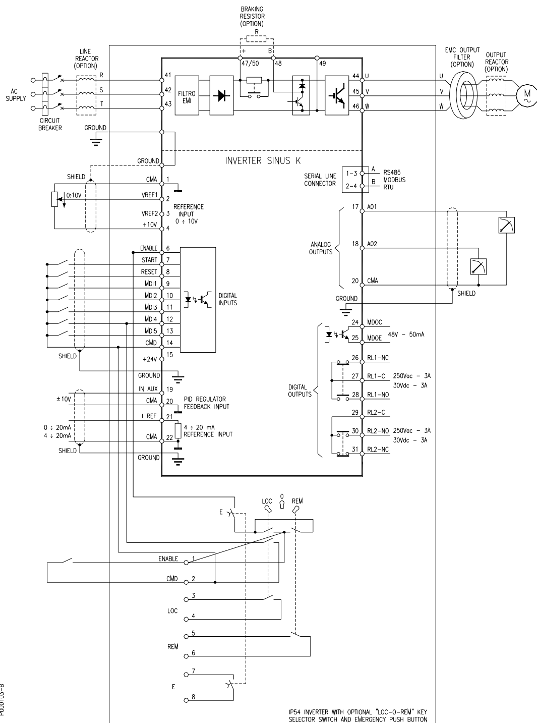
Figure 90: Wiring inverters with optional “LOC-0-REM” key selector switch and emergency push-button.
