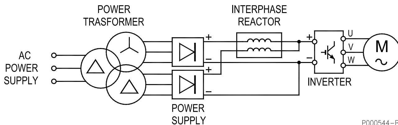
Figure 26: Lay-out of a 12-phase connection.
