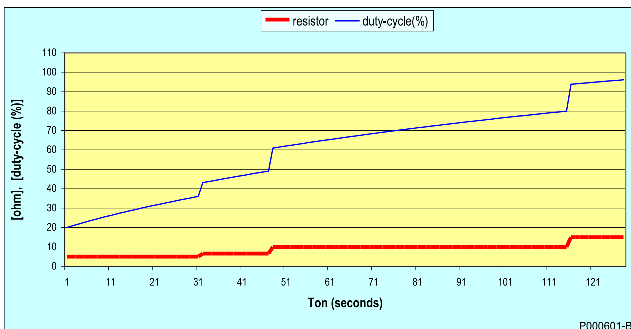
Figure 61: Max. allowable duty-cycle (depending on T_{on} ) for the connected braking resistor.
