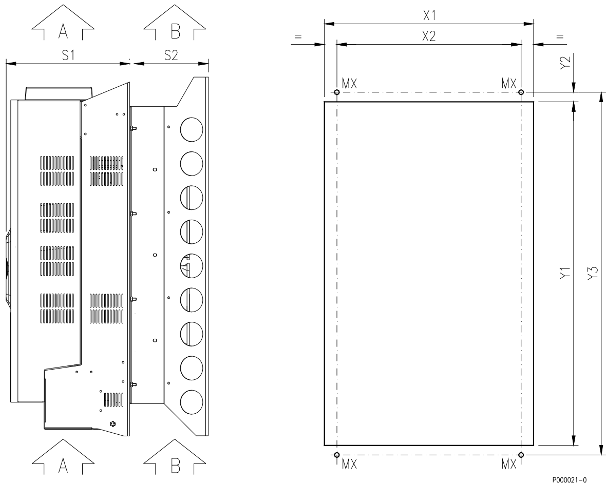
Figure 17: Through-panel assembly and fixing points for SINUS K S15, S20, S30.
