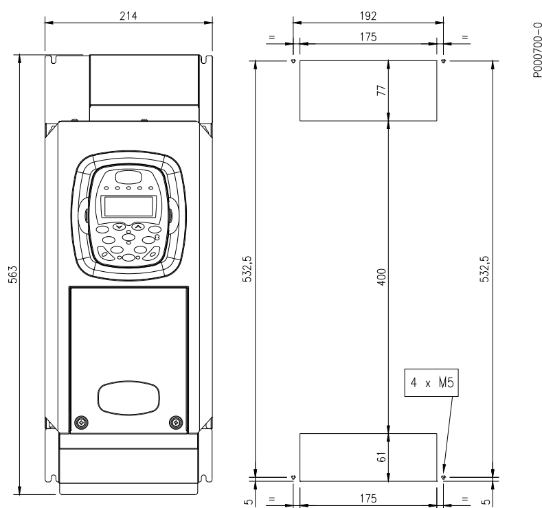
Figure 16: Piercing template for the through-panel assembly for SINUS K S12.
