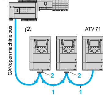
Optimized solution for daisy chain connection to the CANopen machine bus
