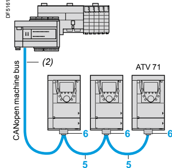
Example of CANopen diagram with daisy chain tap
