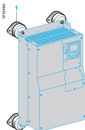
ATV 71H...Y drive mounted on DNV kit VW3 A9 64
