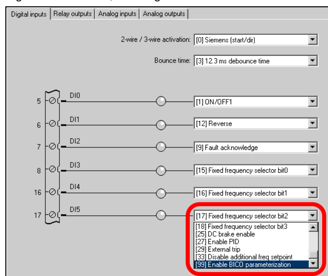
Figure 3-1: CU240E, enabling of BICO interconnection of the DIs
