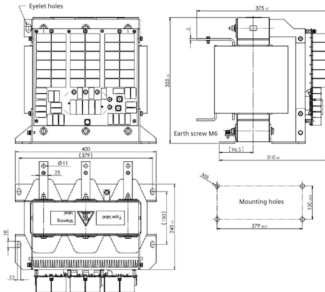
Figure 8-12 Dimensions for JTA:TEF1203-0LB
