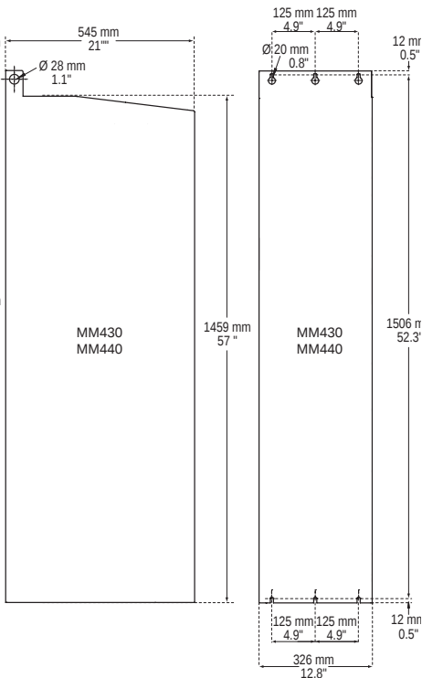
Frame Size GX
