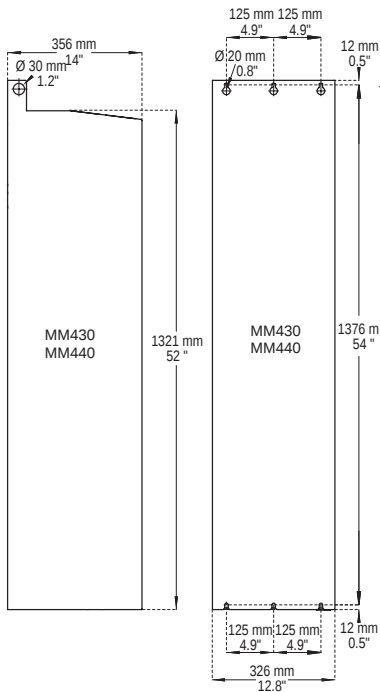
Frame Size FX
