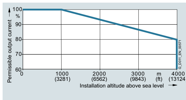
Permissible output current as a function of installation altitude for SINAMICS G120X for low overload (LO)
