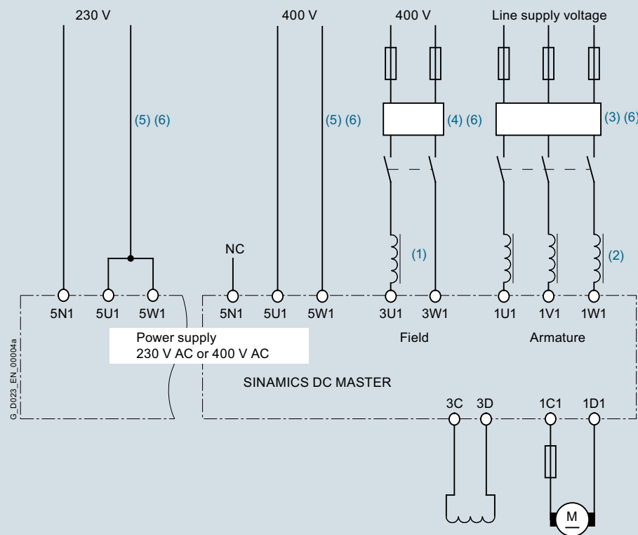
Arrangement of reactors and radio interference suppression filters
