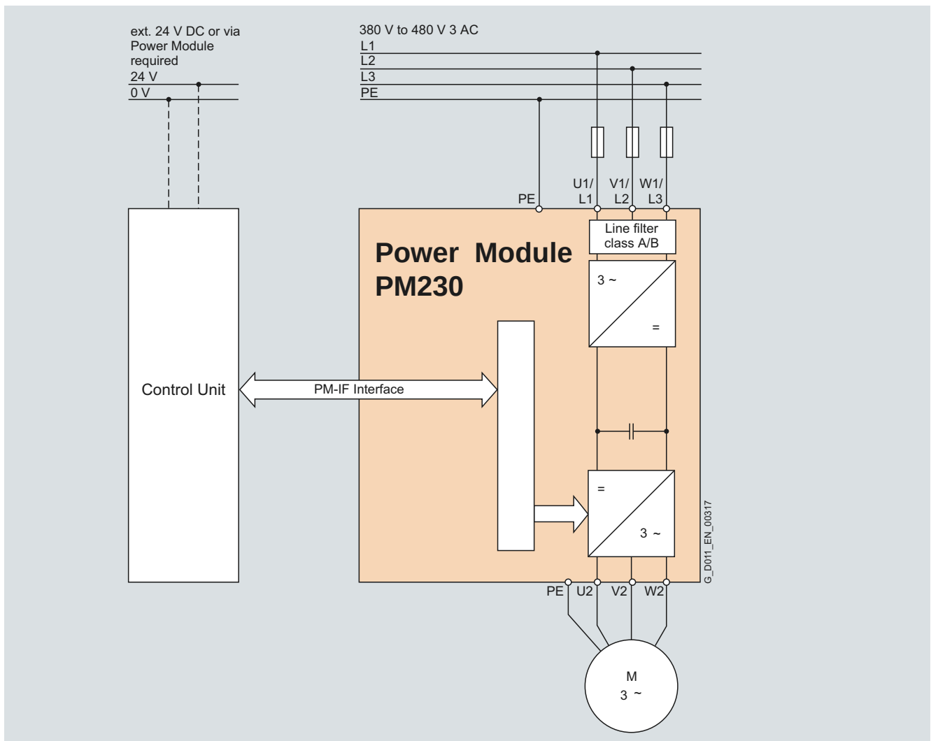
Connection diagram for PM230 Power Module with integrated line filter class A or B
