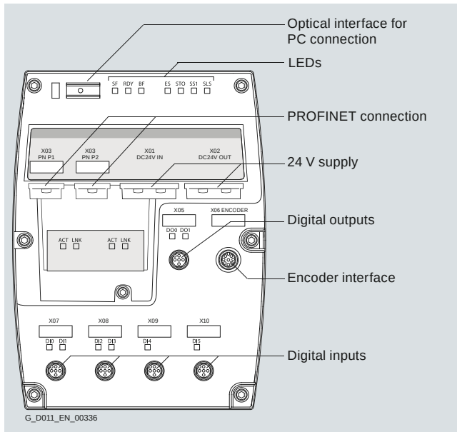
CU240D PN-F PP Control Unit
