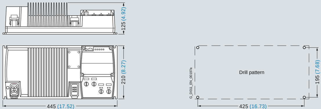
SINAMICS G110D, frame size FSA, with integrated line filter class A
