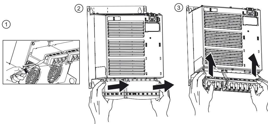
Figure 4-2 Access to power and motor terminals on FSD, FSE and FSF
