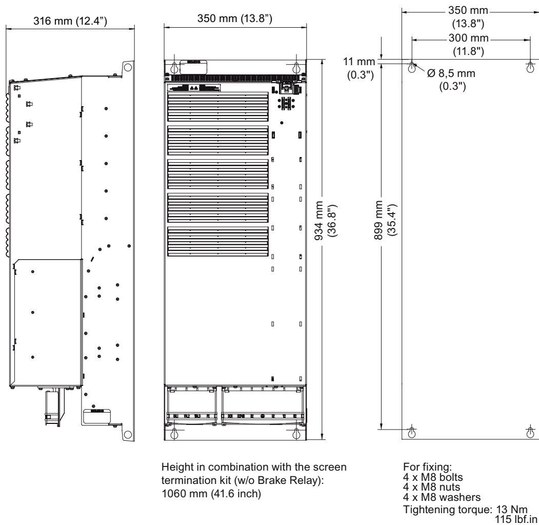
Figure 3-8 Dimensions and drill pattern, FSF filtered (HO 45 kW ... 75 kW)
