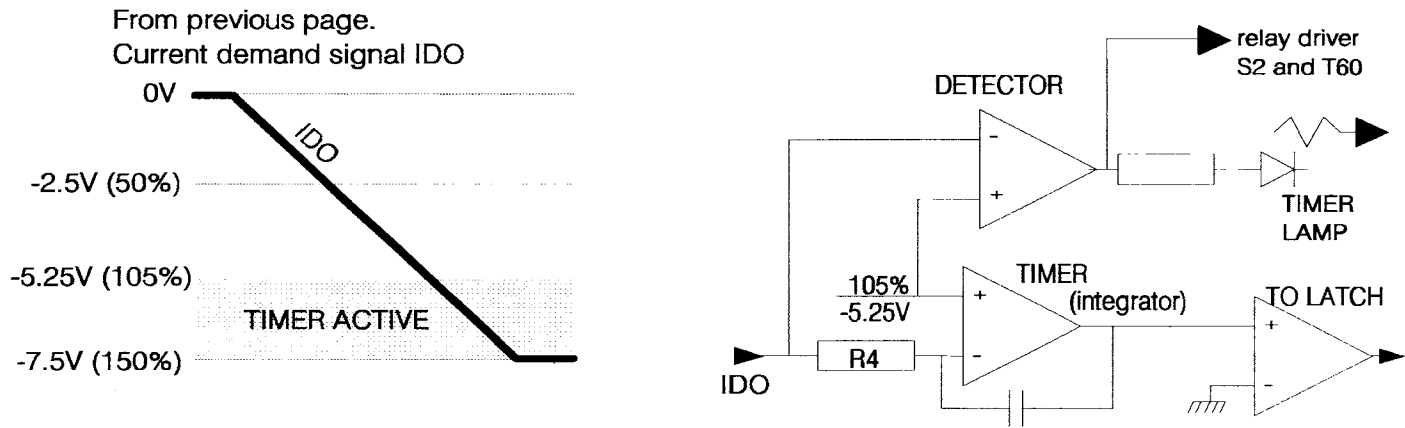
SCHEMATIC OF STALL TIMER
