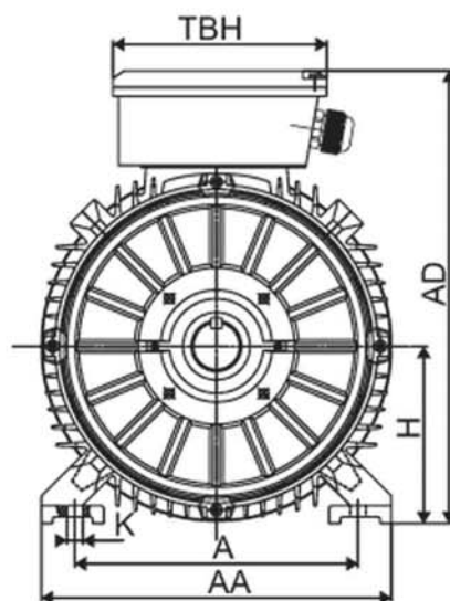
C.I.housing
